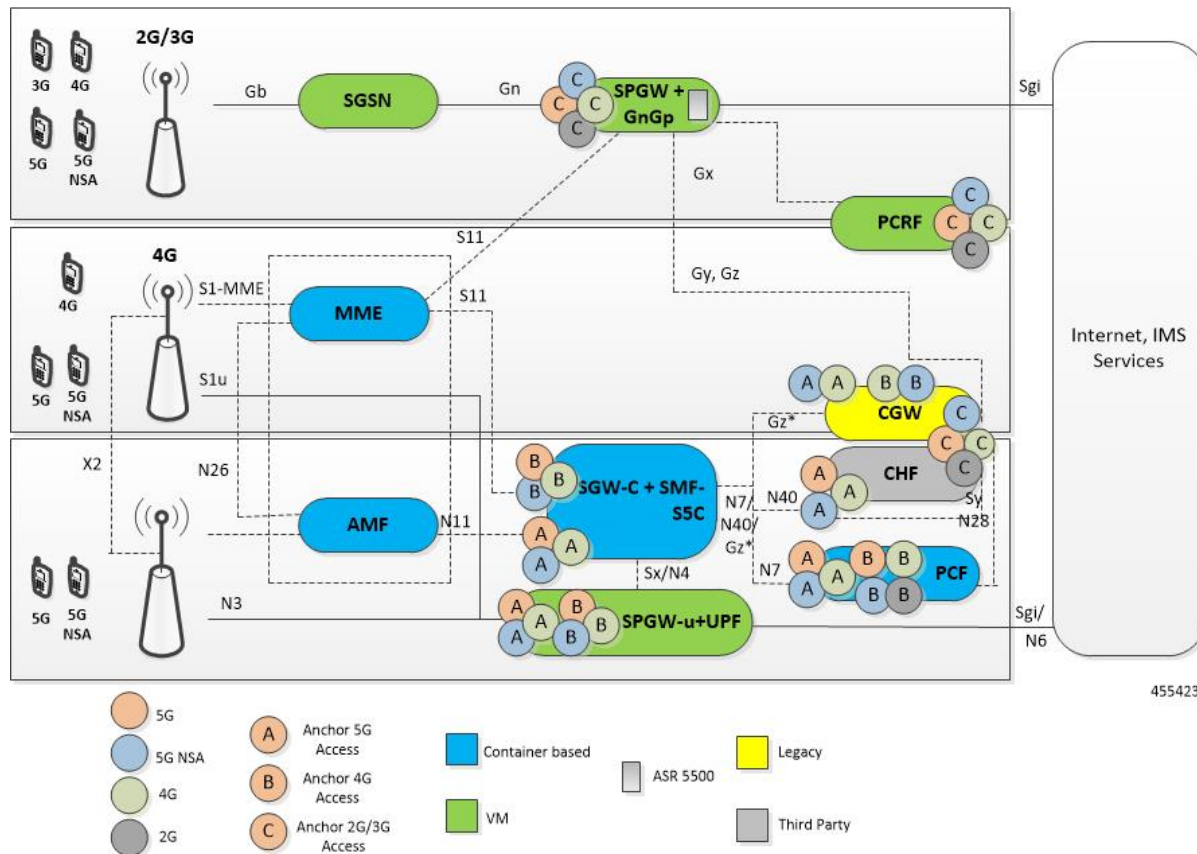
Figure 8: Converged Core Architecture
