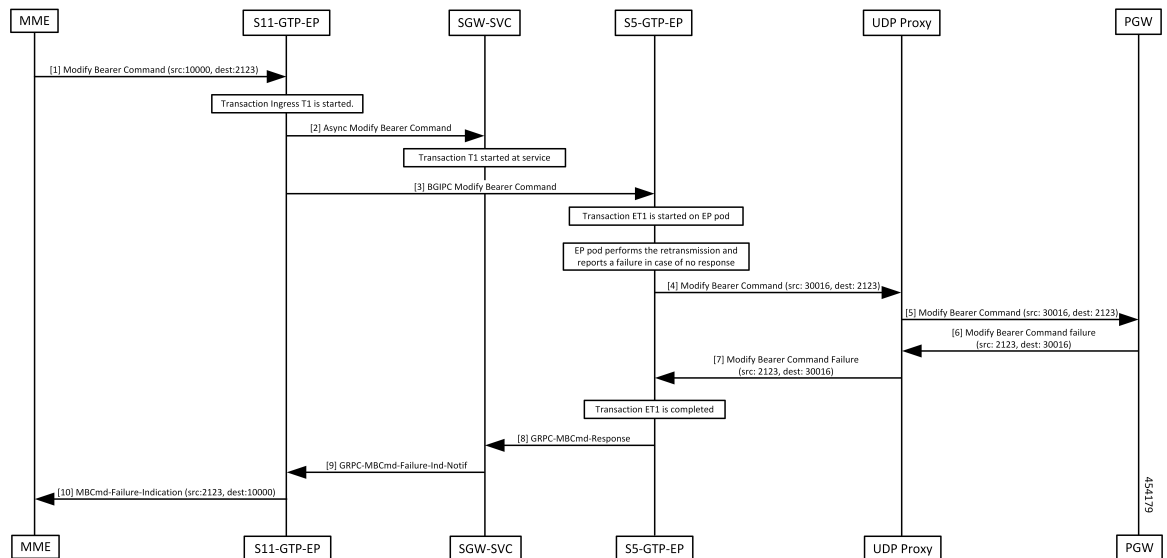
Figure 88: MBC Failure Handling Call Flow
