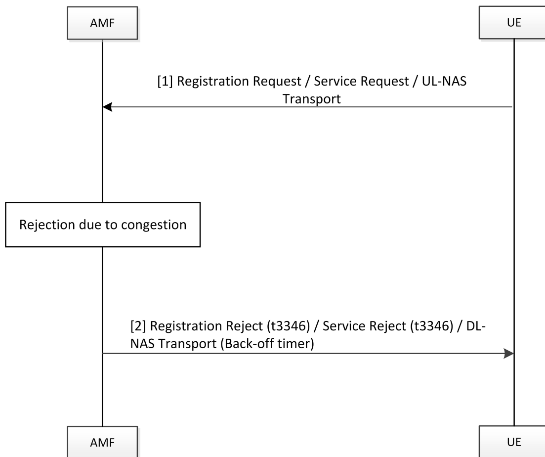
Figure 69: T3346 Timer Call Flow
