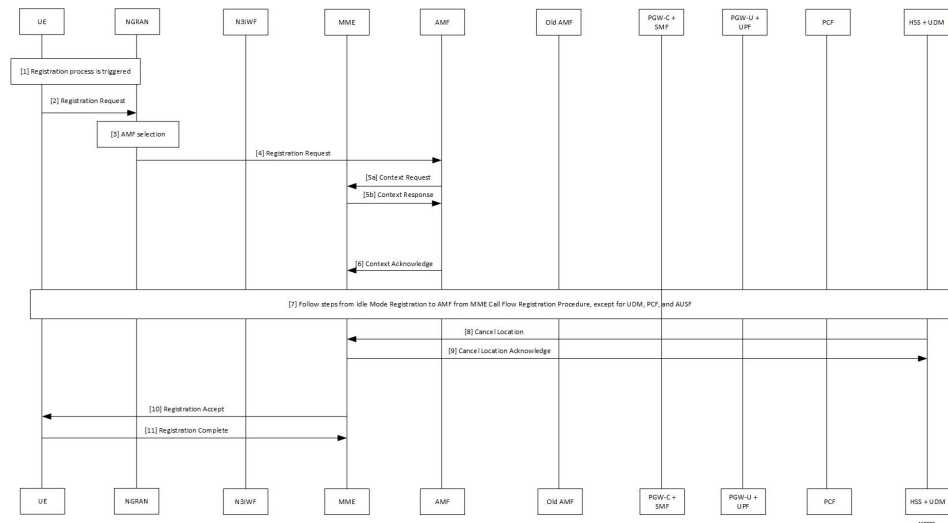
Figure 91: AMF-MME (N26_Idle) Scenario Scenario Call Flow
