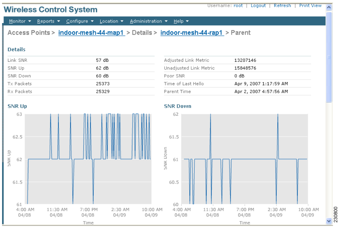
Figure 6-32 Mesh SNR Graphs Page (Top)
