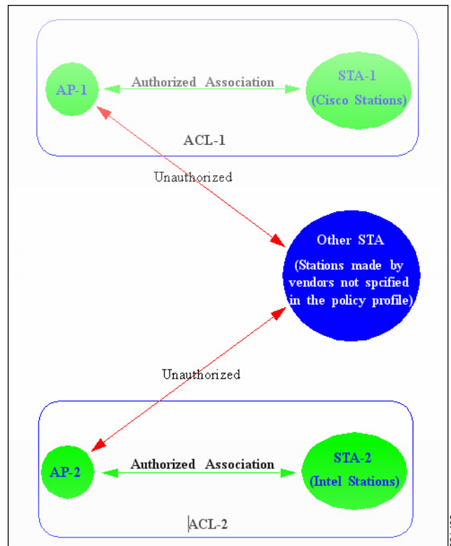
Figure 19-33 Unauthorized Access Point-station Associations Filtered by Station Vendors
