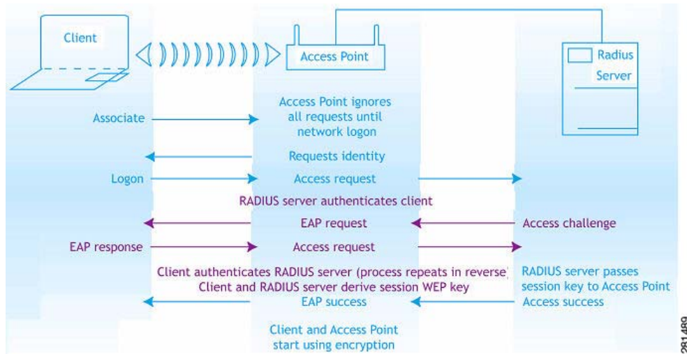
Figure 19-8 802.1x User Authentication Process
