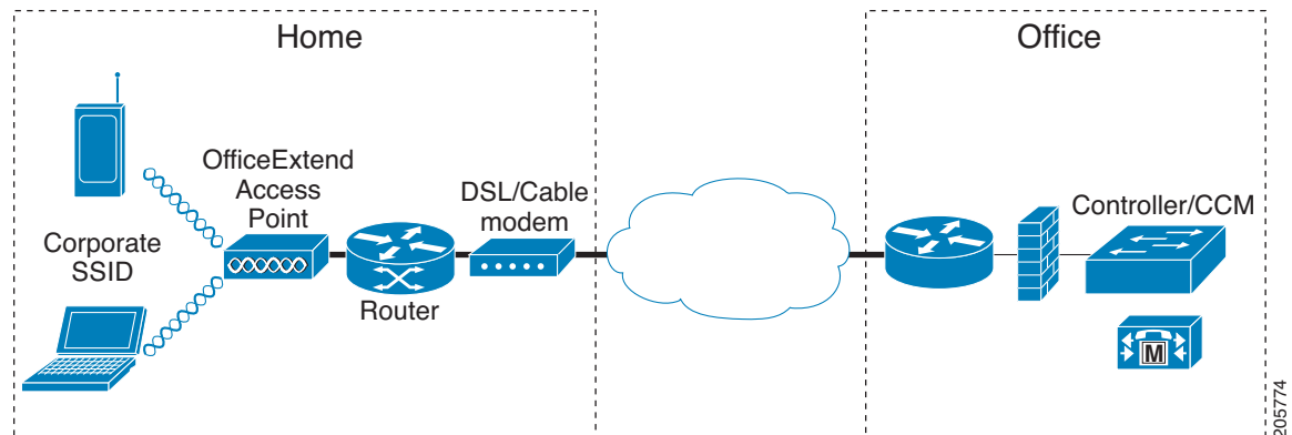
Figure 9-21 Typical OfficeExtend Access Point Setup
