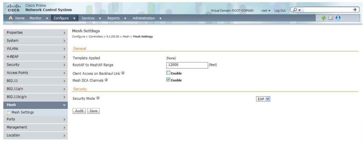
Figure 9-6 Mesh Settings Page
