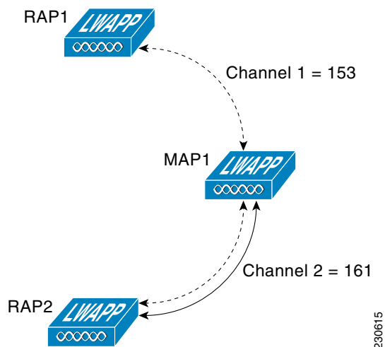
Figure 9-4 Mesh Access Point (MAP1) Selects a Parent
