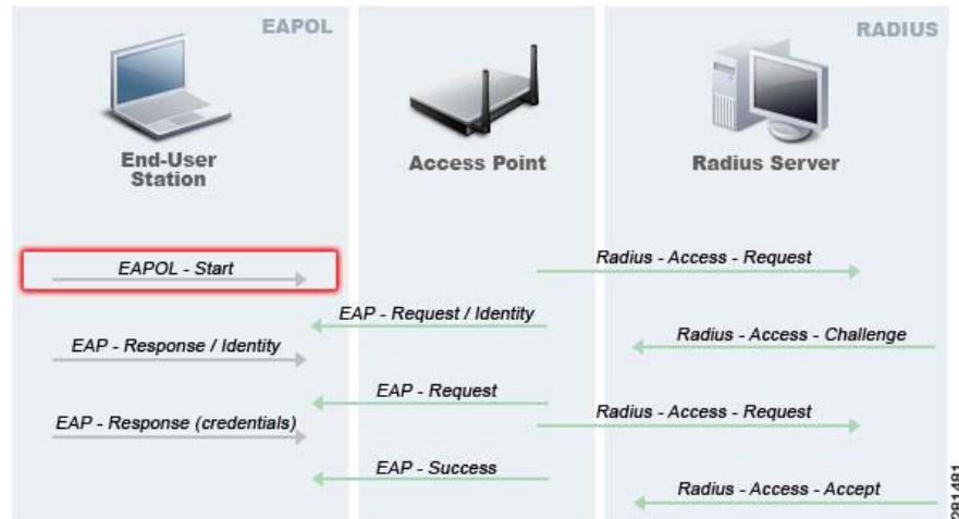
Figure 19-3 EAPOL-Start Protocol and EAPOL-Start Attack
