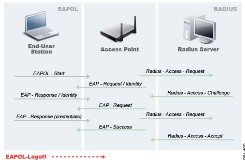
Figure 19-14 EAPOL-Logoff Protocol and EAPOL-Logoff Attack
