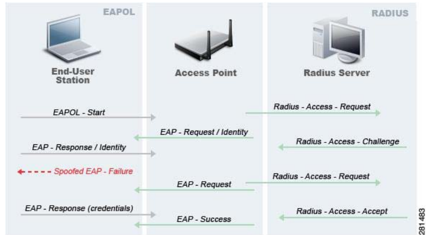
Figure 19-16 EAP-Failure Protocol and Premature EAP-Failure Attack
