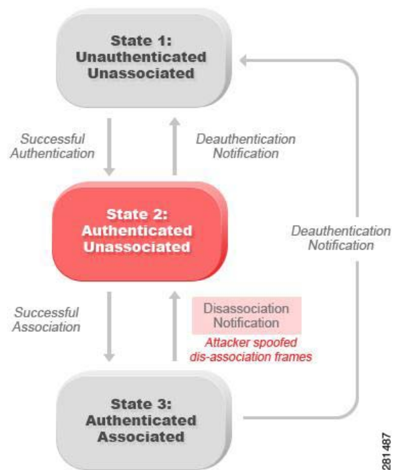
Figure 19-12 Client State Machine and Disassociation Broadcast Attack
