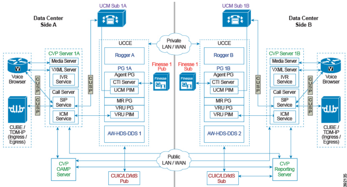
Figure 57: Detailed 2000 Agent Reference Design
