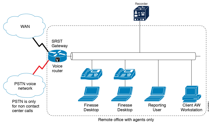
Figure 51: Remote Office with Agents—Physical View
