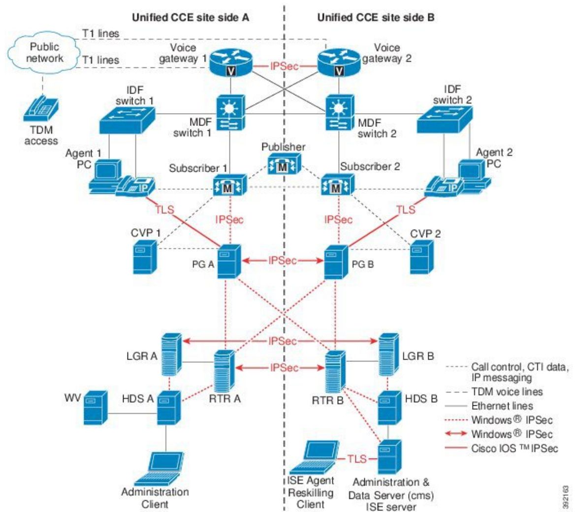
Figure 101: IPsec Deployment Example
