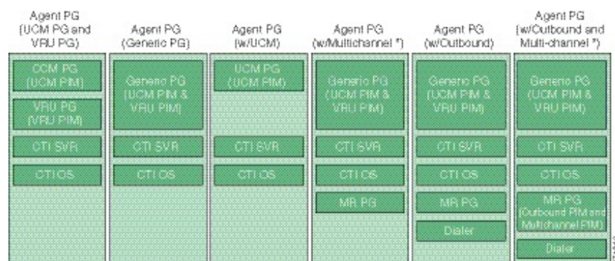
Figure 141: Agent PG Configuration Options with CTI OS
