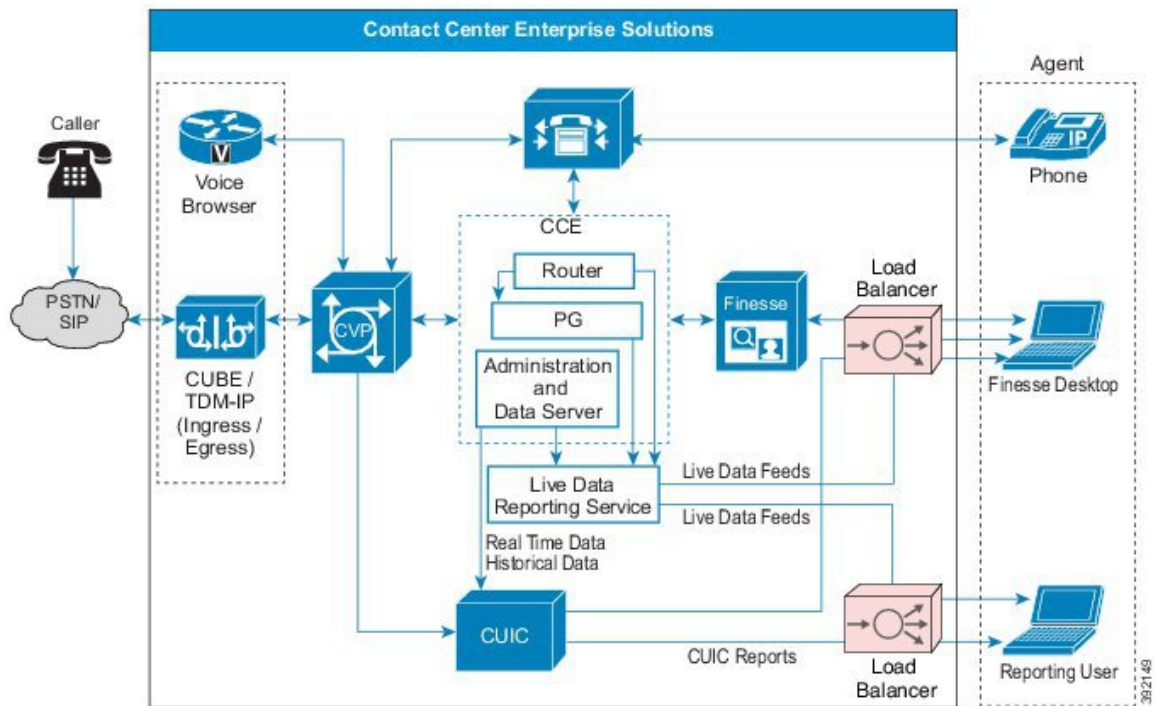
Figure 70: Unified Intelligence Center Deployment with Unified CCE for Historical and Real-Time Reporting
