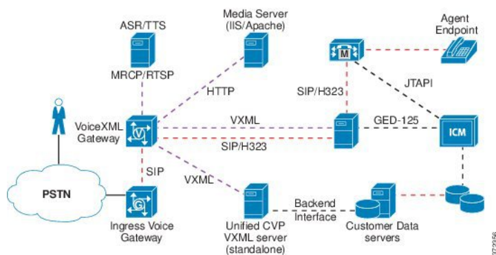
Figure 136: VRU-Only Functional Deployment
