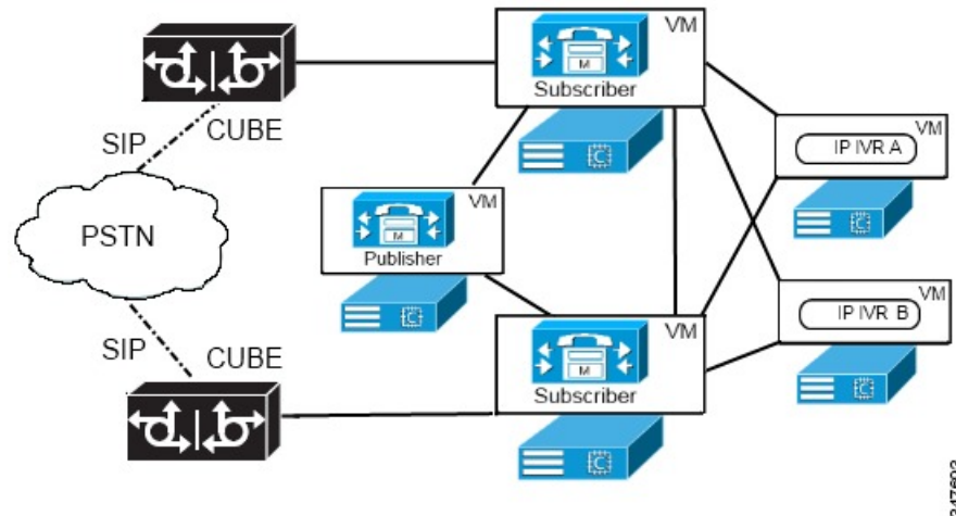
Figure 139: IP IVR High Availability Deployment
