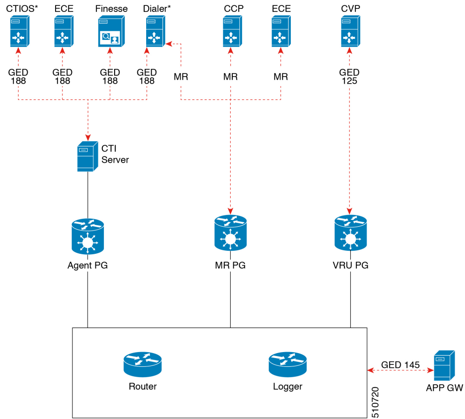
Figure 102: Secured Connection Example
