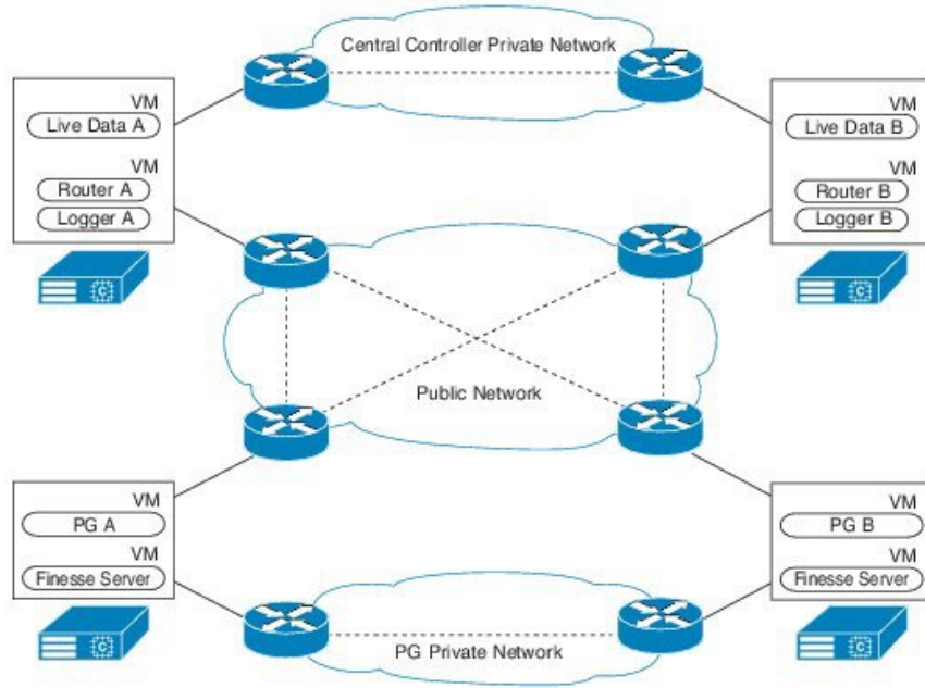
Figure 61: High Availability Design for Central Controller
