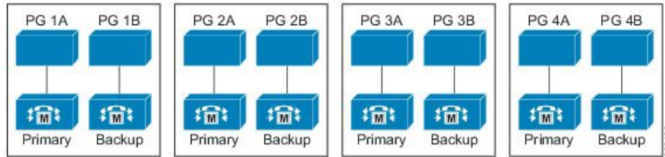
Figure 63: Deploy Agent PG for Each Pair of Subscribers in a Cluster
