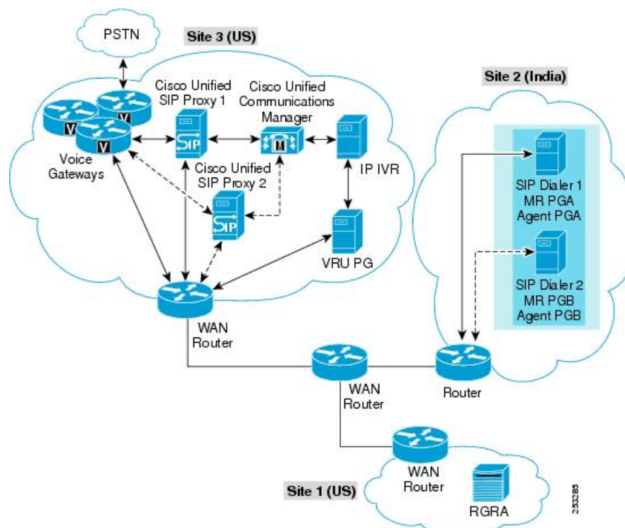
Figure 140: Distributed Deployment Example for Transfer-to-VRU Campaign with Unified IP IVR
