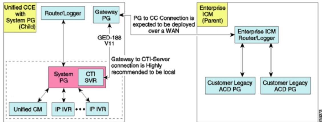
Figure 126: Connection Between Gateway PG and System PG
