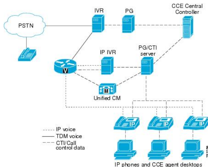
Figure 133: Traditional VRU Integration Using VRU Double Trunking
