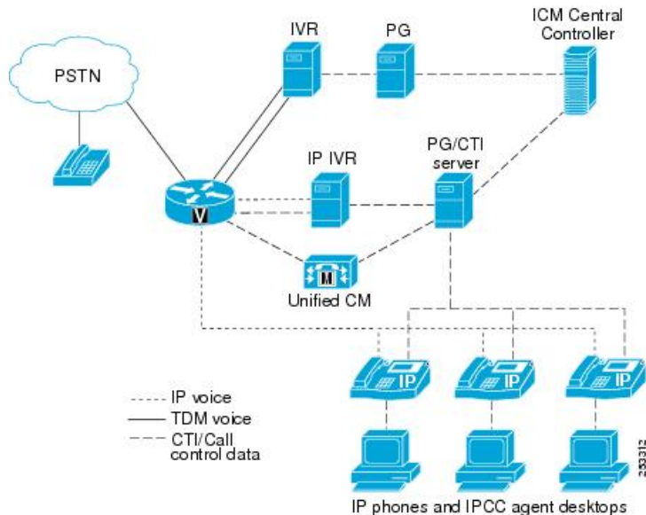
Figure 134: Unified Communications Manager Transfer and VRU Double Trunking
