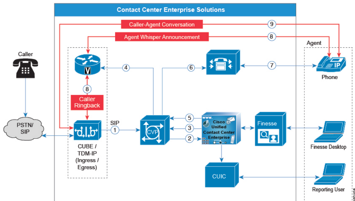
Figure 121: Whisper Announcement Call Flow
