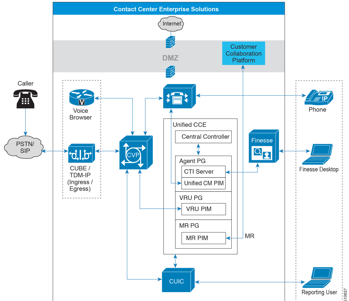
Figure 30: Customer Collaboration Platform in Contact Center Enterprise Solutions
