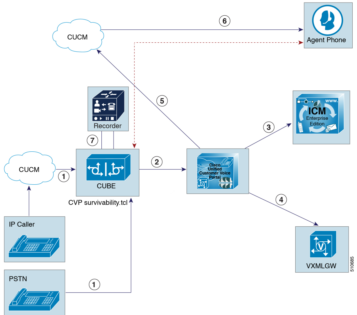
Figure 78: Network-Based Recording Call Flow
