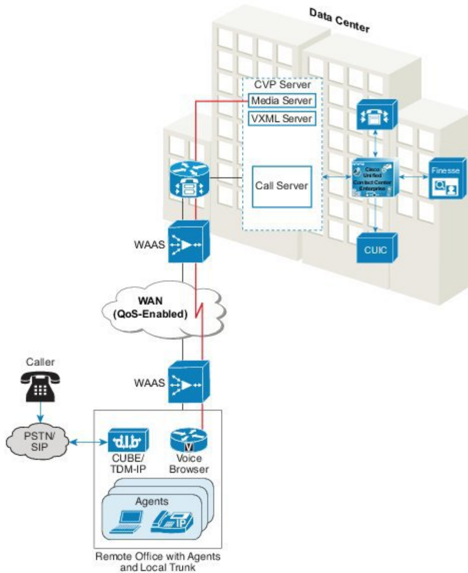
Figure 60: Distributed Deployment Over WAN
