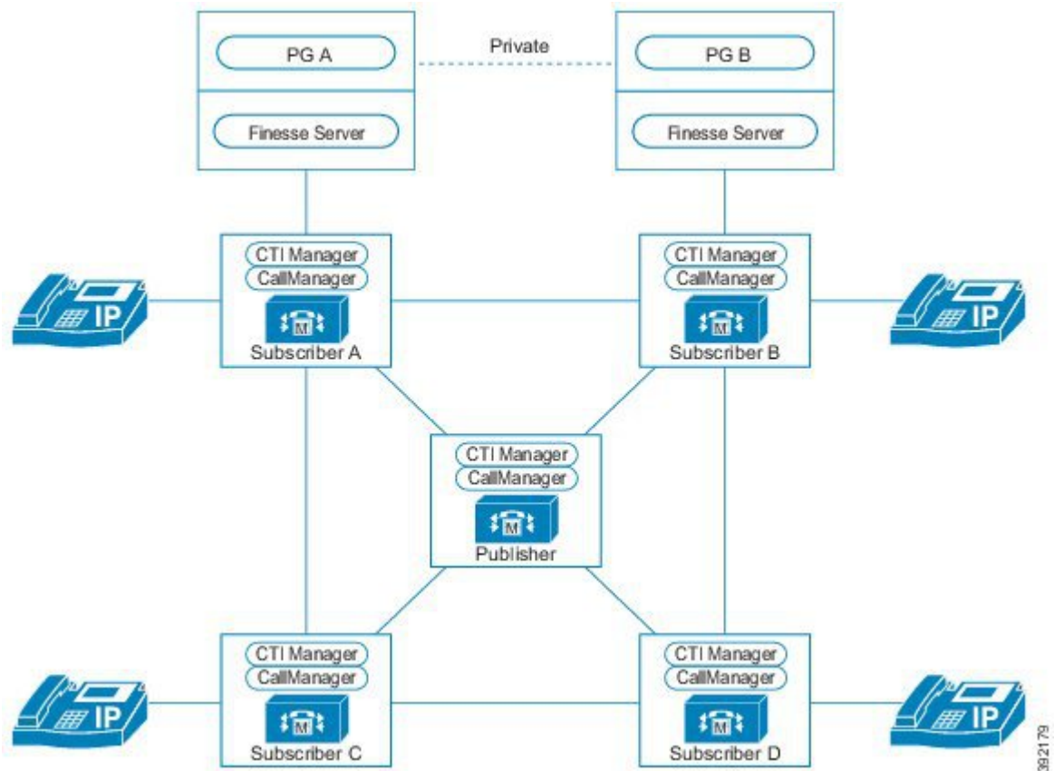
Figure 62: High Availability Design for Unified CM Cluster
