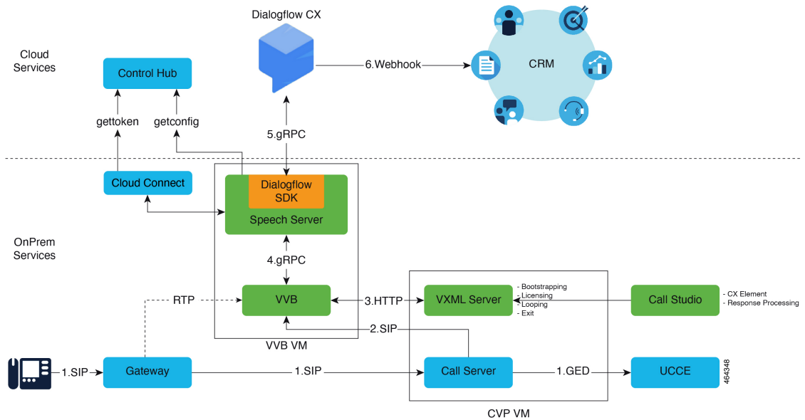
Figure 108: Architecture
