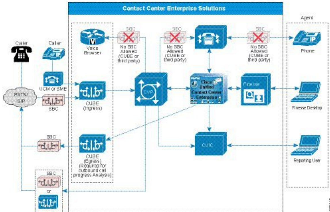
Figure 79: SBC Implementation
