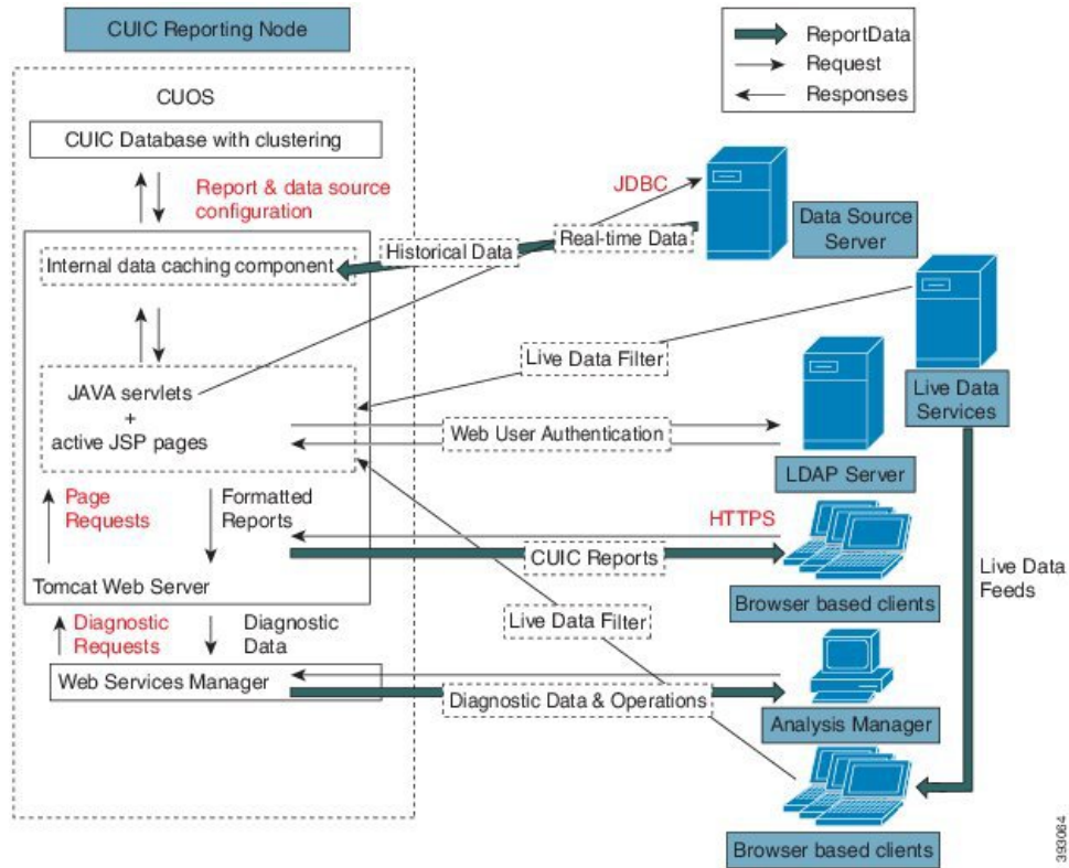
Figure 68: Unified Intelligence Center Architecture
