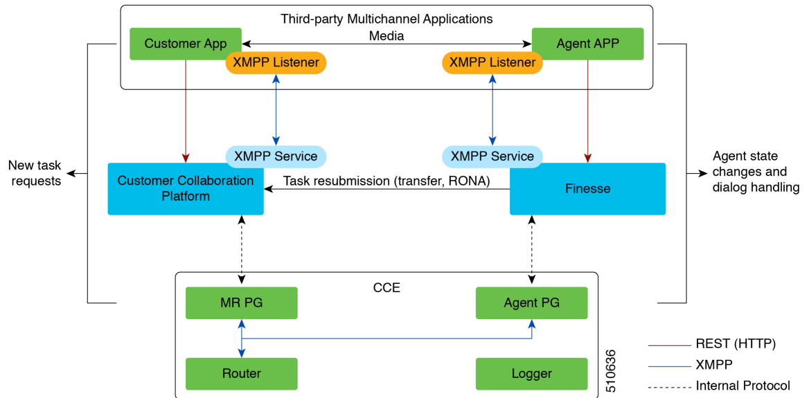
Figure 73: Task Routing for Third-party Multichannel Applications Solution Components
