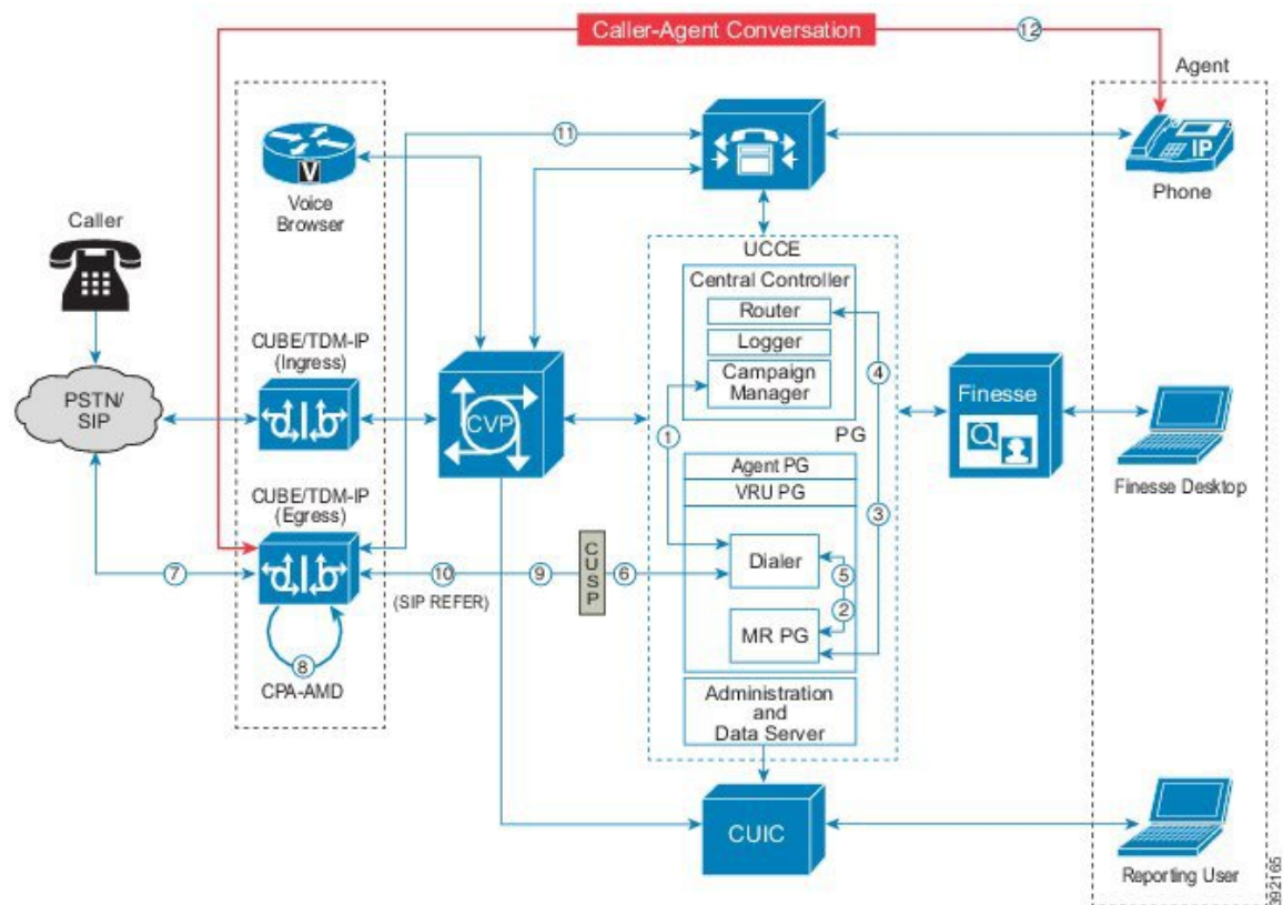
Figure 109: SIP Dialer Agent Campaign Call Flow
