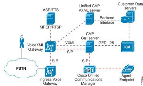
Figure 135: VXML Server (Standalone) Functional Deployment
