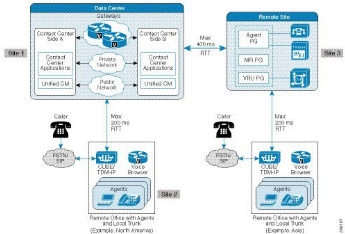
Figure 115: Distributed Outbound SIP Dialer Deployment for Transfer to a VRU Campaign with CVP
