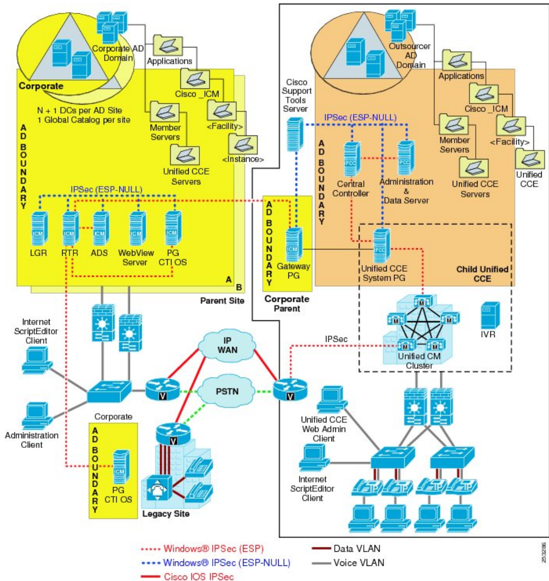
Figure 127: Active Directory and Firewall Deployment
