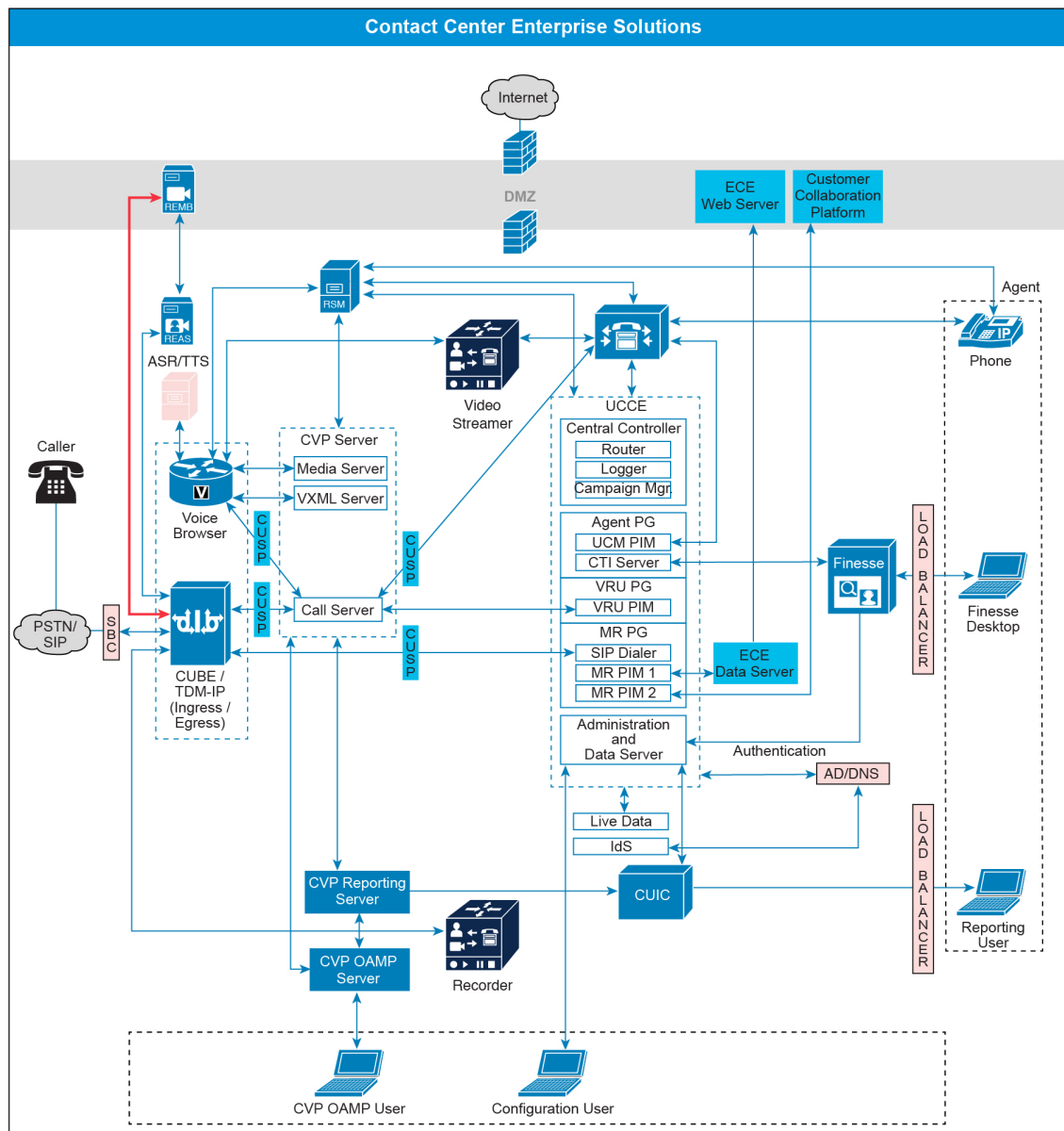
Figure 37: Logical Component Connectivity
