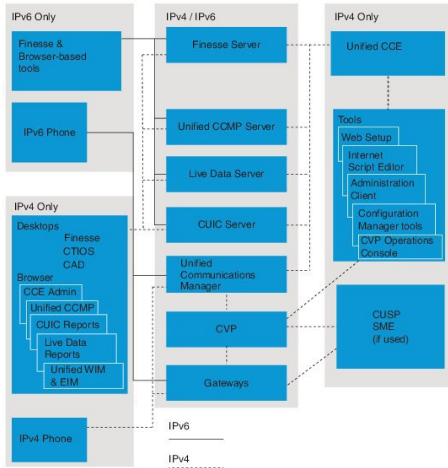
Figure 124: Unified CCE Deployment with Both IPv4 and IPv6 Agents
