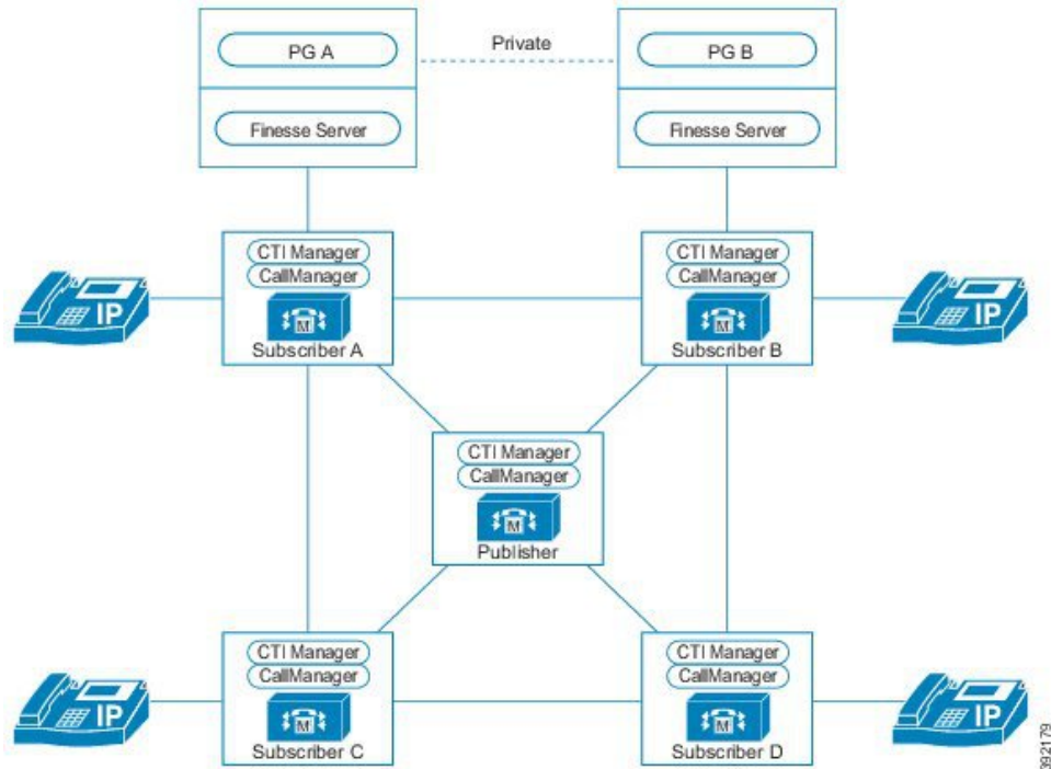
Figure 66: Single Agent PG Pair for Entire Unified CM Cluster
