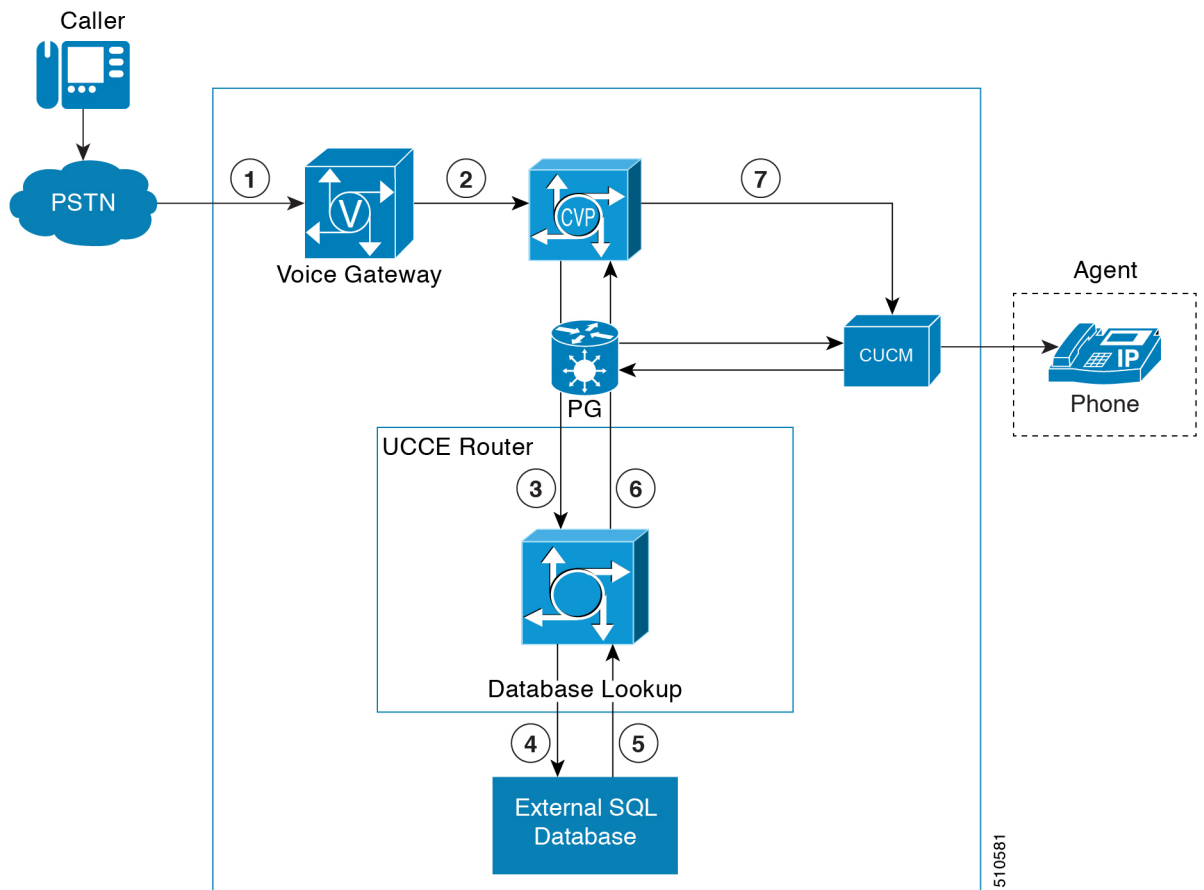
Figure 117: Database Lookup Call Flows
