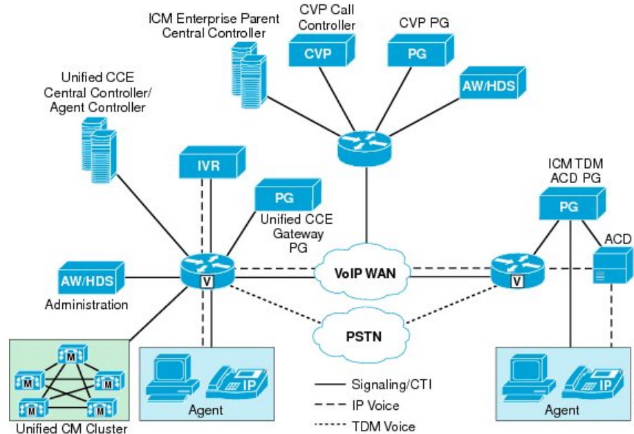
Figure 131: Parent/Child Integration of Traditional ACD with Unified CCE
