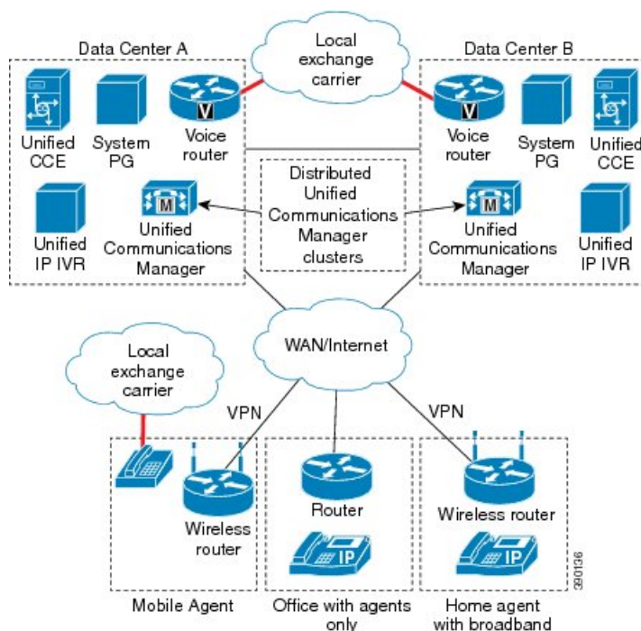
Figure 129: Geographically Redundant Child Sites with Clustering over WAN (Using Unified IP IVR)
