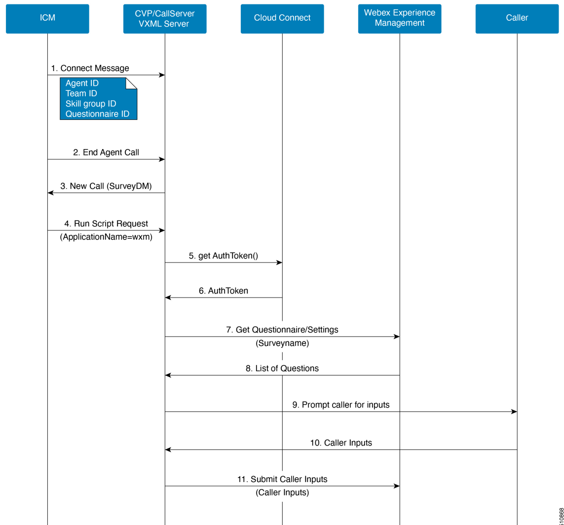
Figure 119: Voice Survey Call Flow
