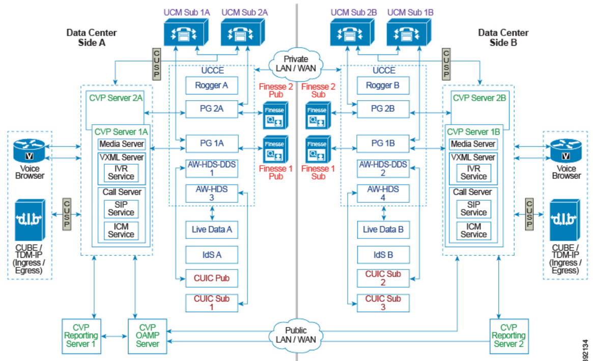
Figure 58: Detailed 4000 Agent Reference Design
