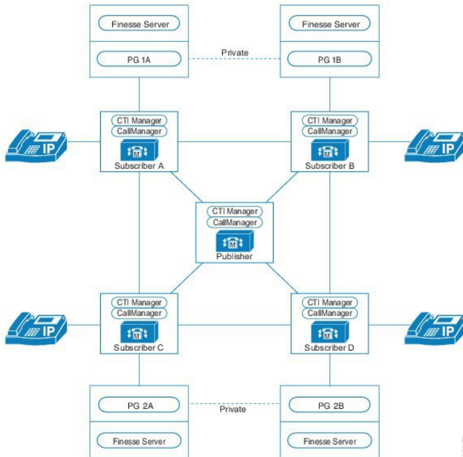
Figure 64: 2 Agent PG Pairs for Unified CM Cluster
