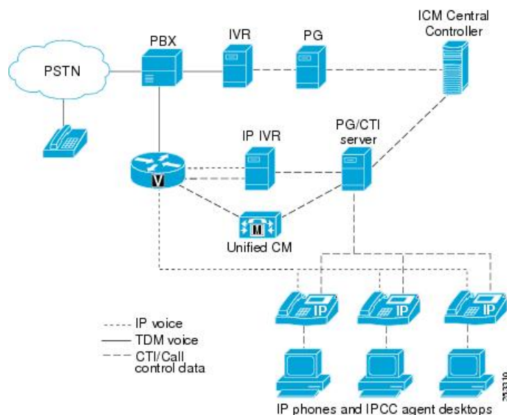
Figure 132: Traditional VRU Integration Using PBX Transfer
