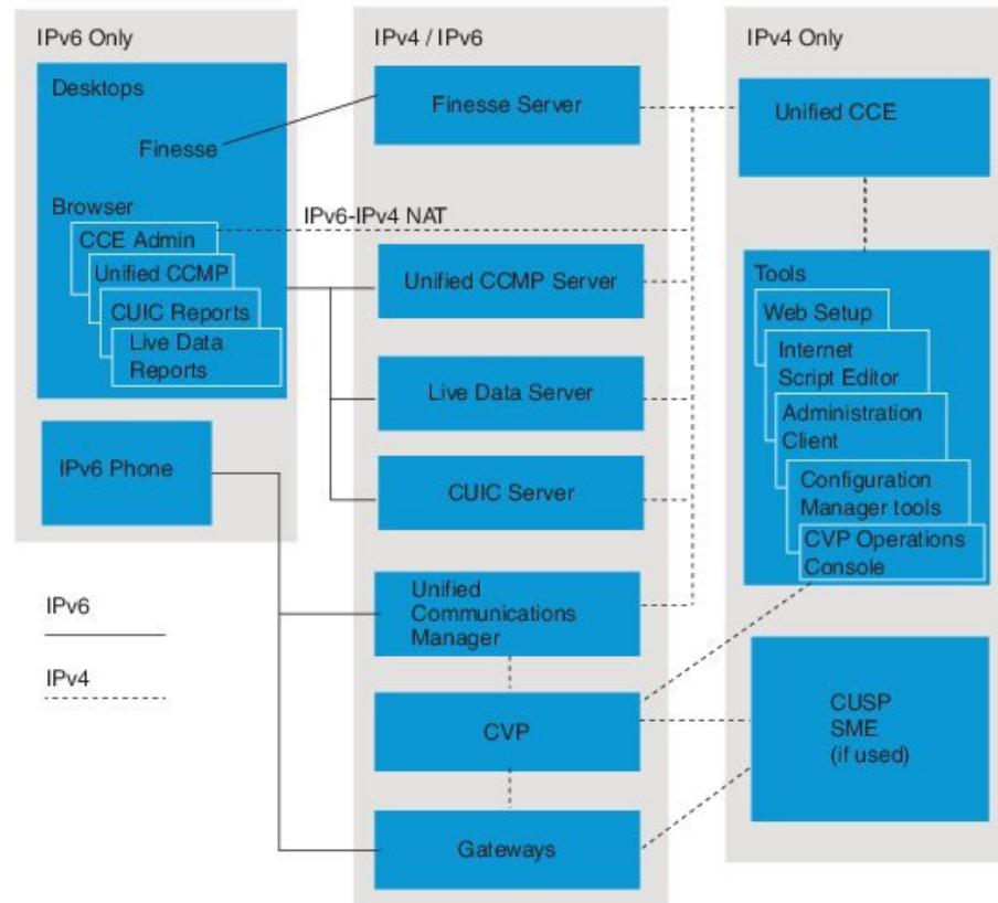
Figure 123: Unified CCE Deployment with Only IPv6 Agents
