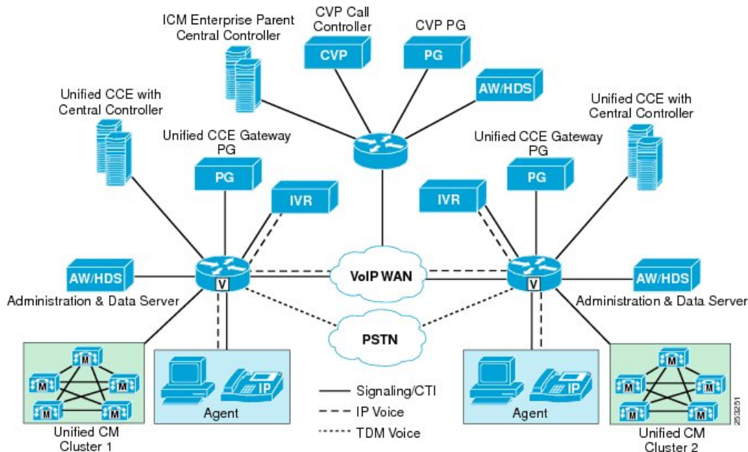
Figure 128: Multisite Deployment with Distributed Call Processing and Parent/Child
