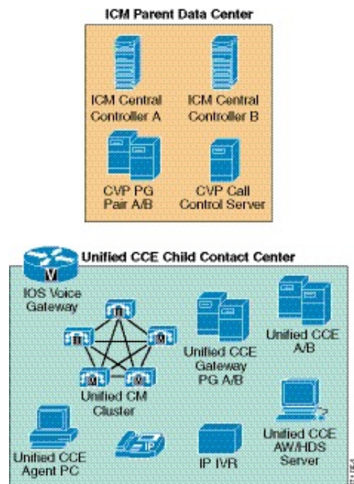
Figure 130: Parent/Child Deployment
