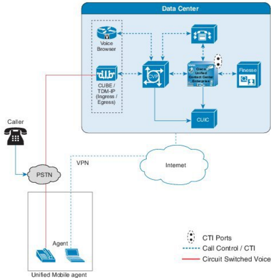
Figure 118: Cisco Unified Mobile Agent Architecture
