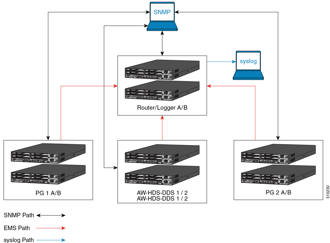
Figure 10: ICM/CCE Event Message Flow
