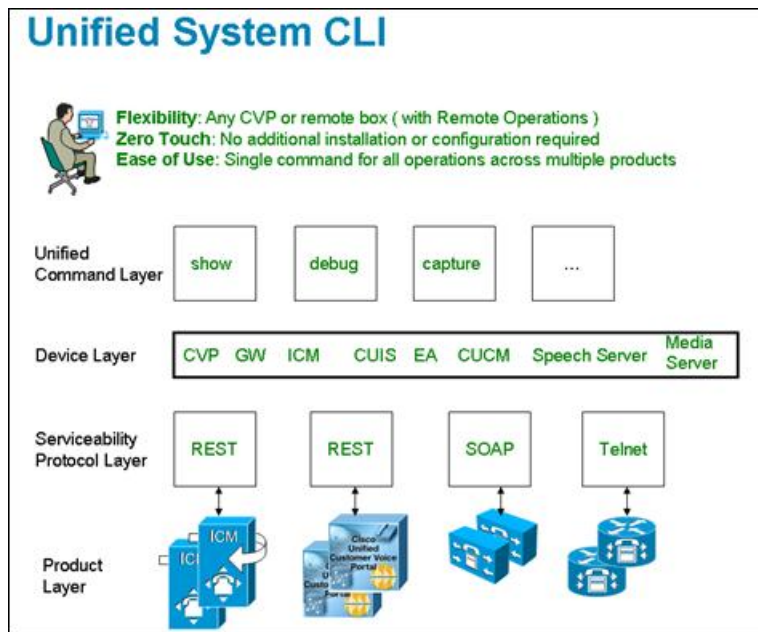
Figure 28: Unified CLI Architecture
