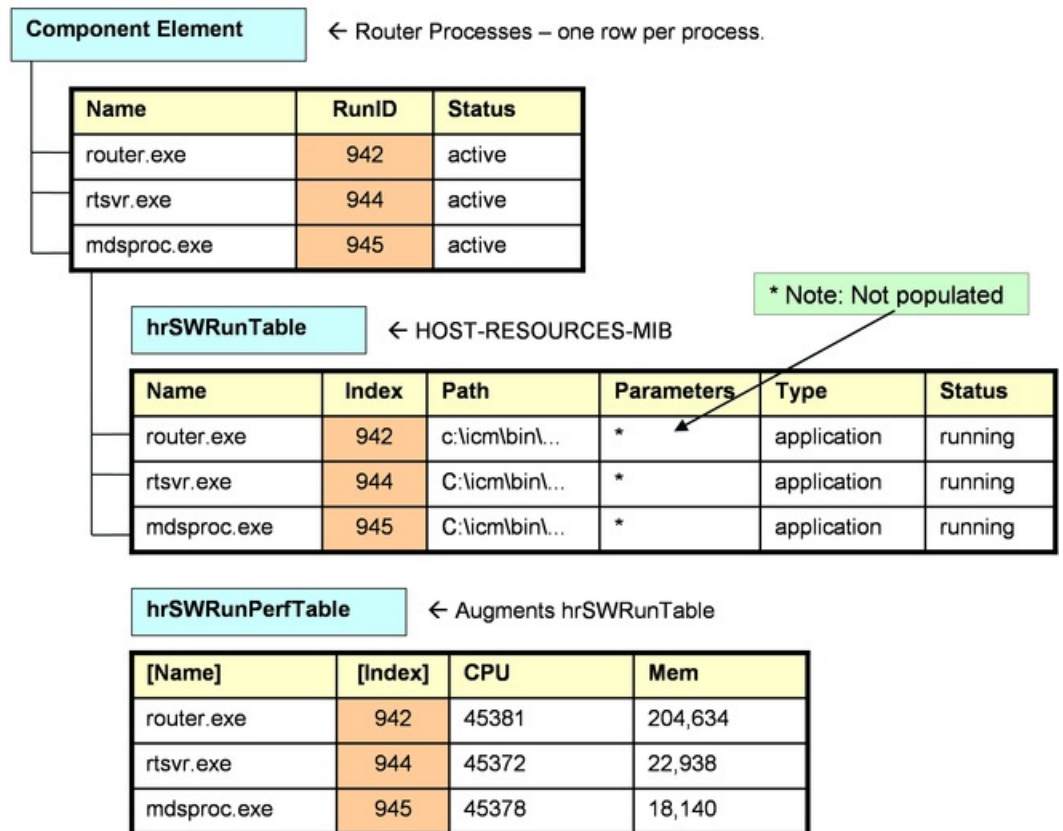
Figure 13: Mapping CCCA MIB Objects to Host MIB Objects
