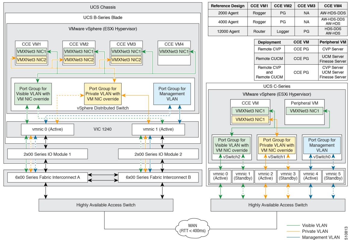
Figure 94: Network Requirements for Cisco UCS C-Series Servers
