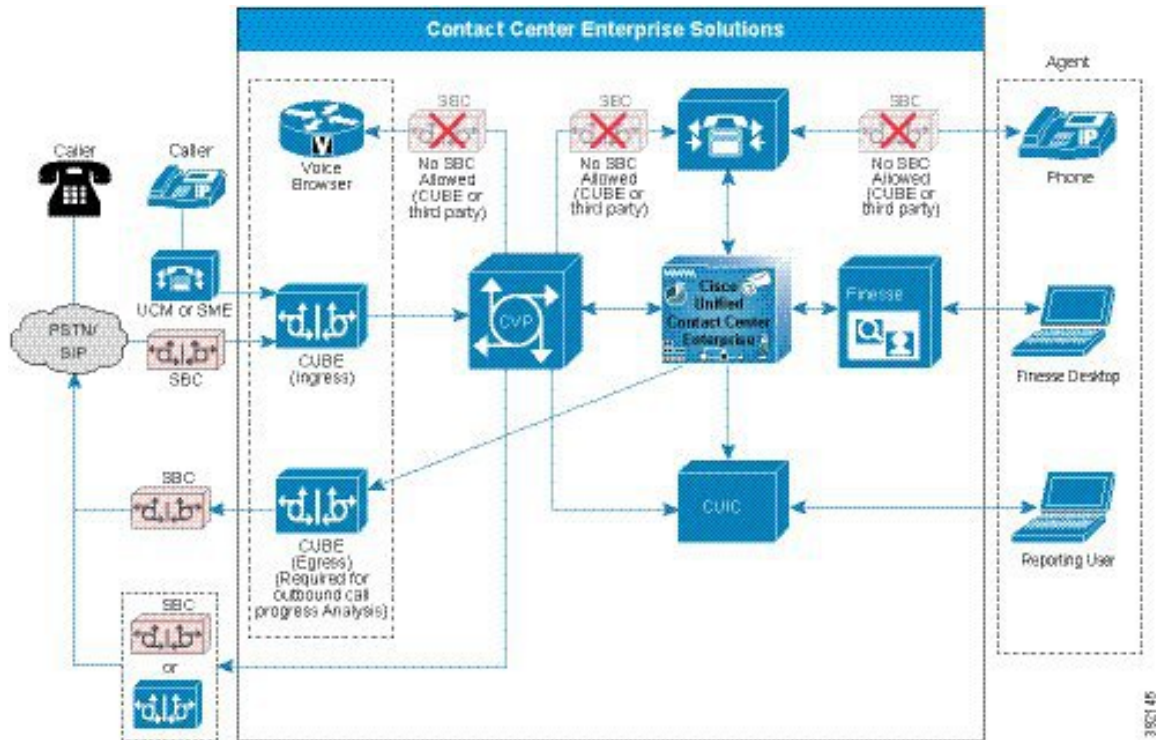
Figure 91: SBC Implementation
