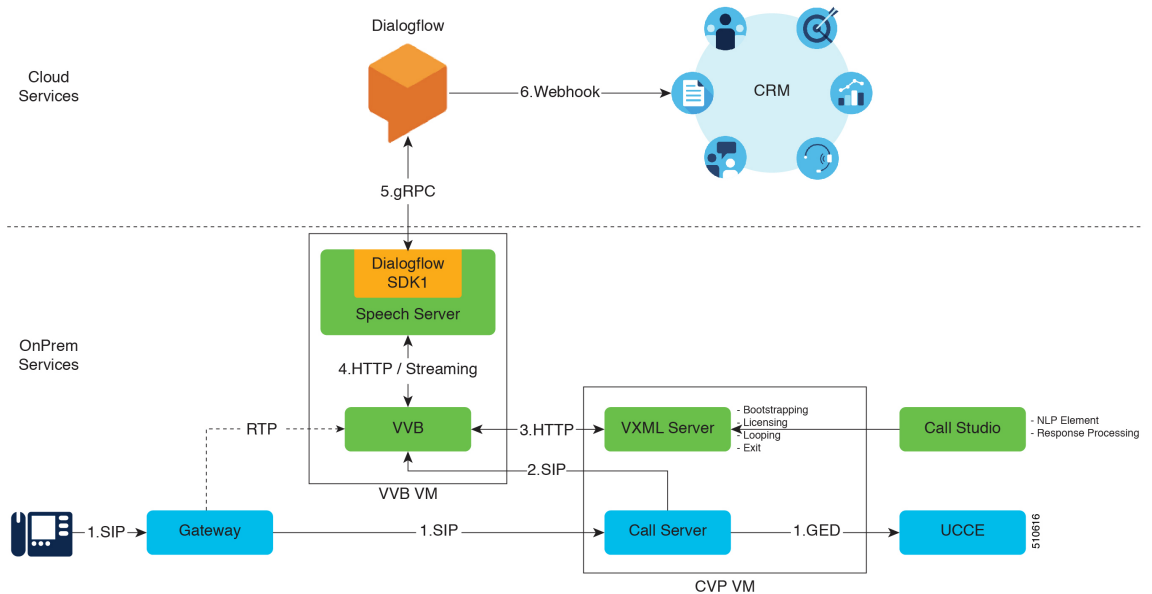
Figure 117: Architecture
