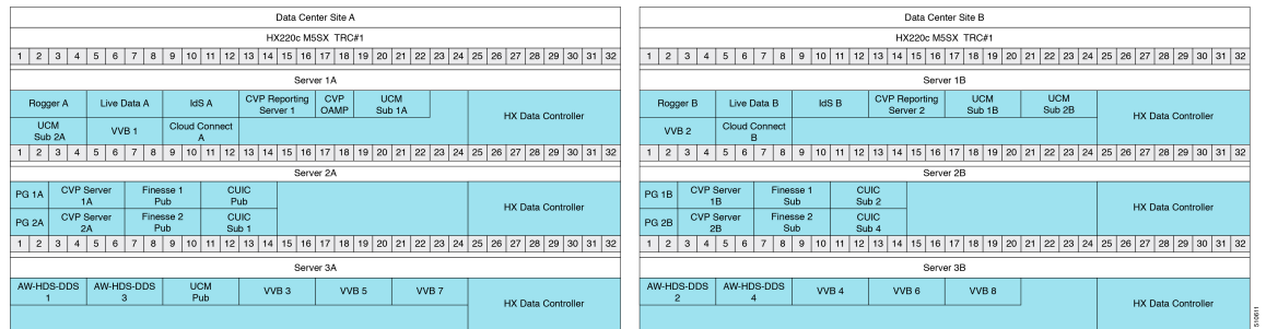
Figure 7: 4000 Agent Reference Design Model
