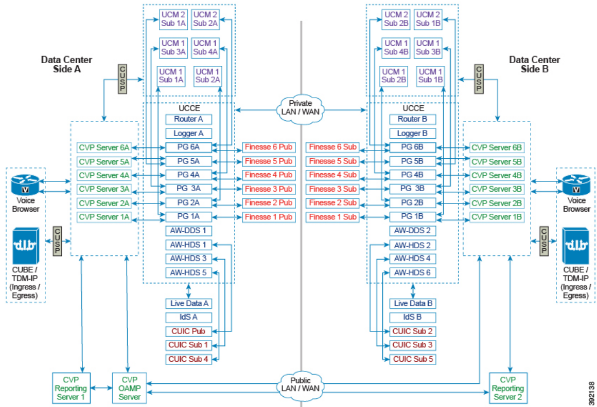
Figure 68: Detailed 12000 Agent Reference Design
