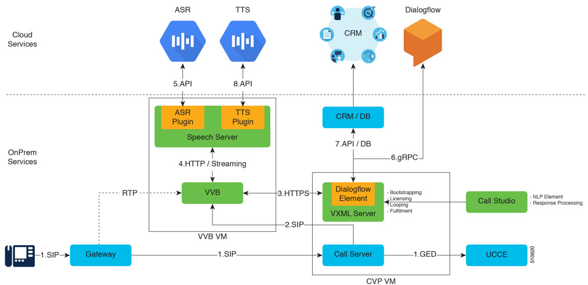
Figure 118: Architecture
