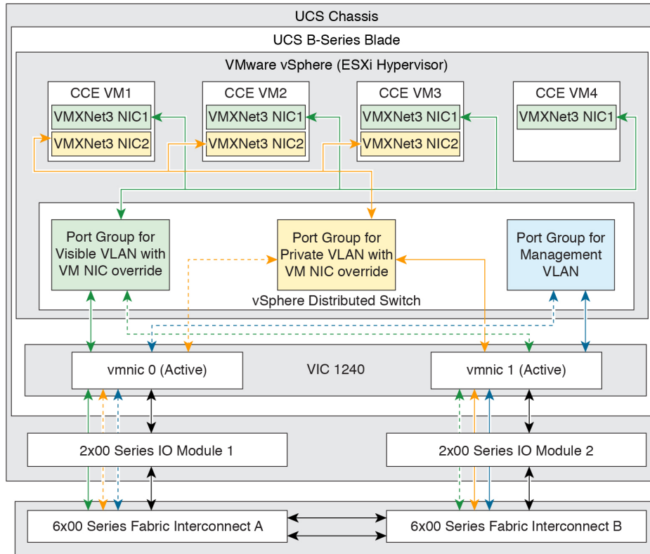
Figure 93: Network Requirements for Cisco UCS B-Series Servers
