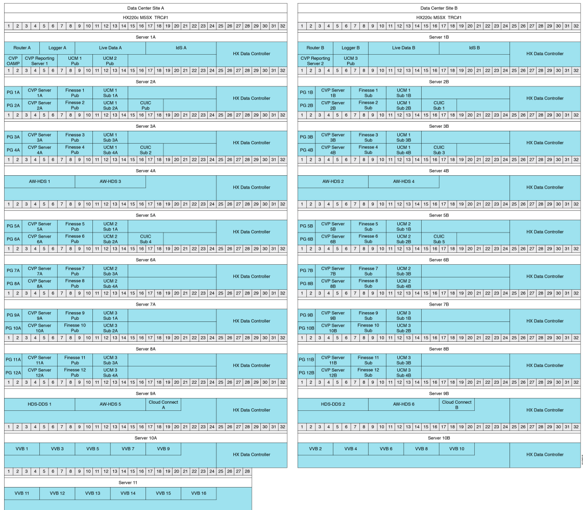
Figure 17: 24000 Agent Reference Design Model
