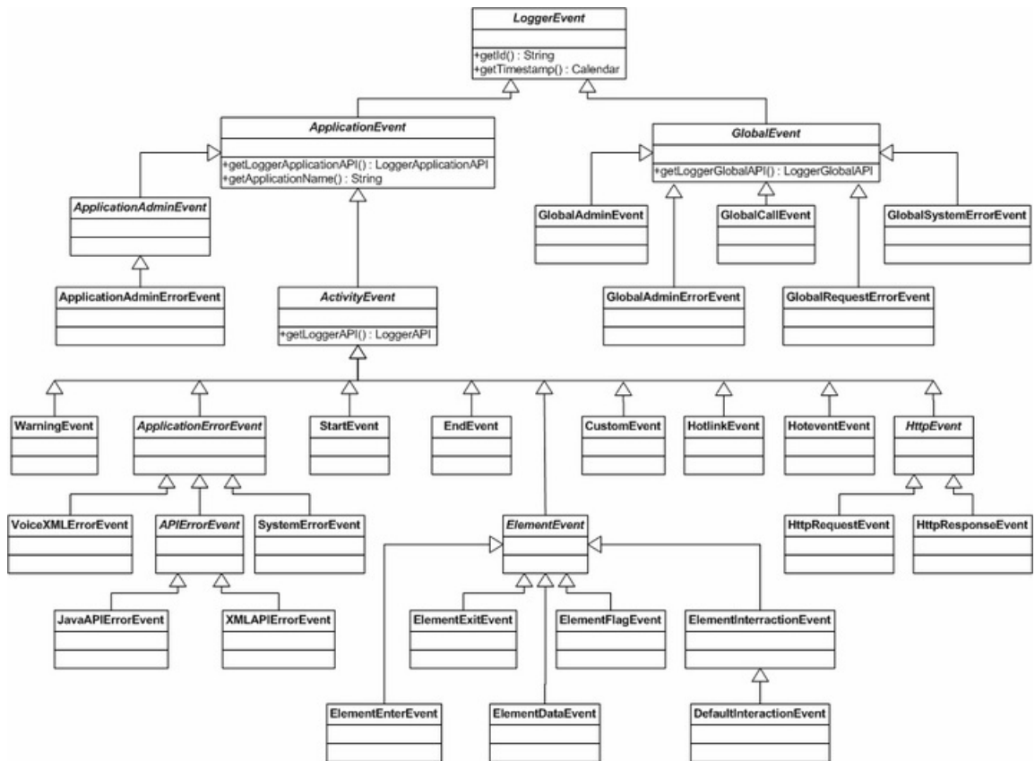
Figure 11: Logger Event
