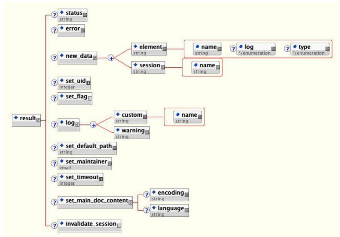
Figure 8: ActionElementsDTD
