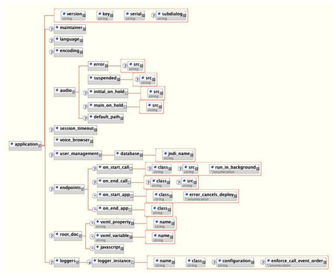
Figure 3: DTD Diagram for XML Document Sent to All Components in Settings Argument
