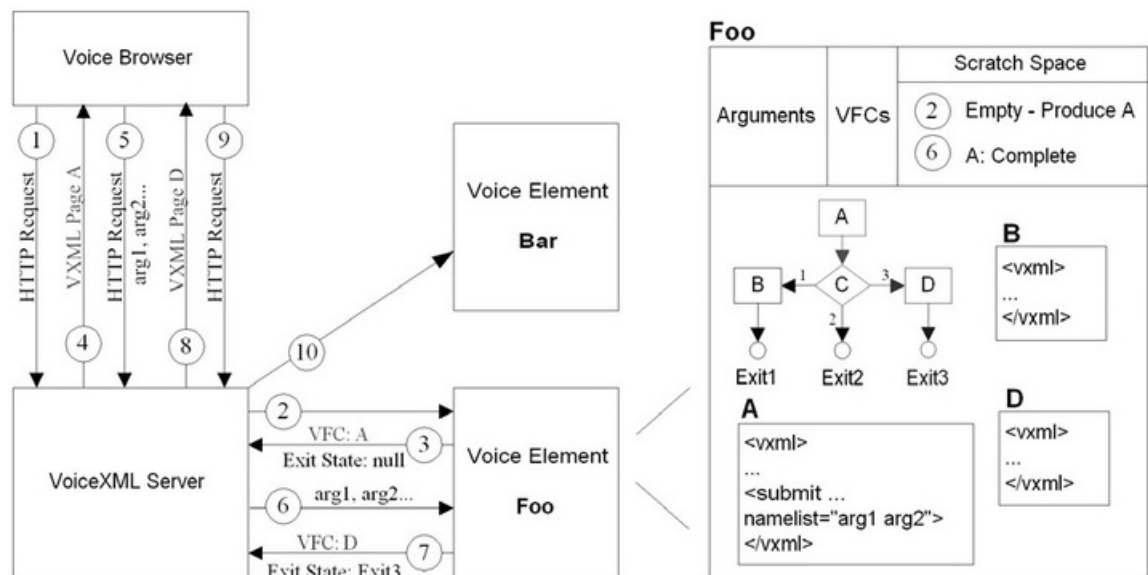
Figure 10: Voice Element Interaction with the VXML Server and the Voice Browser
