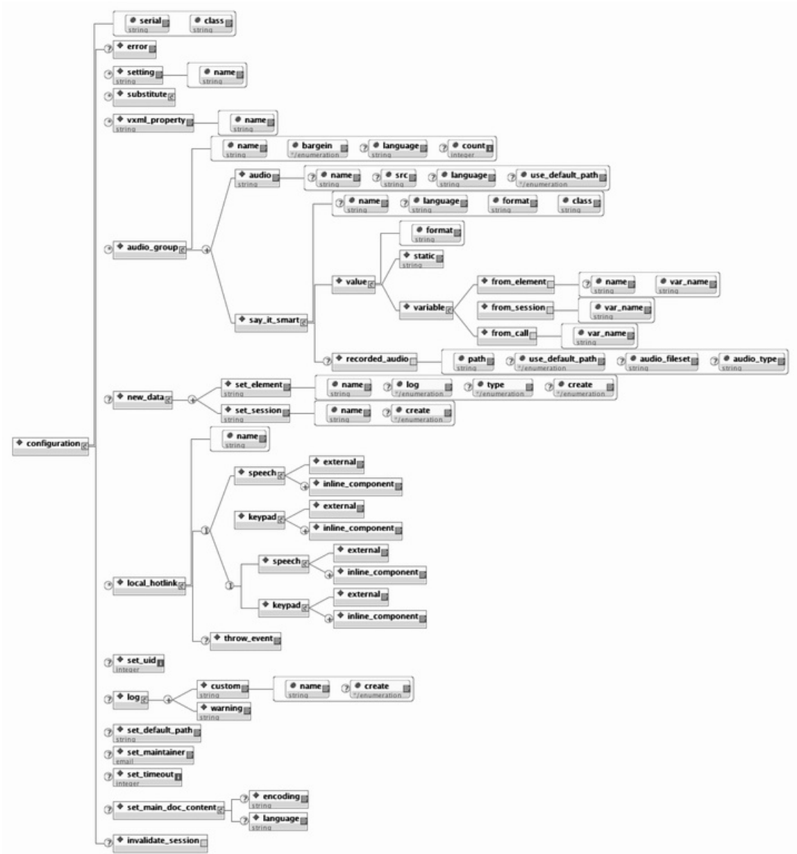
Figure 6: Voice Element Configuration DTD
