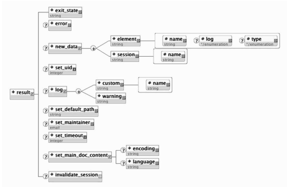
Figure 9: Standard Decision Elements DTD Diagram
