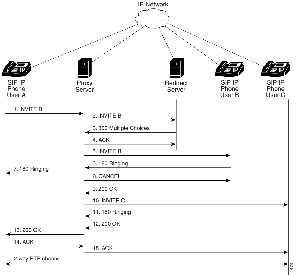
Figure B-12 Cisco SIP IP Phone-to-Cisco SIP IP Phone Network Call Forwarding (No Answer)
