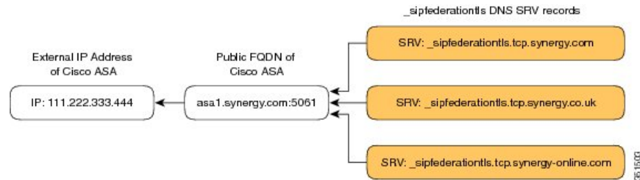
Figure 15: SIP DNS SRV Resolving to FQDN of the Cisco Expressway-C
