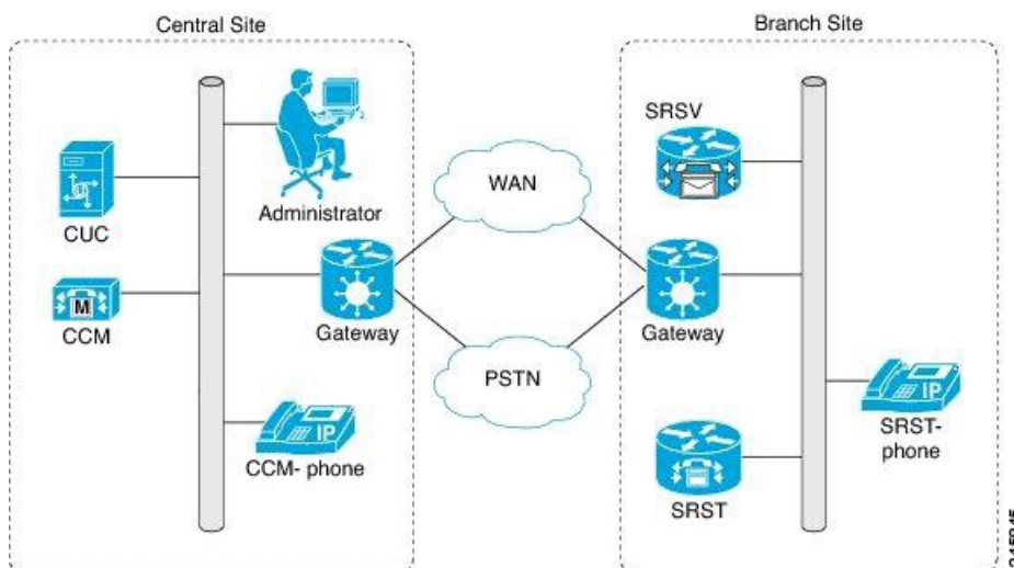
Figure 16: Topology 2
