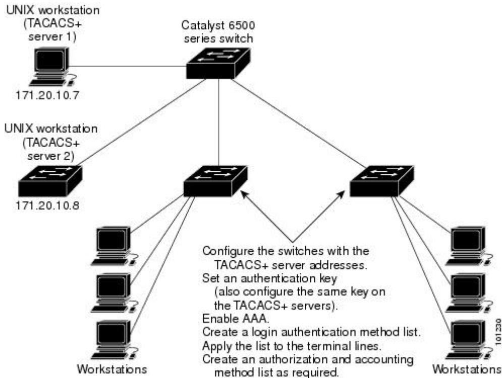
Figure 70: Typical TACACS+ Network Configuration
