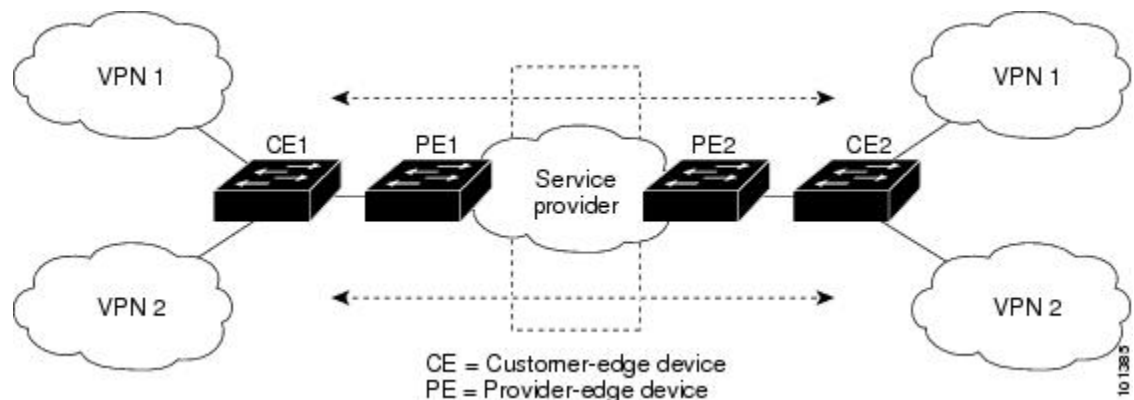
Figure 68: Switches Acting as Multiple Virtual CEs
