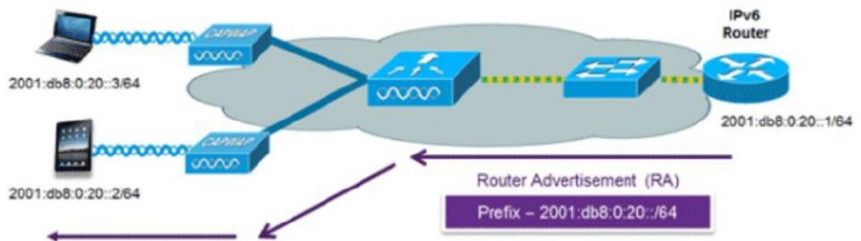
Figure 16: SLAAC Address Assignment
