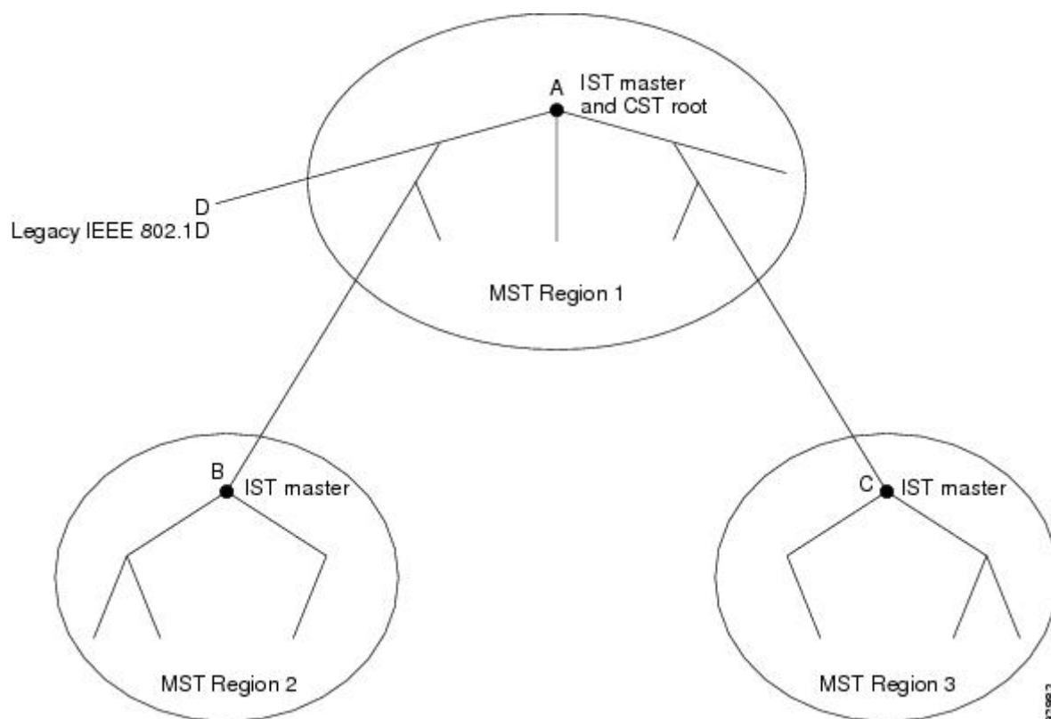
Figure 25: MST Regions, CIST Masters, and CST Root
