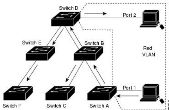
Figure 100: Optimized Flooded Traffic VTP Pruning
