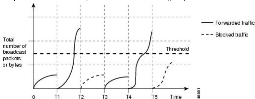
Figure 96: Broadcast Storm Control Example
