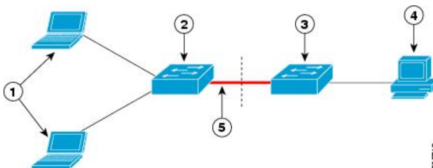
Figure 90: Authenticator and Supplicant Switch using CISP
