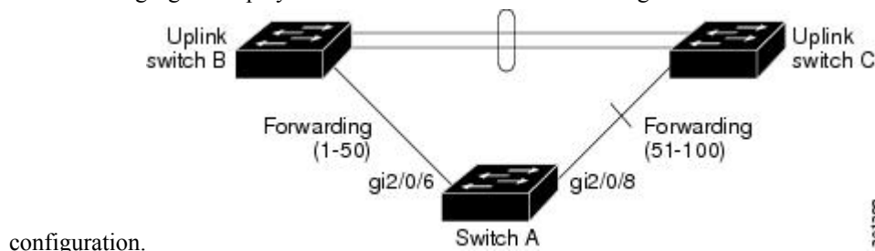
Figure 45: VLAN Flex Links Load-Balancing Configuration Example
