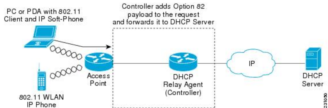
Figure 105: DHCP Option 82
