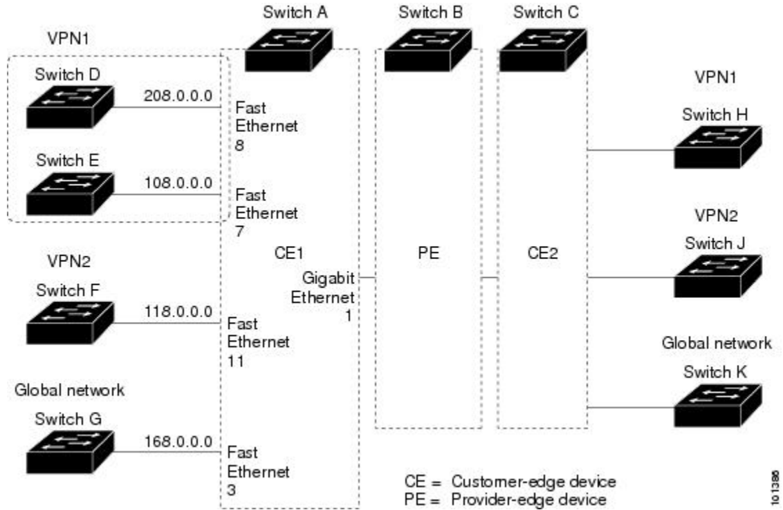
Figure 69: Multi-VRF CE Configuration Example
