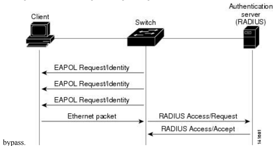
Figure 88: Message Exchange During MAC Authentication Bypass
