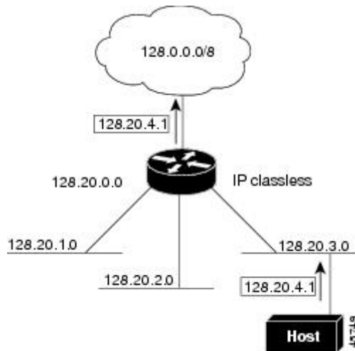
Figure 64: IP Classless Routing
