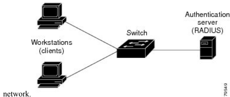
Figure 91: Web-Based Authentication Device Roles
