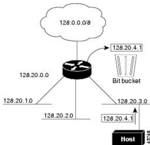
Figure 65: No IP Classless Routing
