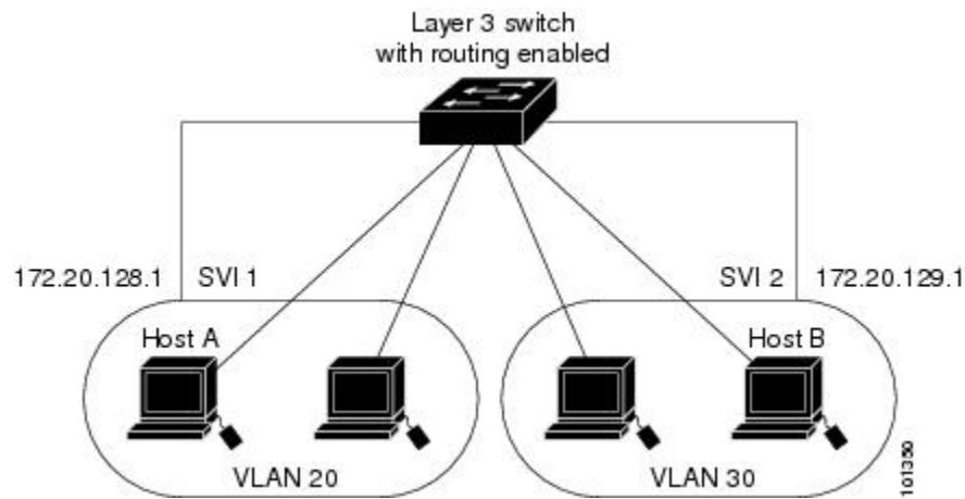
Figure 2: Connecting VLANs with the Switch
