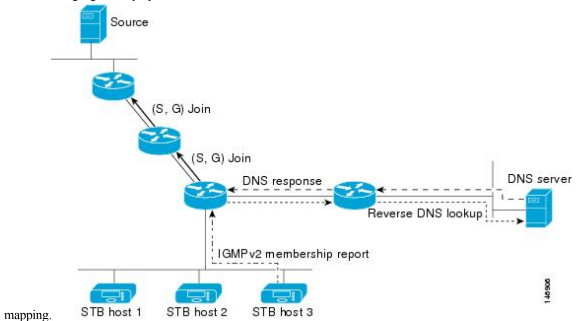
Figure 12: DNS-Based SSM Mapping
