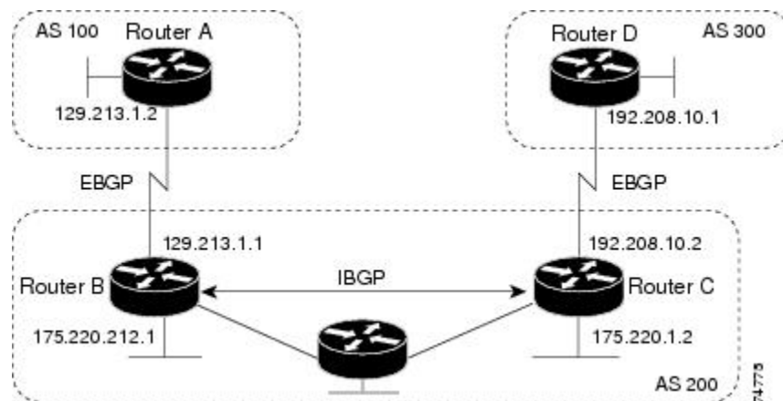
Figure 67: EBGP, IBGP, and Multiple Autonomous Systems
