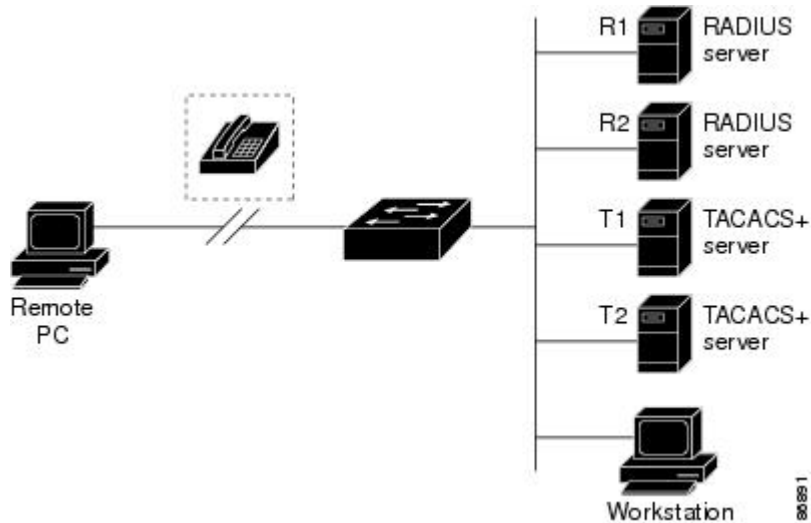
Figure 71: Transitioning from RADIUS to TACACS+ Services
