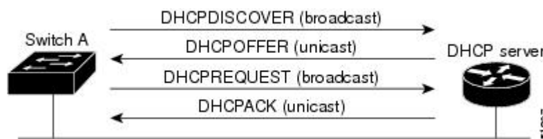
Figure 98: DHCP Client and Server Message Exchange
