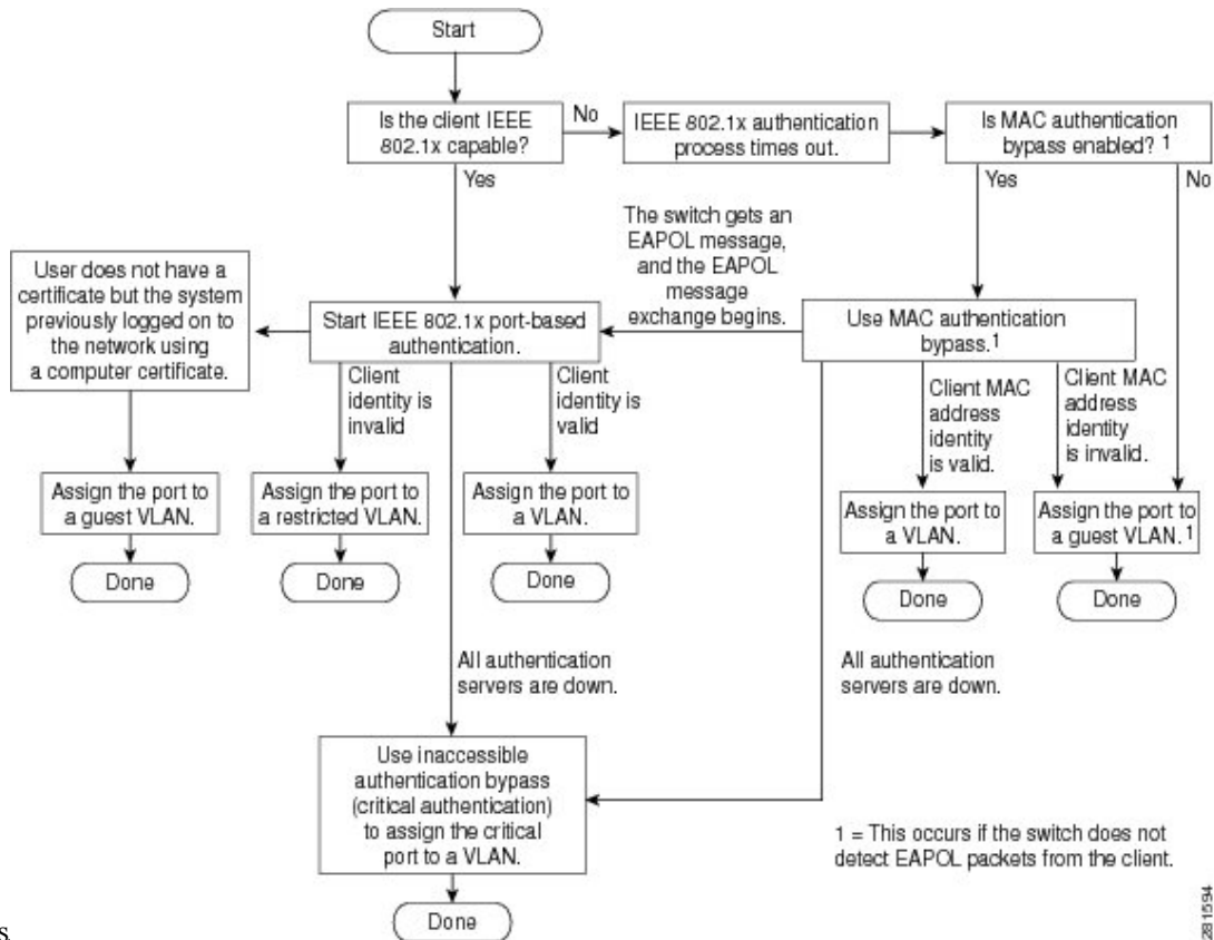
Figure 86: Authentication Flowchart
