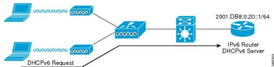
Figure 17: Stateful DHCPv6 Address Assignment
