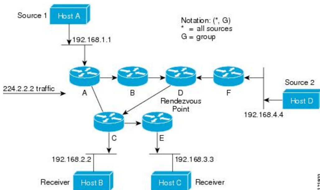
Figure 8: Shared Tree
