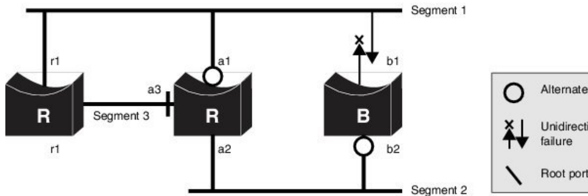
Figure 25: Bridging Loops on Shared Segments
