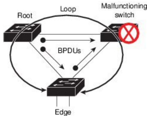
Figure 36: Network Loop Due to a Malfunctioning Switch
