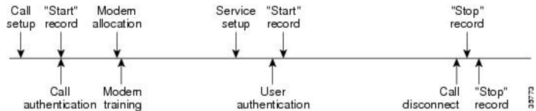
Figure 85: Modem Dial-In Call Setup Sequence With Resource Start-Stop Accounting Enabled
