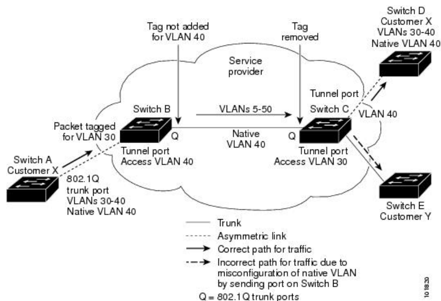
Figure 132: Potential Problems with IEEE 802.1Q Tunneling and Native VLANs
