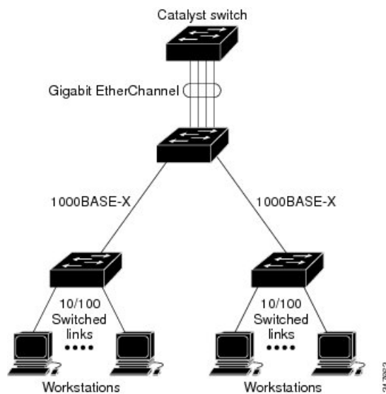
Figure 44: Typical EtherChannel Configuration
