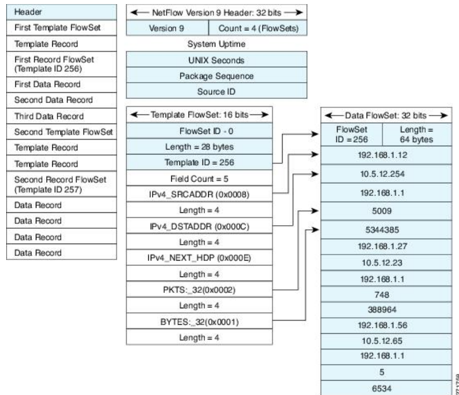
Figure 55: Detailed Example of the NetFlow Version 9 Export Format
