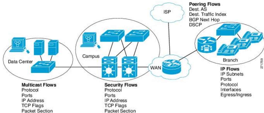
Figure 53: Typical Deployment for Flexible NetFlow
