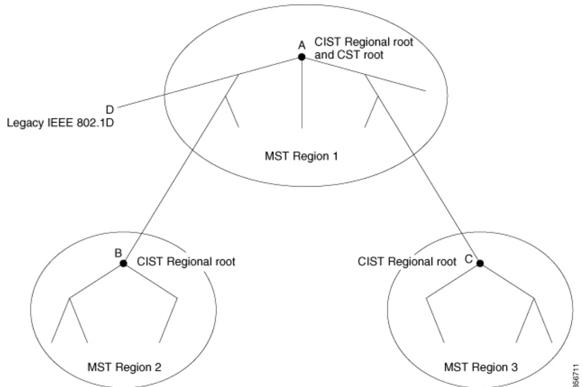
Figure 18: MST Regions, CIST Regional Root, and CST Root
