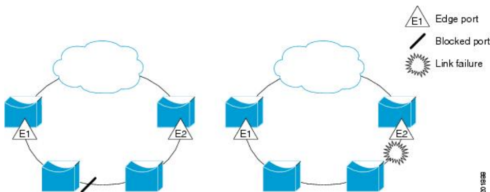
Figure 39: REP Open Segment
