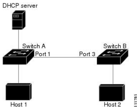
Figure 101: ARP Packet Validation on a VLAN Enabled for Dynamic ARP Inspection
