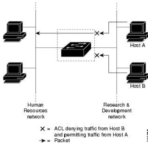
Figure 87: Using ACLs to Control Traffic in a Network
