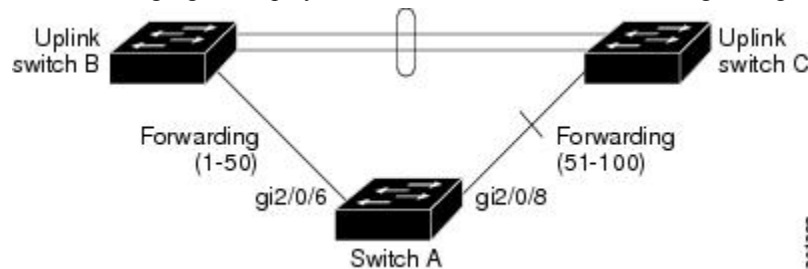
Figure 51: VLAN Flex Links Load-Balancing Configuration Example
