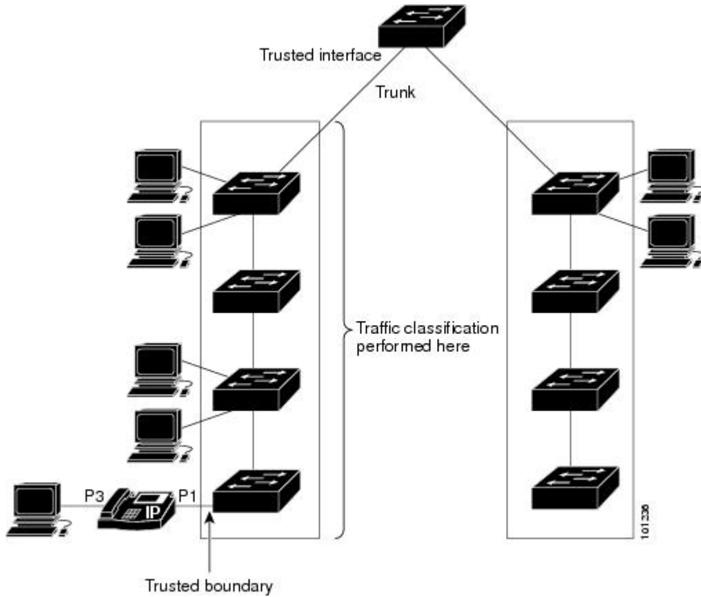
Figure 68: Port Trusted States on Ports Within the QoS Domain
