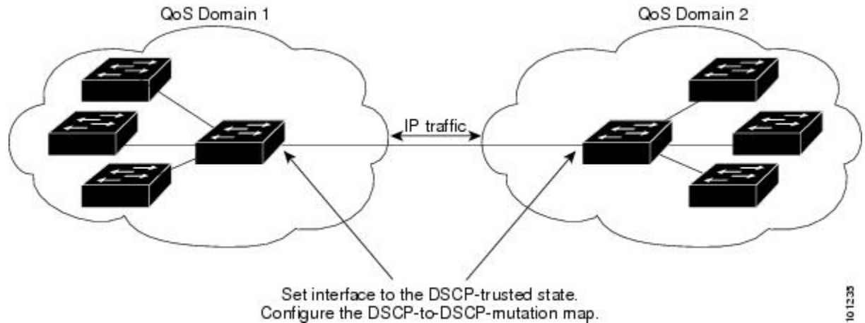
Figure 69: DSCP-Trusted State on a Port Bordering Another QoS Domain
