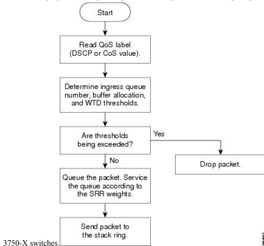
Figure 64: Queueing and Scheduling Flowchart for Ingress Ports on Catalyst 3750-E and 3750-X Switches
