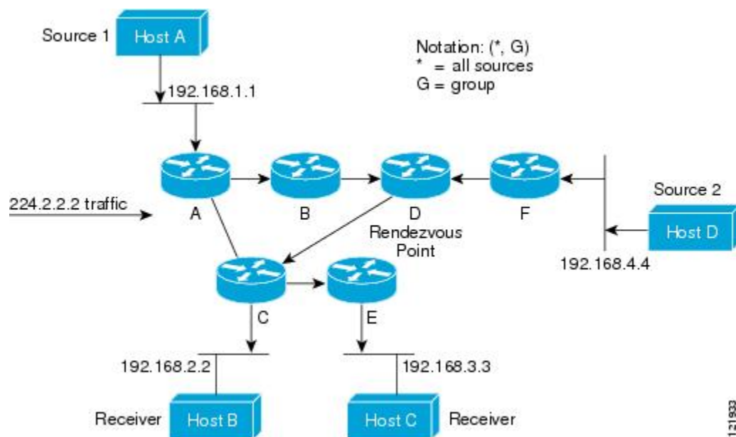
Figure 8: Shared Tree
