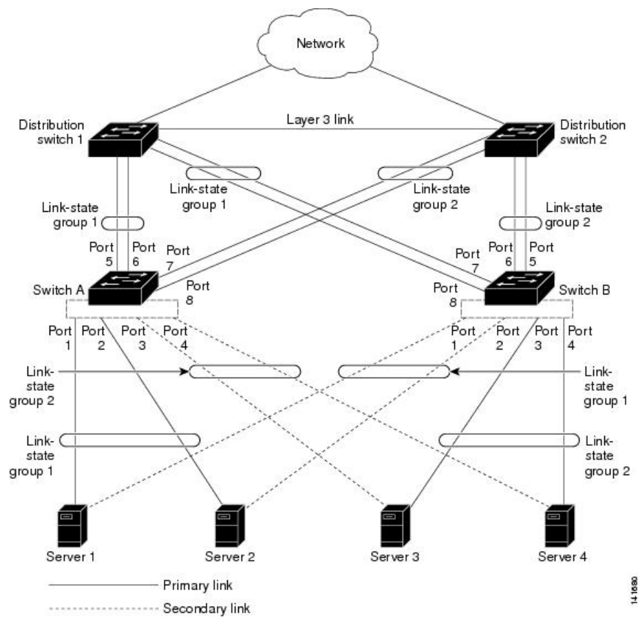
Figure 49: Typical Link-State Tracking Configuration
