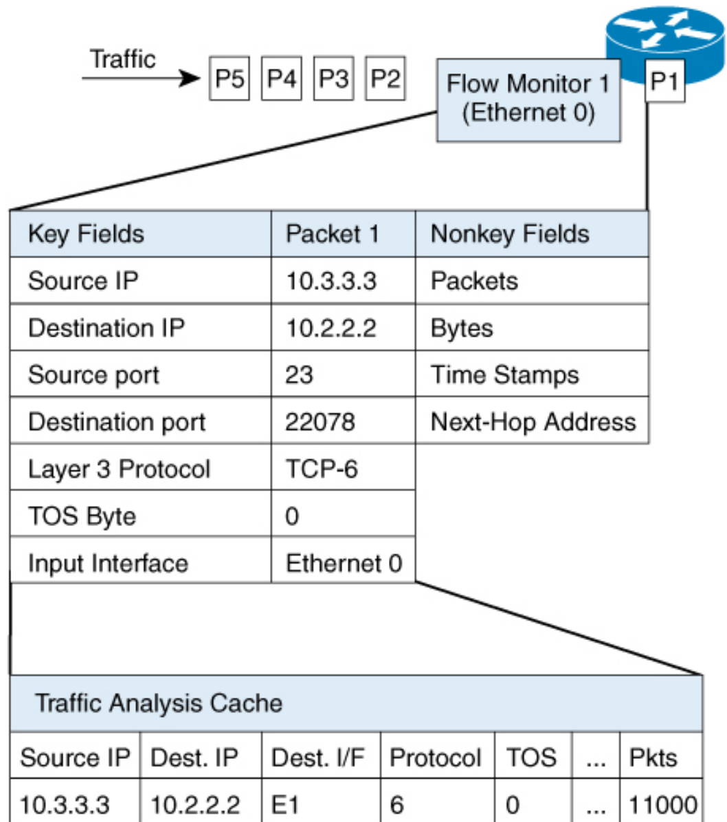
Figure 56: Example of Using a Flow Monitor to Analyze Incoming Traffic
