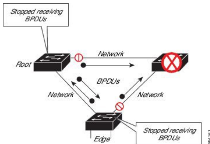
Figure 38: Network Problem Averted with Bridge Assurance Enabled
