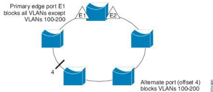
Figure 43: Example of VLAN Blocking
