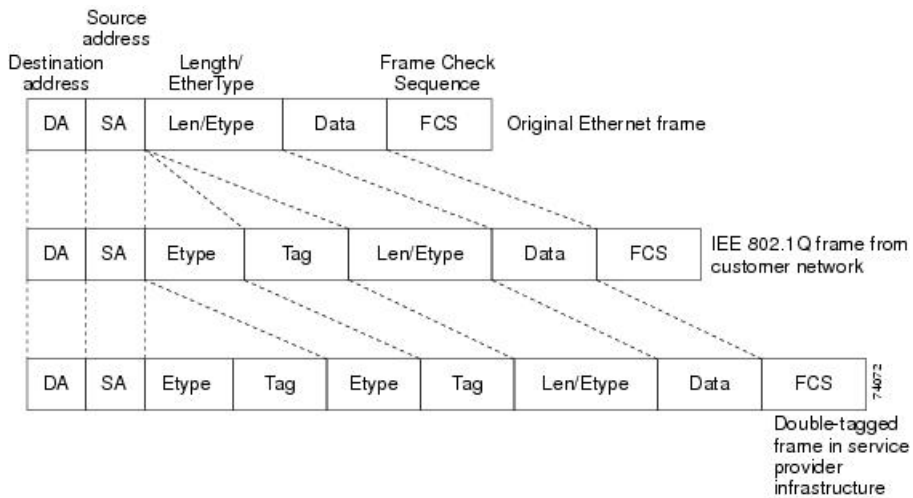
Figure 131: Original (Normal), IEEE 802.1Q, and Double-Tagged Ethernet Packet Formats
