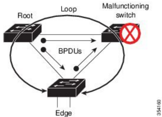
Figure 36: Network Loop Due to a Malfunctioning Switch
