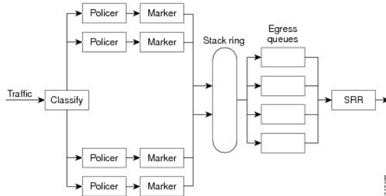
Figure 62: Egress Queue Location on Switch
