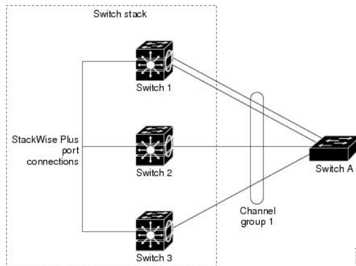
Figure 46: Cross-Stack EtherChannel
