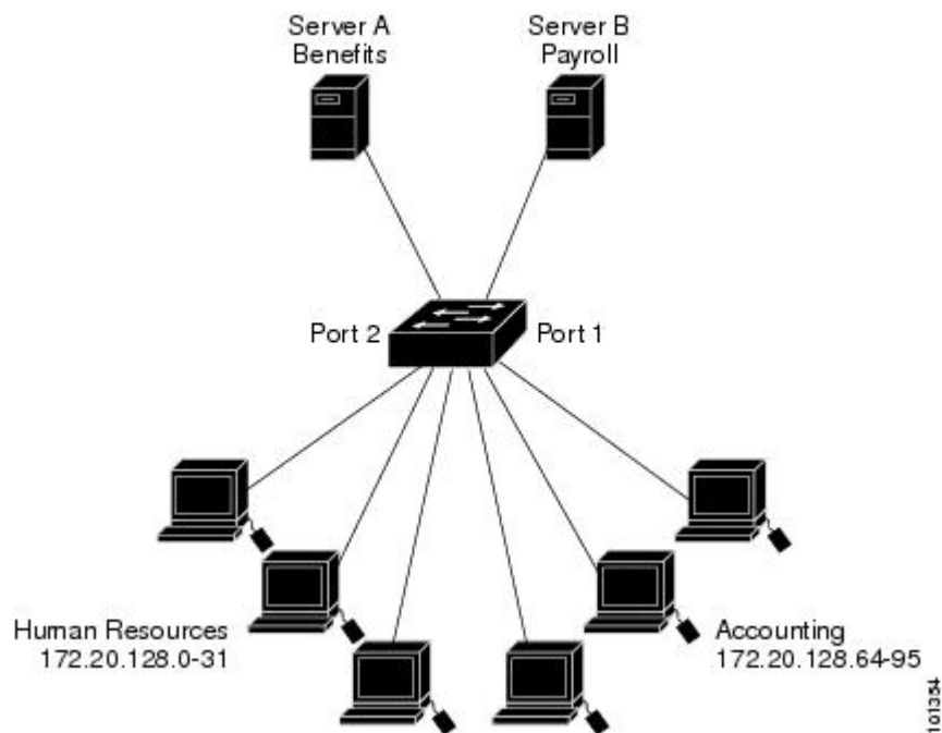
Figure 89: Using Router ACLs to Control Traffic
