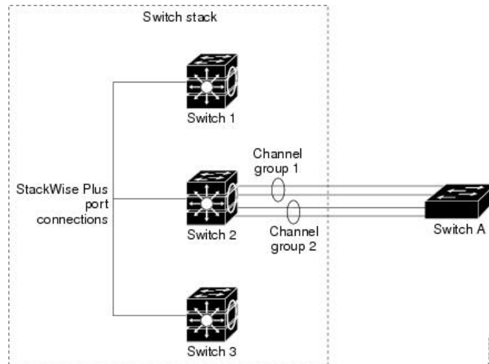
Figure 46: Cross-Stack EtherChannel
