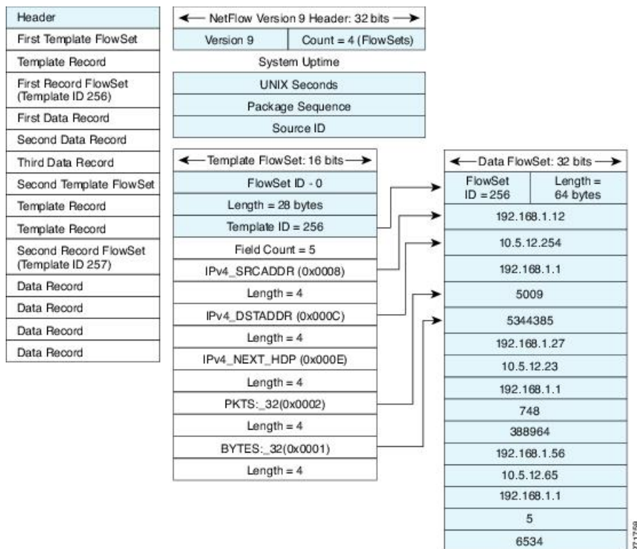
Figure 50: Detailed Example of the NetFlow Version 9 Export Format
