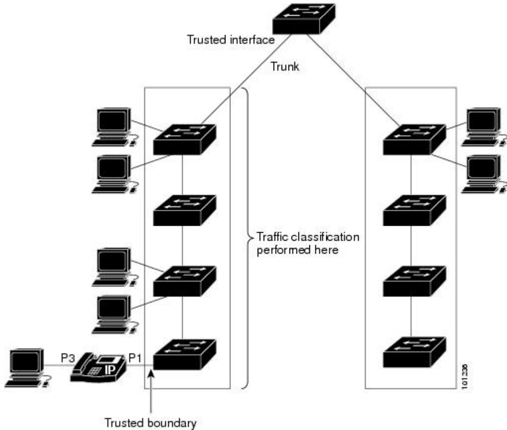
Figure 63: Port Trusted States on Ports Within the QoS Domain
