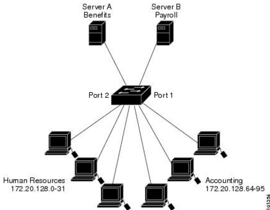
Figure 77: Using Router ACLs to Control Traffic
