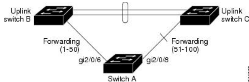
Figure 40: VLAN Flex Links Load-Balancing Configuration Example
