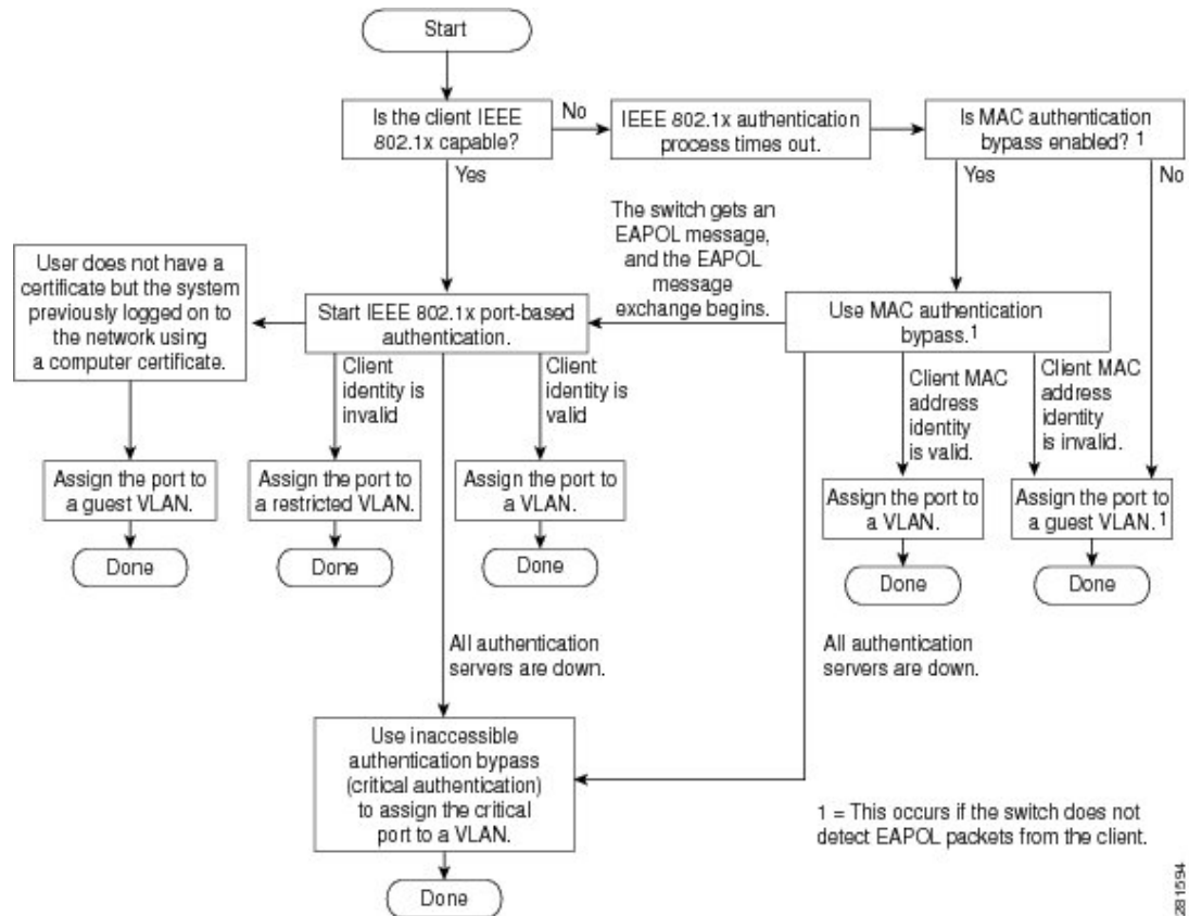
Figure 90: Authentication Flowchart
