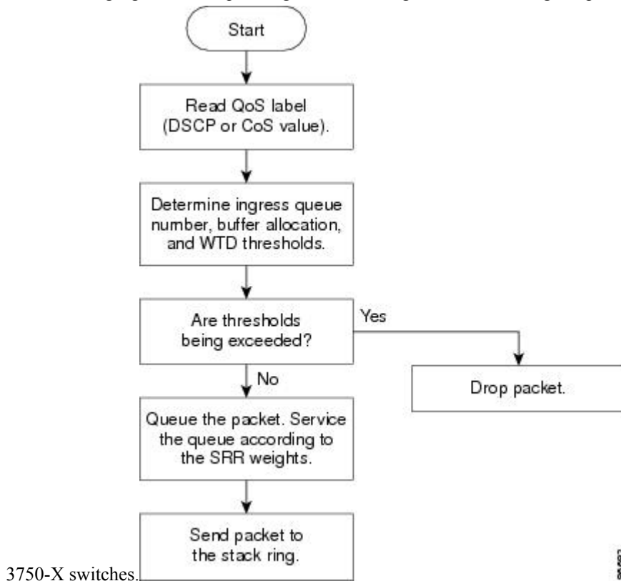
Figure 59: Queueing and Scheduling Flowchart for Ingress Ports on Catalyst 3750-E and 3750-X Switches
