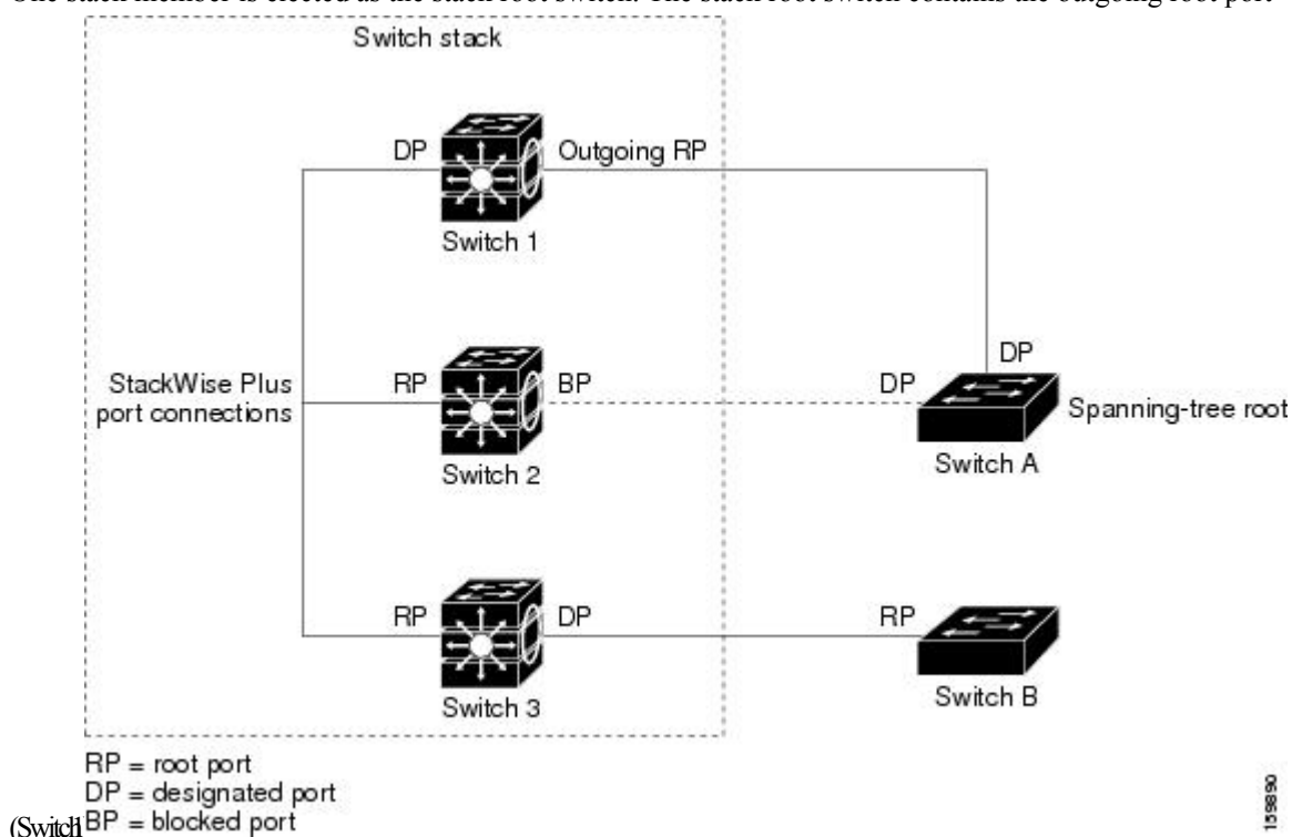
Figure 8: Spanning-Tree Port States in a Switch Stack
