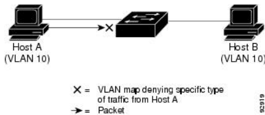
Figure 78: Using VLAN Maps to Control Traffic
