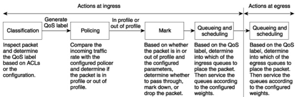
Figure 54: QoS Basic Wired Model
