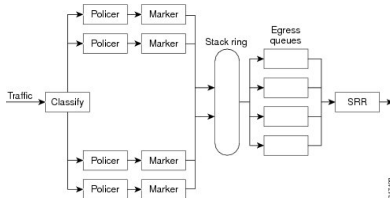
Figure 57: Egress Queue Location on Switch
