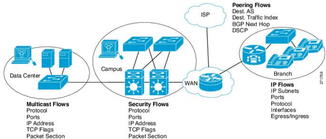
Figure 48: Typical Deployment for Flexible NetFlow
