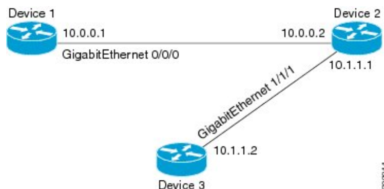
Figure 76: Topology for Applying Access Control Lists
