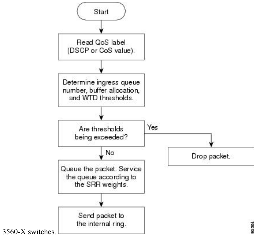
Figure 59: Queueing and Scheduling Flowchart for Ingress Ports on Catalyst 3560-E and 3560-X Switches
