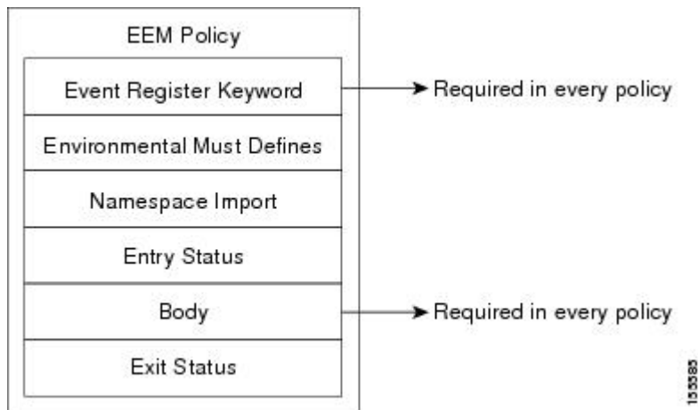
Figure 112: Tcl Policy Structure and Requirements
