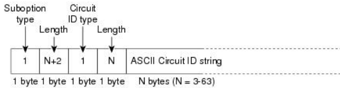
Figure 88: User-Configured Suboption Packet Formats
