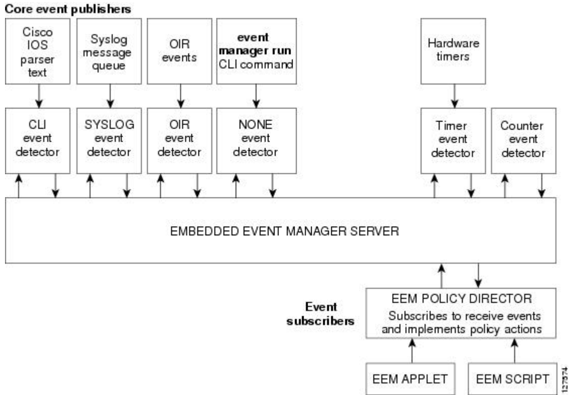
Figure 109: Embedded Event Manager Core Event Detectors
