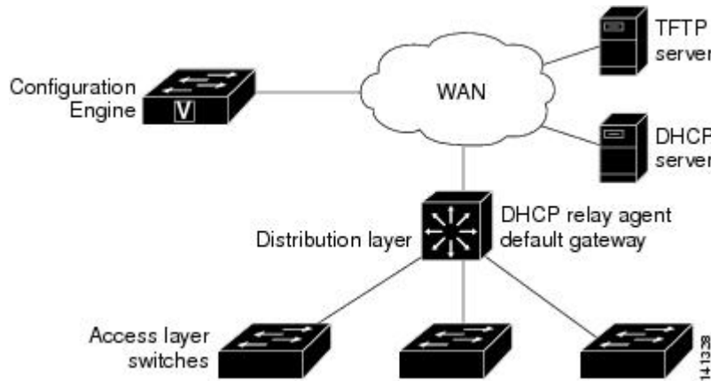
Figure 43: Initial Configuration
