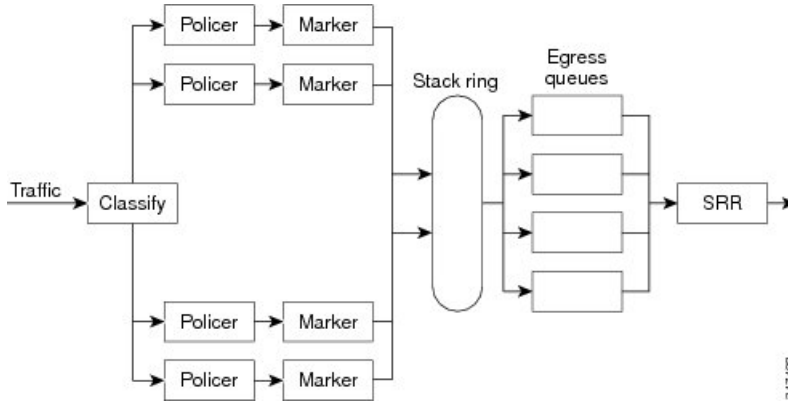
Figure 56: Egress Queue Location on Switch
