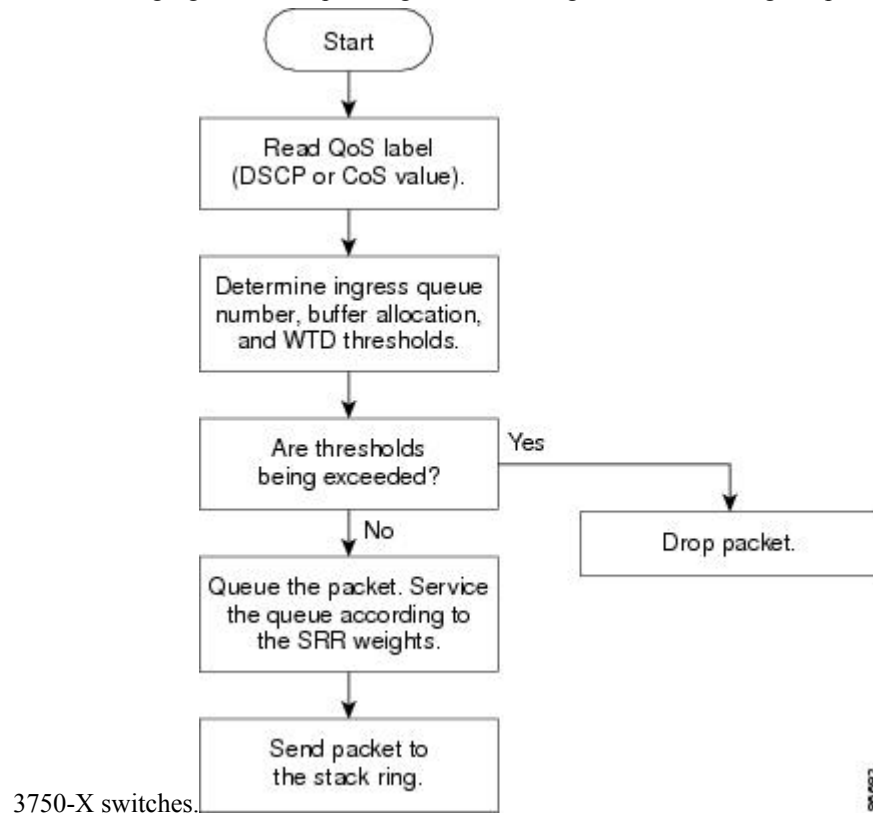
Figure 58: Queueing and Scheduling Flowchart for Ingress Ports on Catalyst 3750-E and 3750-X Switches
