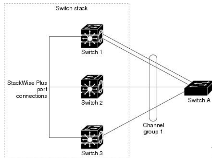
Figure 35: Cross-Stack EtherChannel
