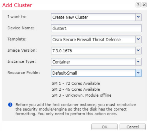
Figure 274: Multi-Instance Cluster
