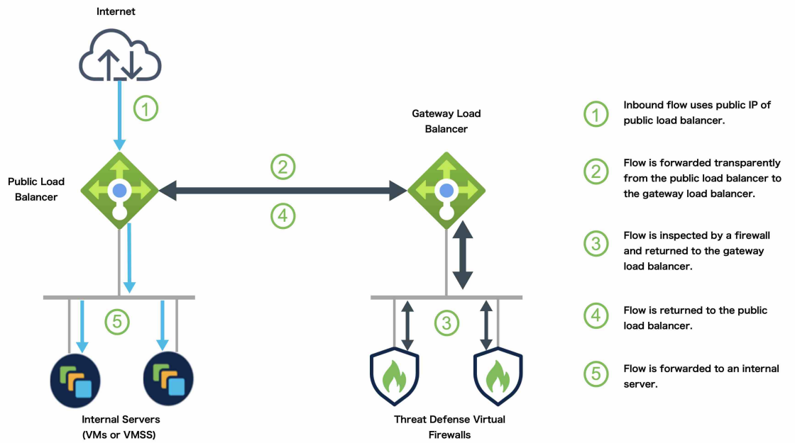
Figure 249: Inbound Traffic Use Case and Topology with GWLB
