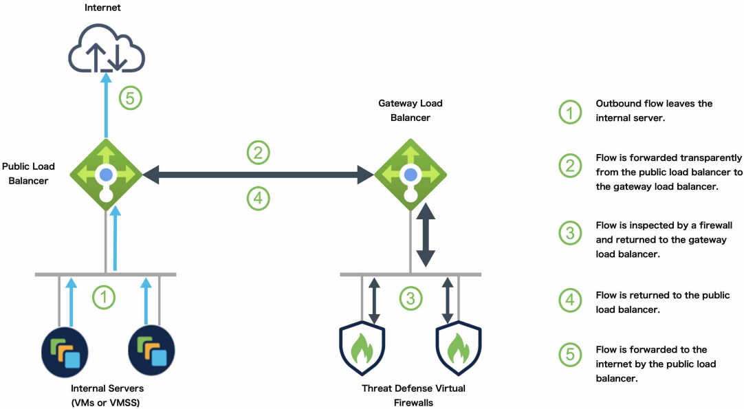
Figure 250: Outbound Traffic Use Case and Topology with GWLB
