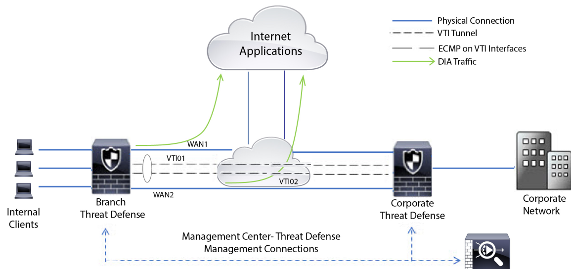
Figure 389: Configuring Policy Based Routing on Branch Threat Defense in Management Center
