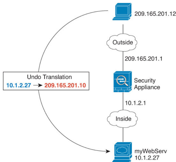
Figure 372: Static NAT for an Inside Web Server
