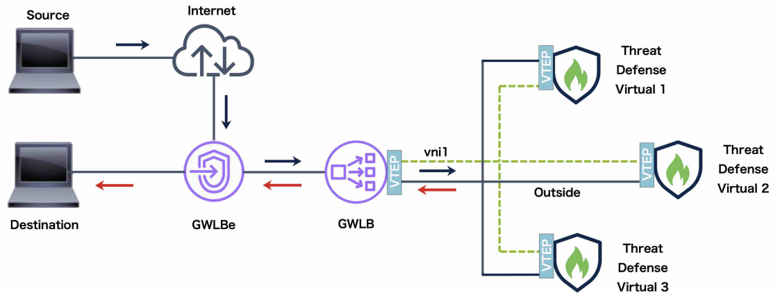
Figure 243: Geneve Single-Arm Proxy
