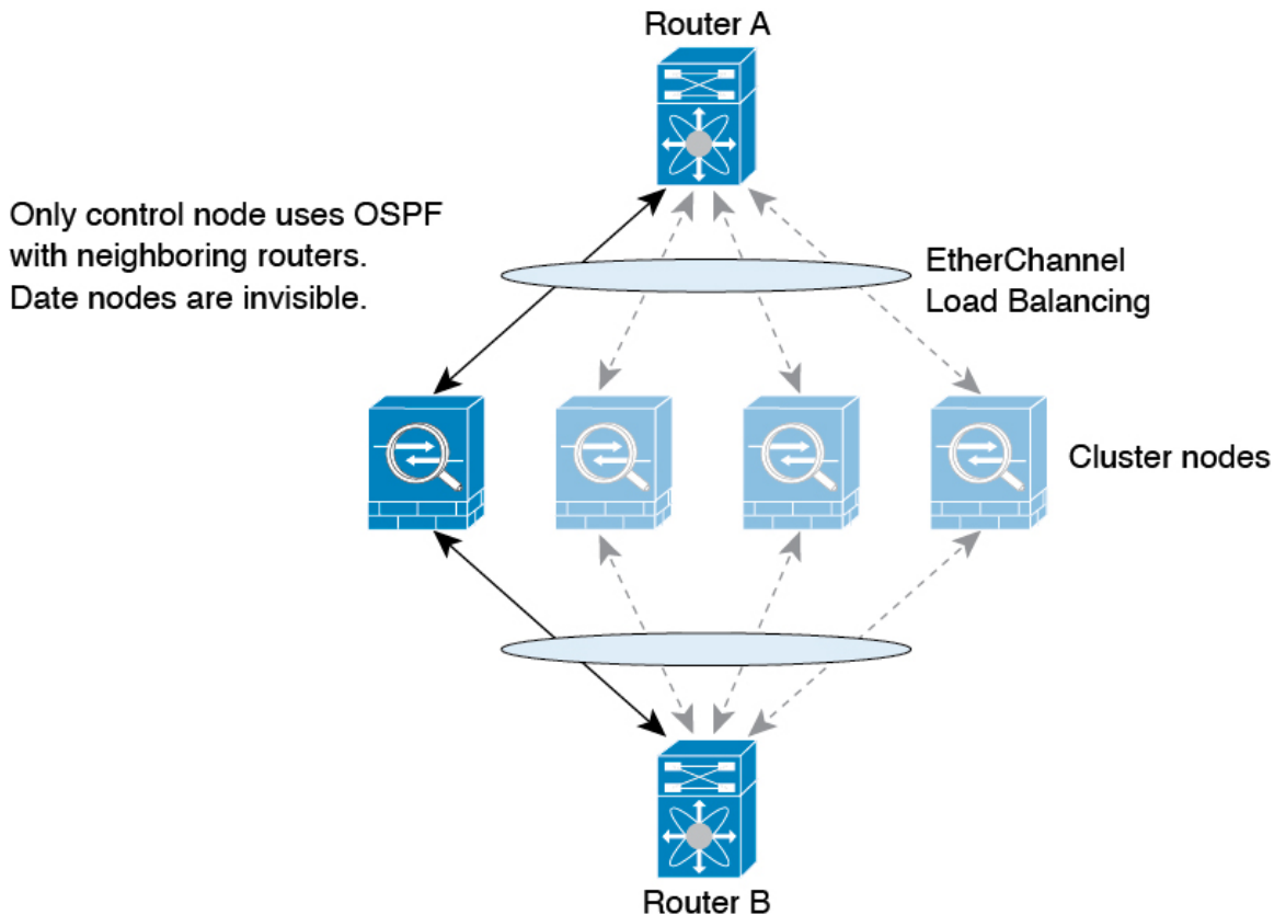
Figure 379: Dynamic Routing in Spanned EtherChannel Mode
