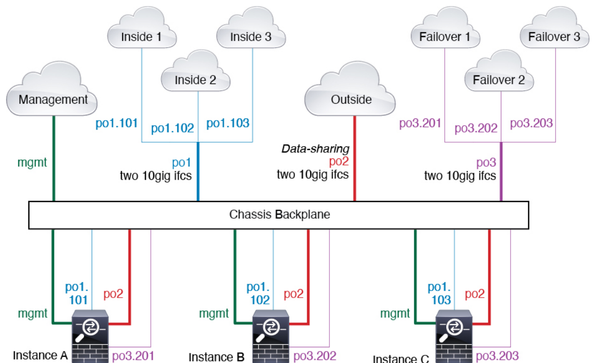
Figure 119: Typical Multi-Instance Deployment
