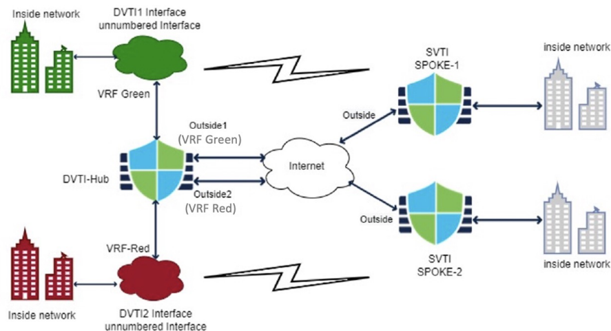
Figure 382: Site-to-Site VPNs with Multiple Virtual Routers and Dynamic VTI
