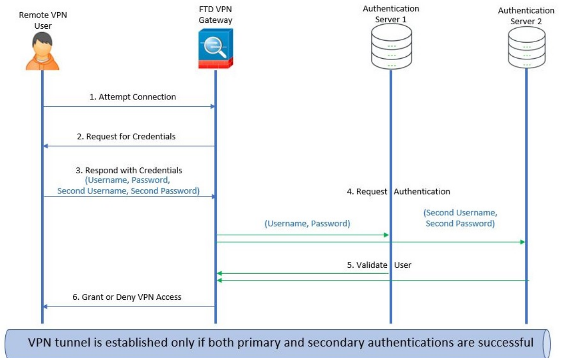
Figure 405: Remote Access VPN Secondary or Double Authentication
