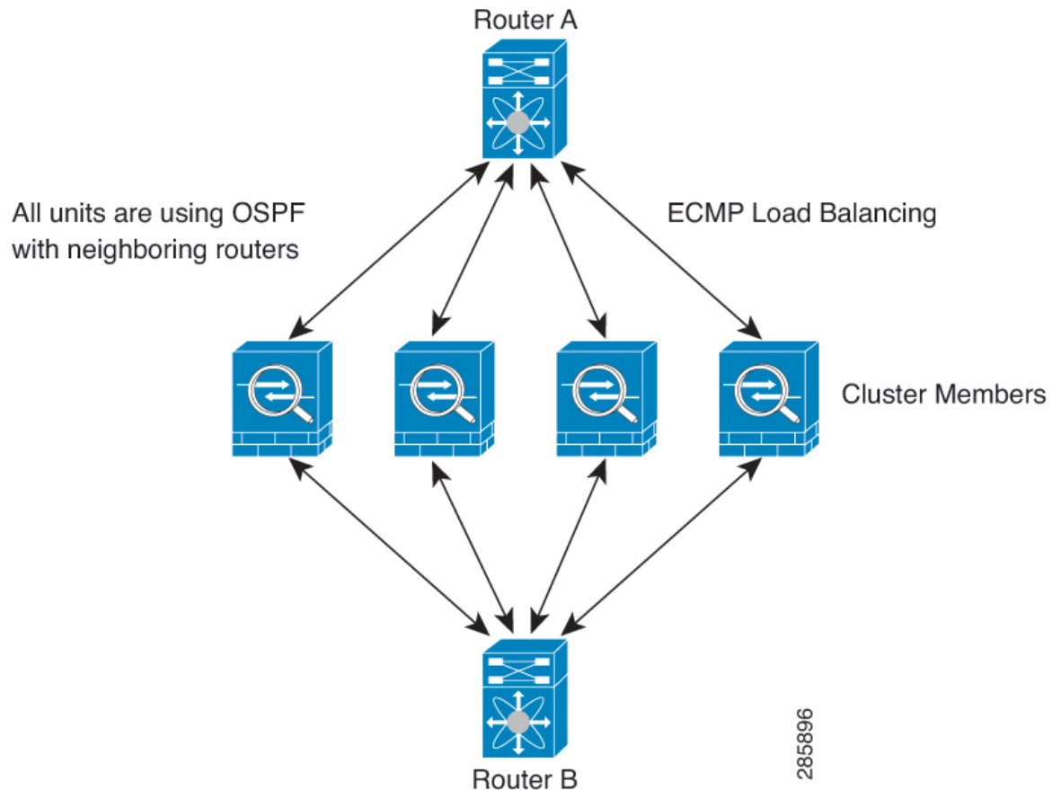
Figure 380: Dynamic Routing in Individual Interface Mode
