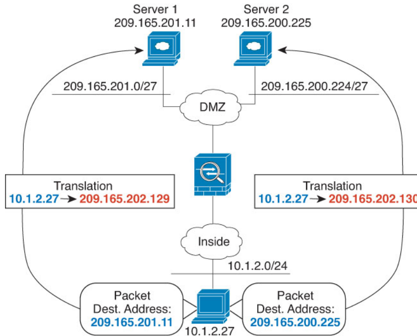
Figure 376: Manual NAT with Different Destination Addresses
