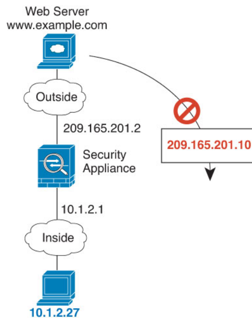
Figure 363: Remote Host Attempts to Initiate a Connection to a Mapped Address
