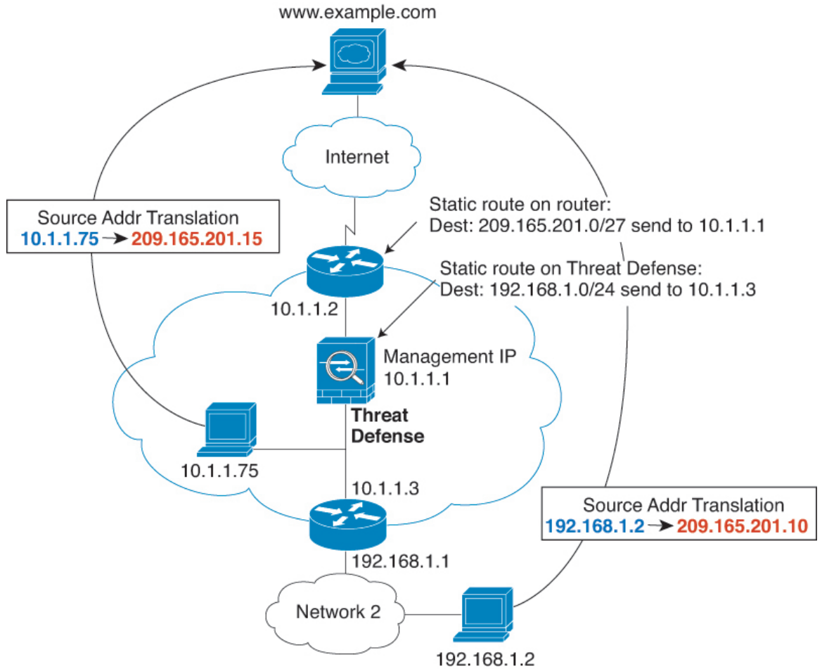
Figure 98: NAT Example: NAT within a Bridge Group
