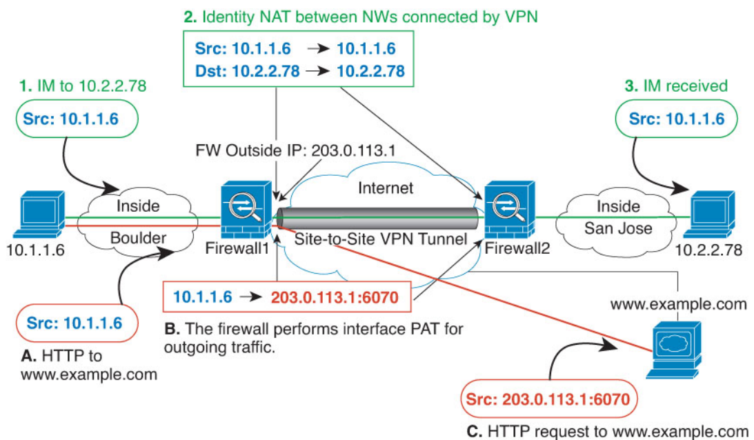
Figure 378: Interface PAT and Identity NAT for Site-to-Site VPN
