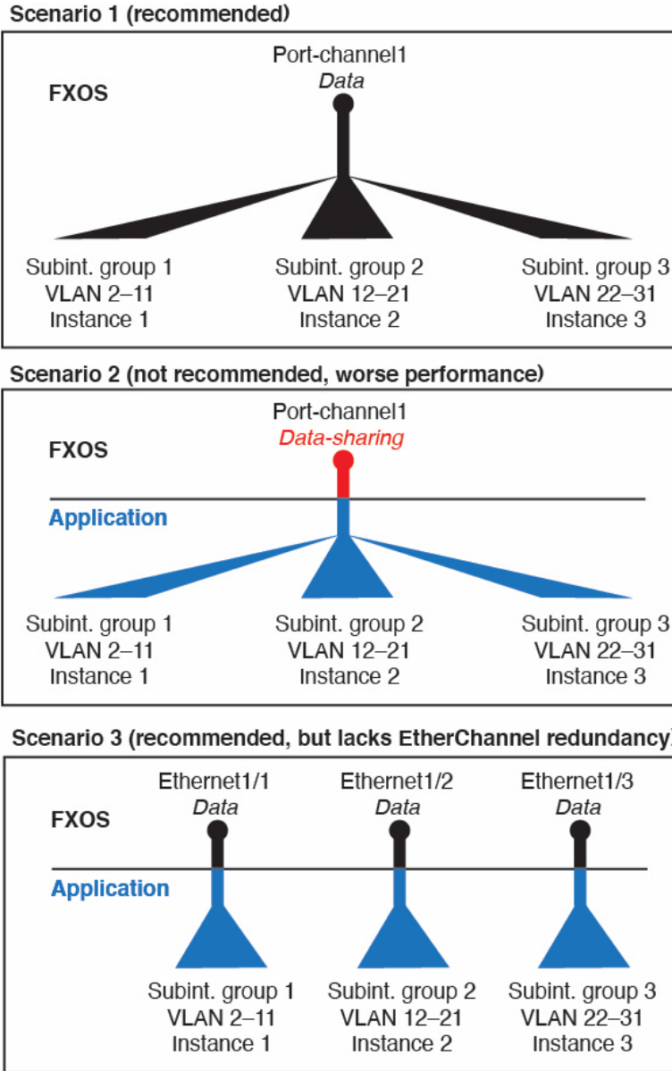
Figure 109: VLANs in the Chassis vs. the Instance
