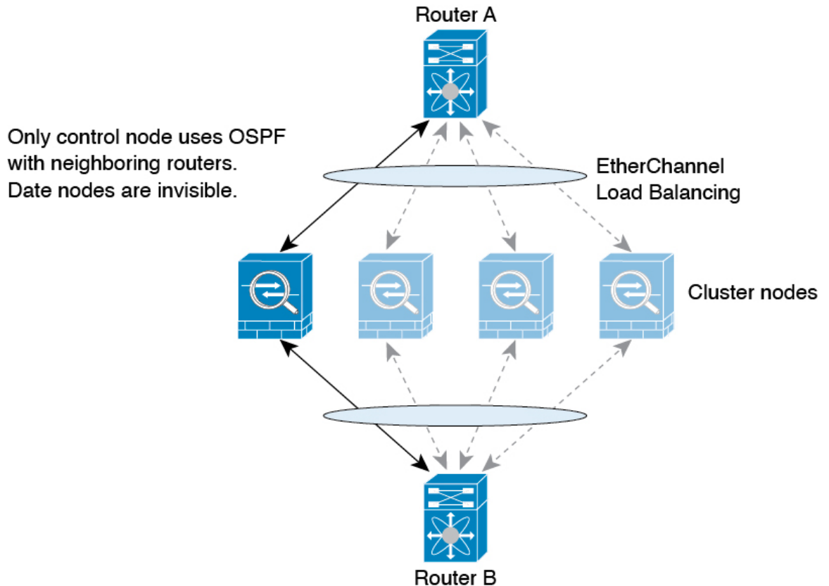
Figure 208: Dynamic Routing in Spanned EtherChannel Mode
