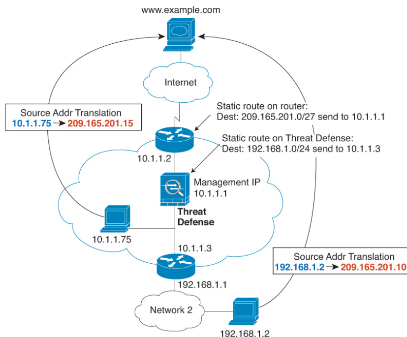
Figure 359: NAT Example: Transparent Mode
