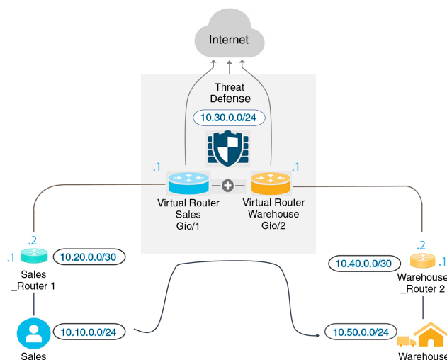
Figure 381: Interconnecting Two Virtual Routers - An Example
