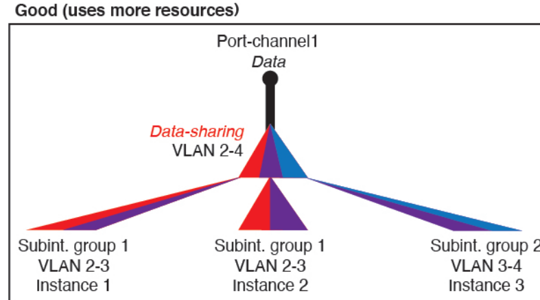
Figure 111: Good: Sharing Multiple Subinterface Groups on One Parent
