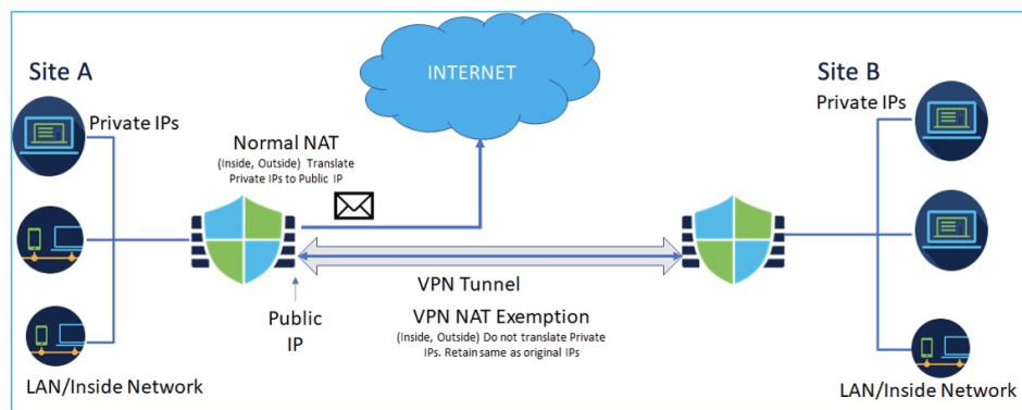
Figure 361: Site-to-site VPN Topology with NAT Exemption
