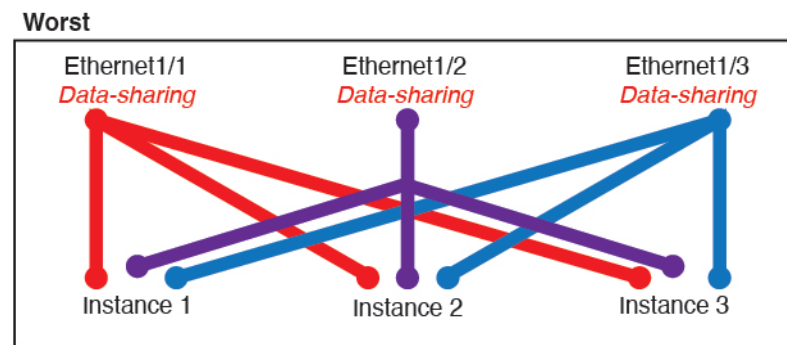
Figure 103: Worst: Shared Parent Interfaces
