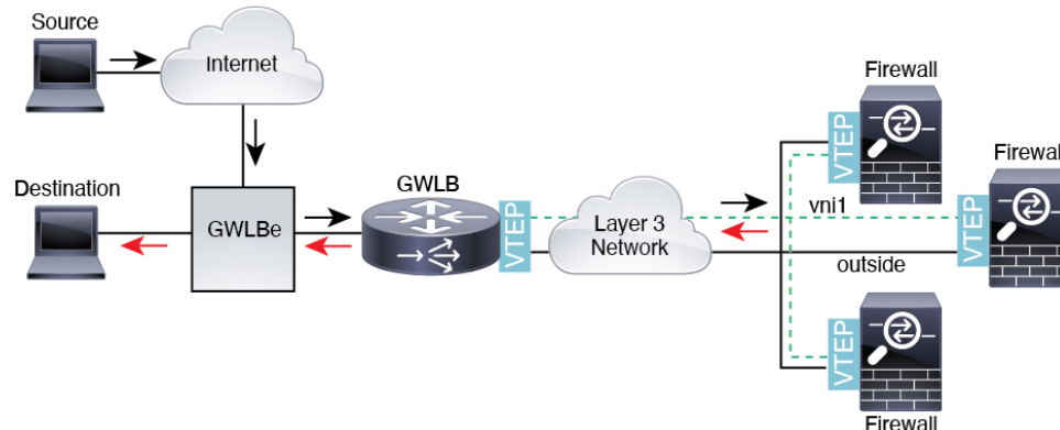
Figure 345: Geneve Single-Arm Proxy
