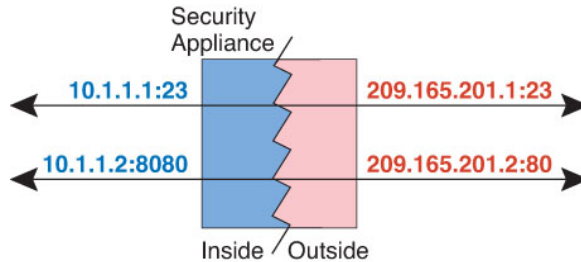
Figure 366: Typical Static NAT with Port Translation Scenario
