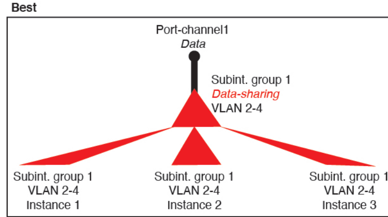
Figure 110: Best: Shared Subinterface Group on One Parent
