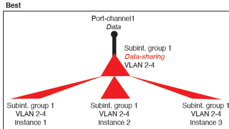
Figure 100: Best: Shared Subinterface Group on One Parent
