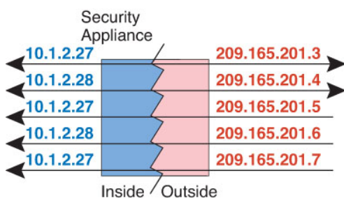
Figure 369: Few-to-Many Static NAT
