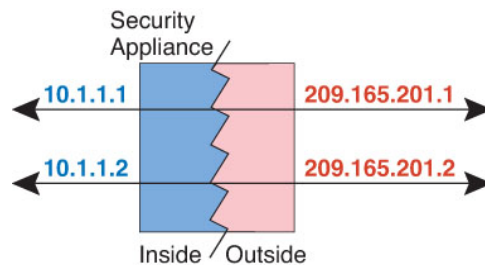
Figure 365: Static NAT
