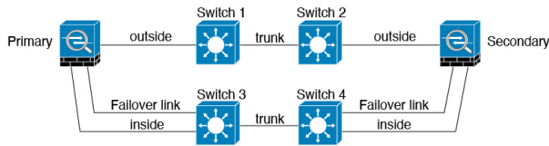
Figure 173: Connecting with a Secure Switch
