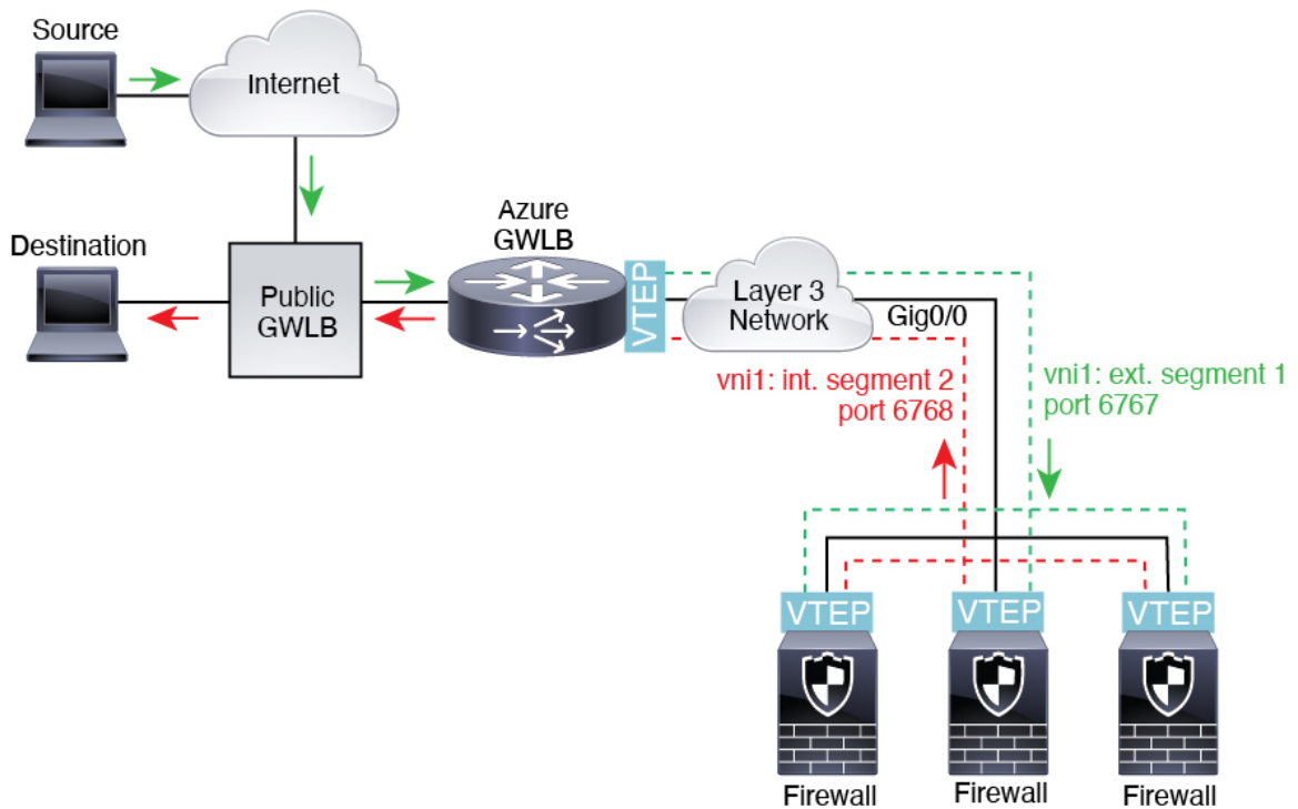
Figure 346: Azure Gateway Load Balancer with Paired Proxy
