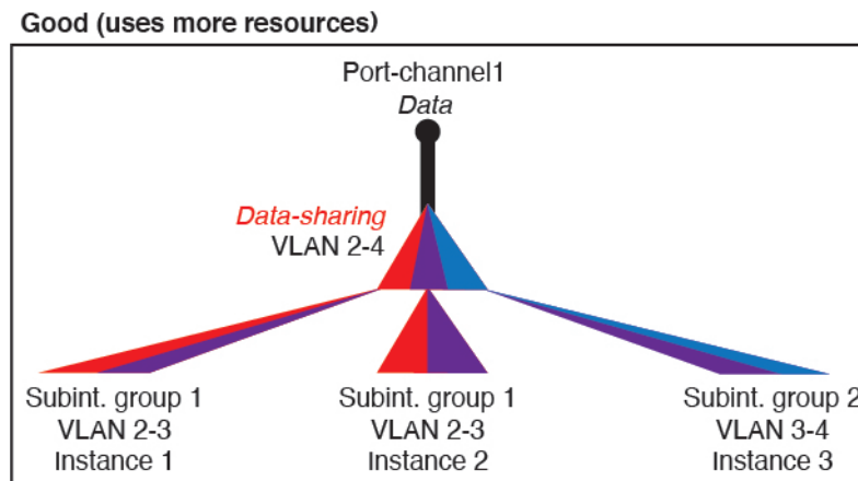
Figure 101: Good: Sharing Multiple Subinterface Groups on One Parent
