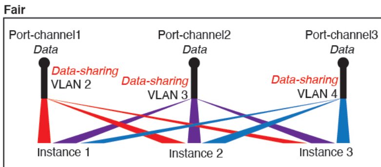
Figure 112: Fair: Shared Subinterfaces on Separate Parents
