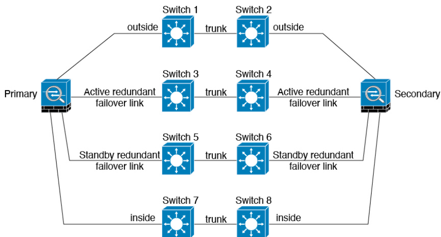
Figure 175: Connecting with Inter-switch Links
