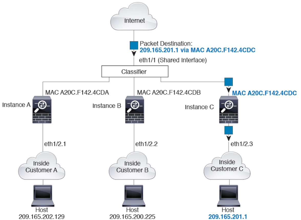
Figure 114: Packet Classification with a Shared Interface Using MAC Addresses
