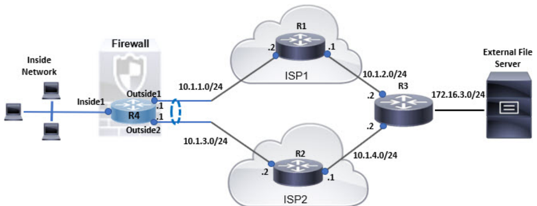
Figure 384: Configuration Example for ECMP
