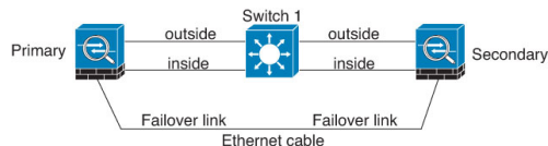
Figure 172: Connecting with a Cable
