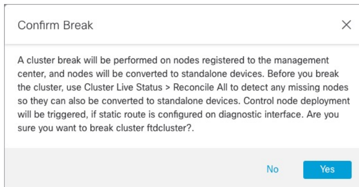
Figure 19: Confirm Break
