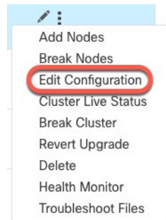
Figure 22: Edit Configuration
