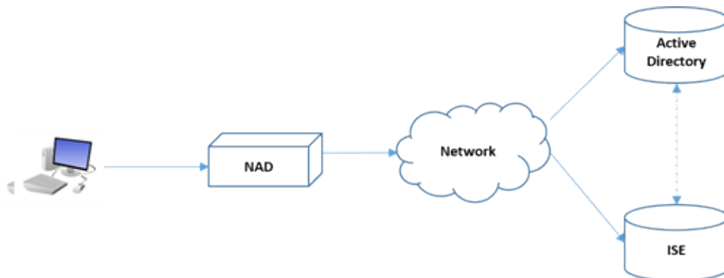
Figure 35: Easy Connect Enforcement Mode Basic Flow
