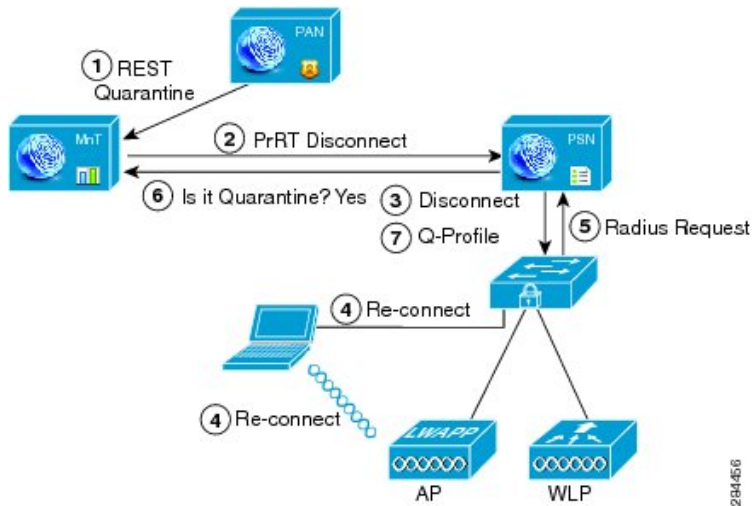
Figure 25: ANC Quarantine Flow
