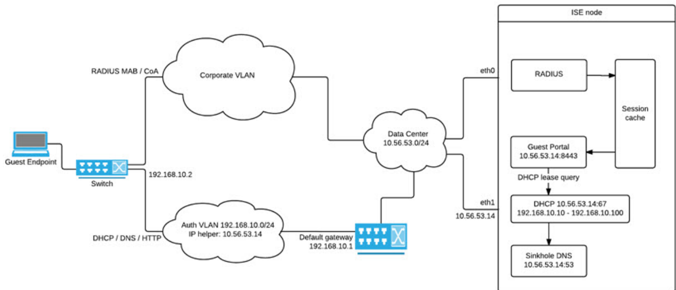
Figure 18: Auth VLAN Configured with IP Helper
