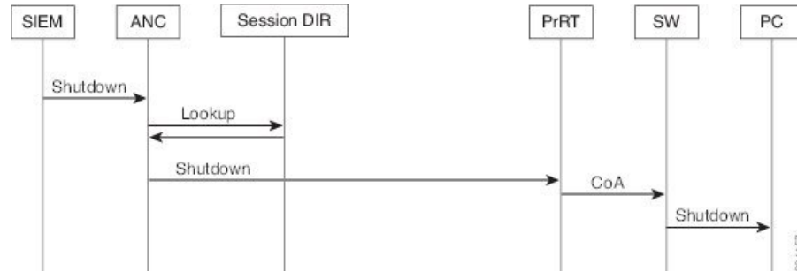
Figure 26: ANC Shutdown Flow
