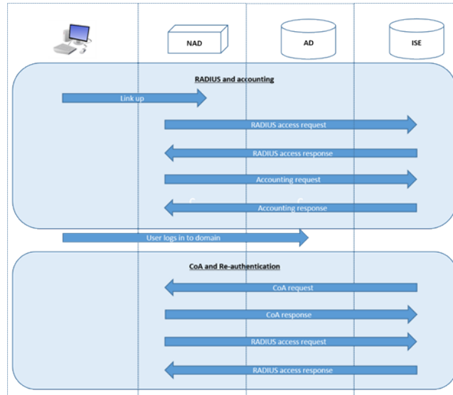
Figure 36: Easy Connect Enforcement Mode Detailed Flow
