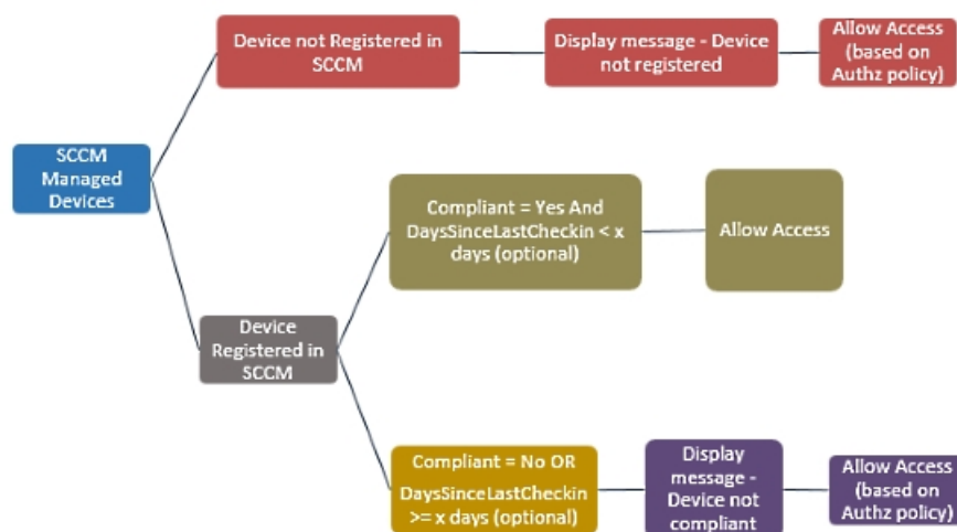
Figure 21: SCCM Workflow
