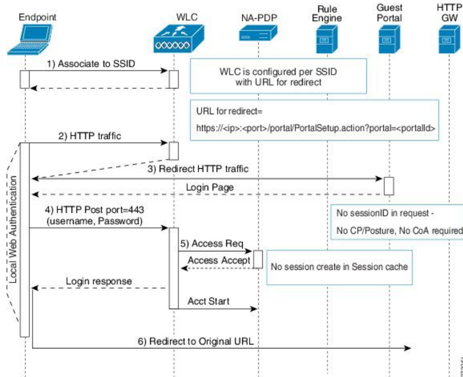
Figure 44: WLC with Local WebAuth Non-Posture Flow
