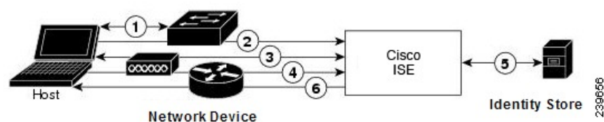
Figure 75: RADIUS-Based Authentication with EAP
