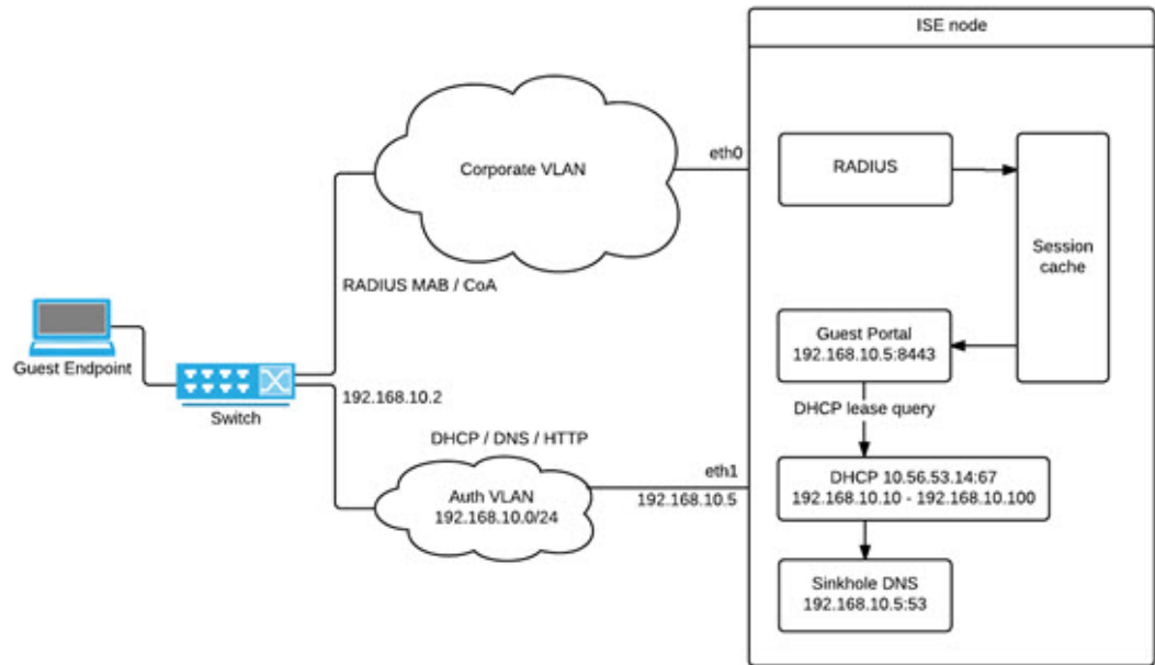
Figure 17: Auth VLAN Connected to Cisco ISE Node
