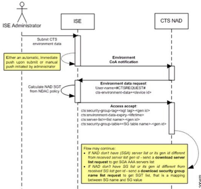
Figure 65: Environment CoA Notification Flow
