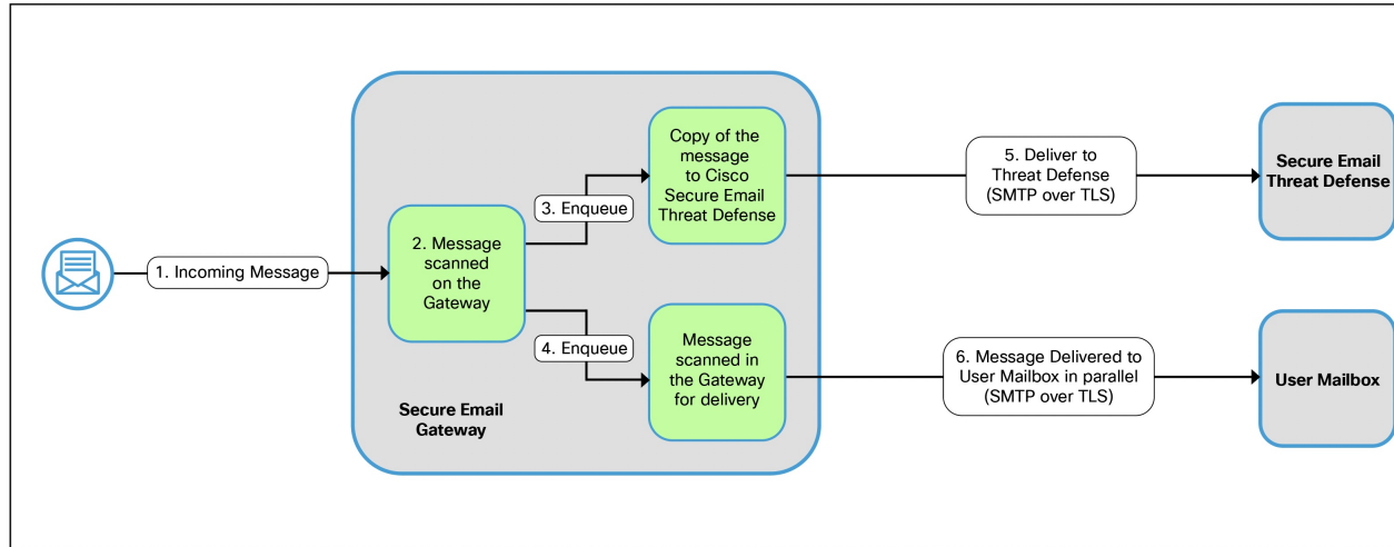
Figure 18: Overview of Threat Defense Connector
