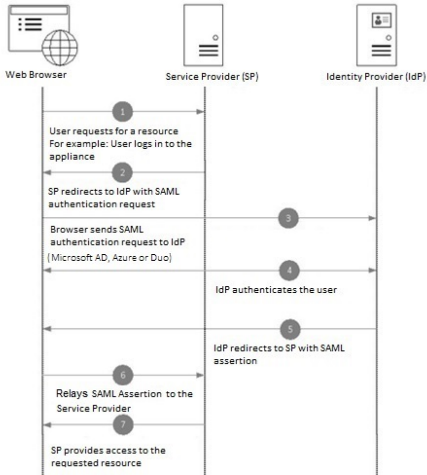
Figure 76: SAML Workflow
