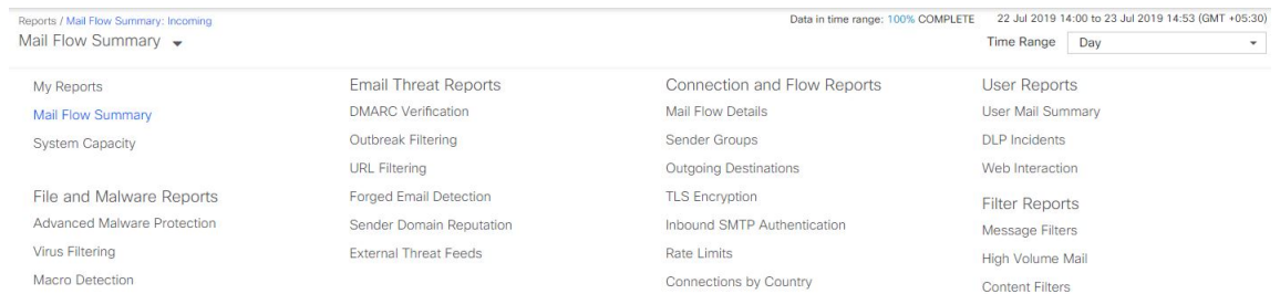
Figure 70: Reports Drop-down
