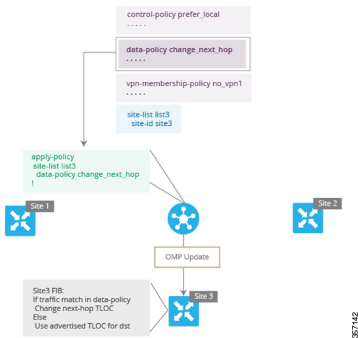
Figure 9: Data Policy Topology
