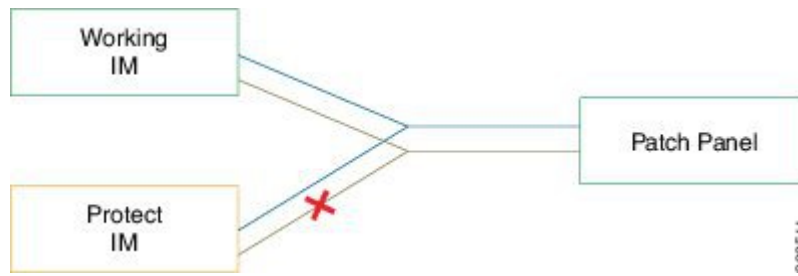
Figure 1: Y Cable
