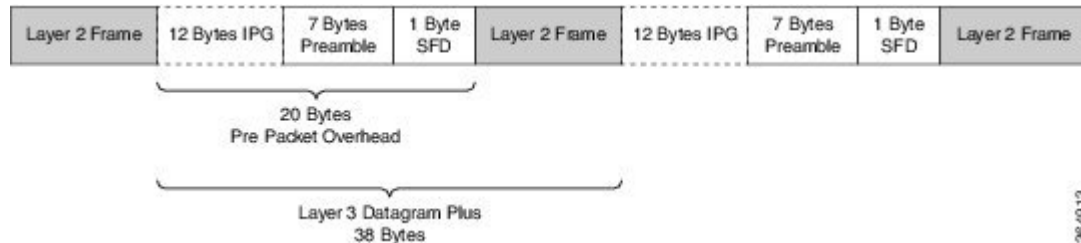
Figure 5: Ethernet Overhead
