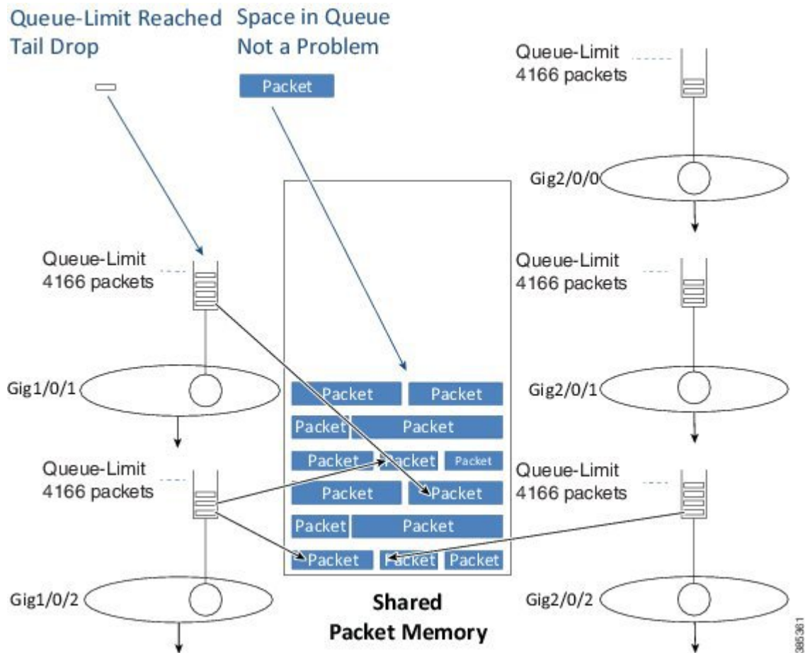
Figure 72: Tail Drop
