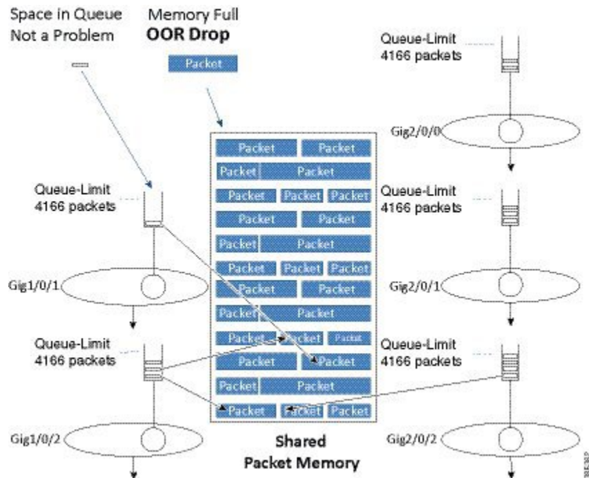
Figure 73: OOR Drop
