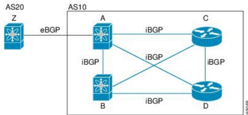
Figure 10: iBGP Network
