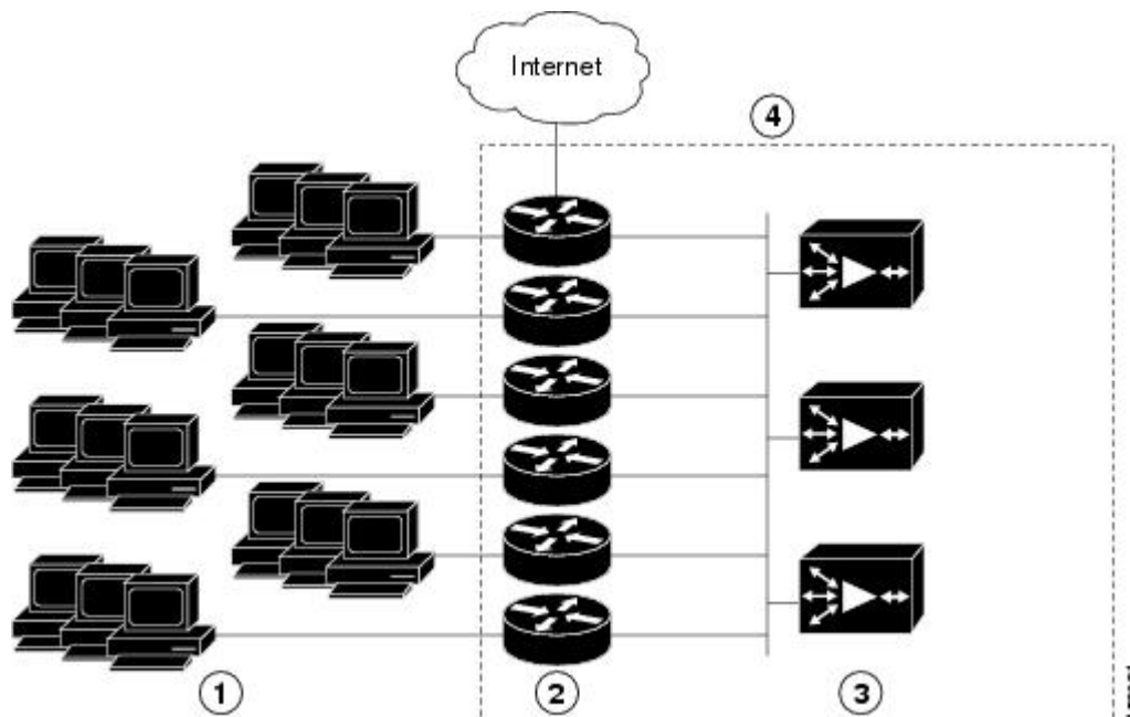
Figure 31: Service Groups with WCCP Version 2
