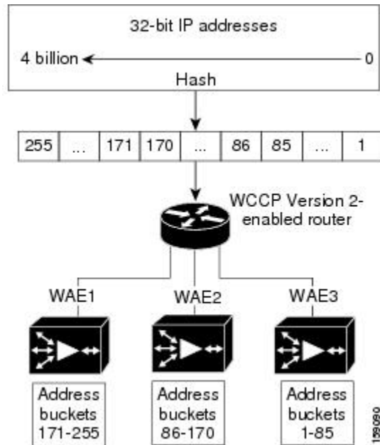
Figure 32: Load Balancing Through Hashing of IP Addresses
