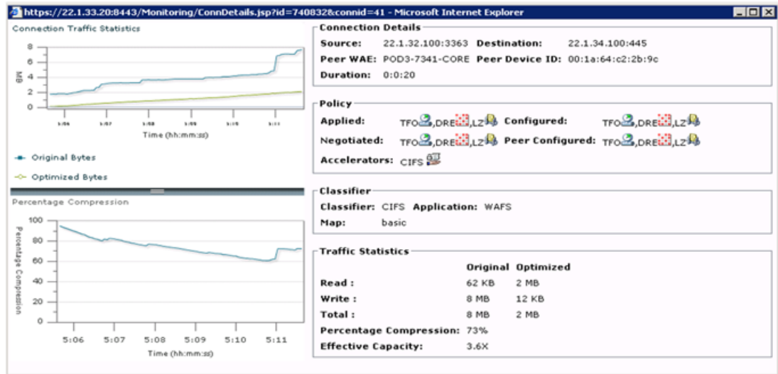
Figure 1-14 WAAS Central Manager: Flow Details Pop-Up Window
