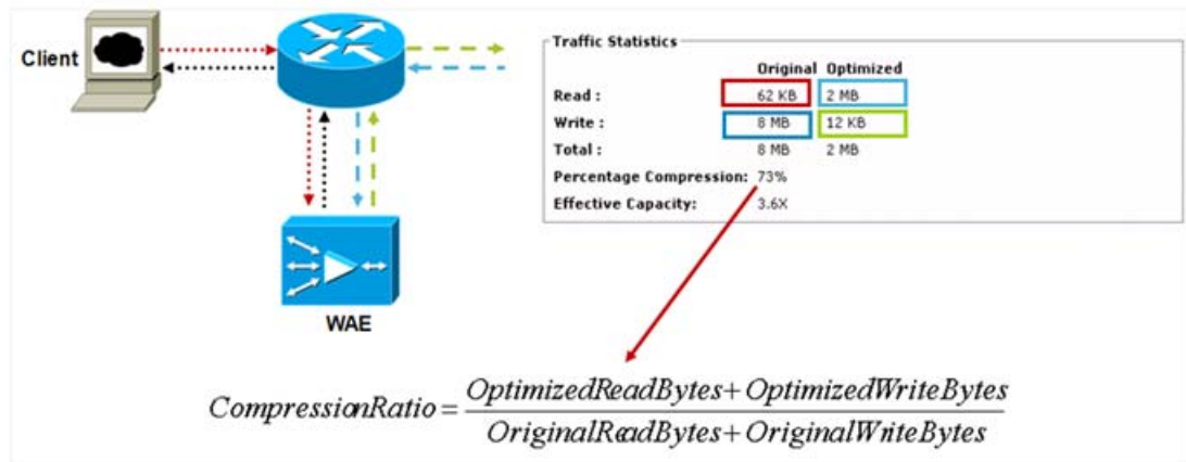
Figure 1-15 Interpreting Traffic Statistics
