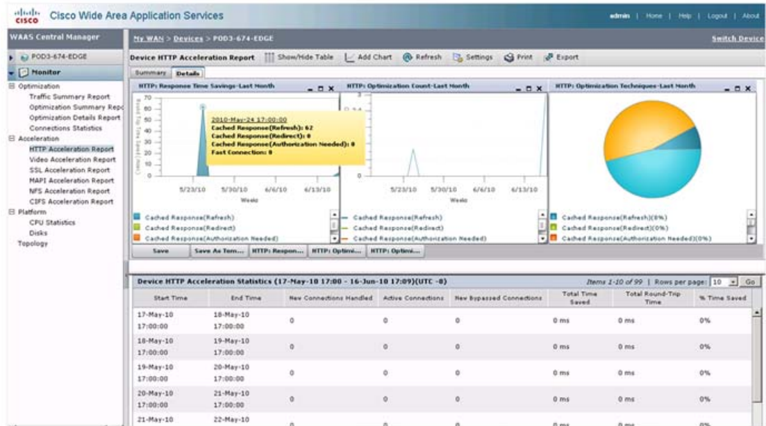
Figure 1-16 WAAS Central Manager: Device HTTP Acceleration Report
