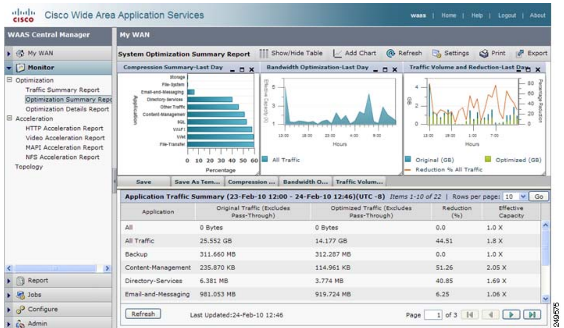
Figure 1-12 WAAS Central Manager: Device Optimization Summary Report
