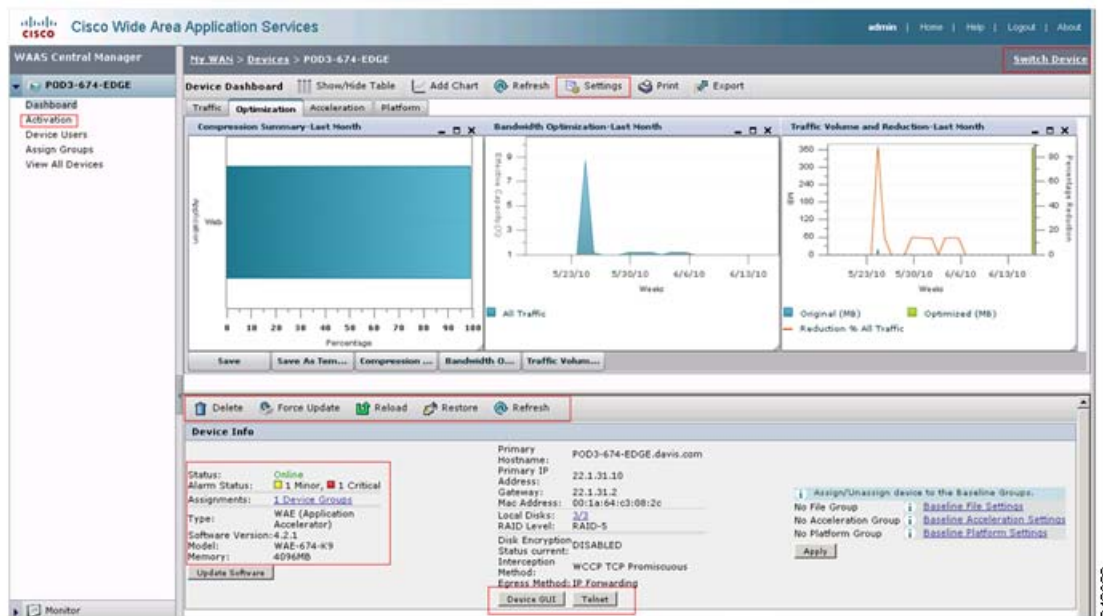
Figure 1-11 WAAS Central Manager: Device Dashboard
