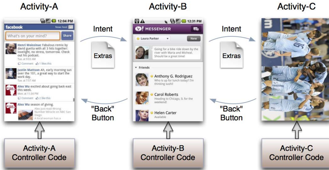
Figure 2-2 Android Activity Overview
