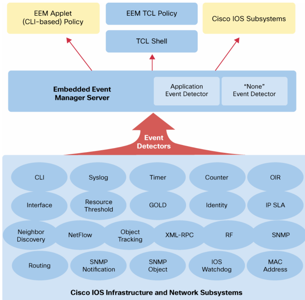
Figure 1. EEM Architecture
