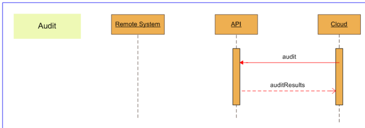
Figure 5.37 Sequence Diagram for Resource Management Audit API
