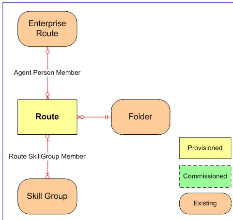
Figure 5.23 Route Relationships
