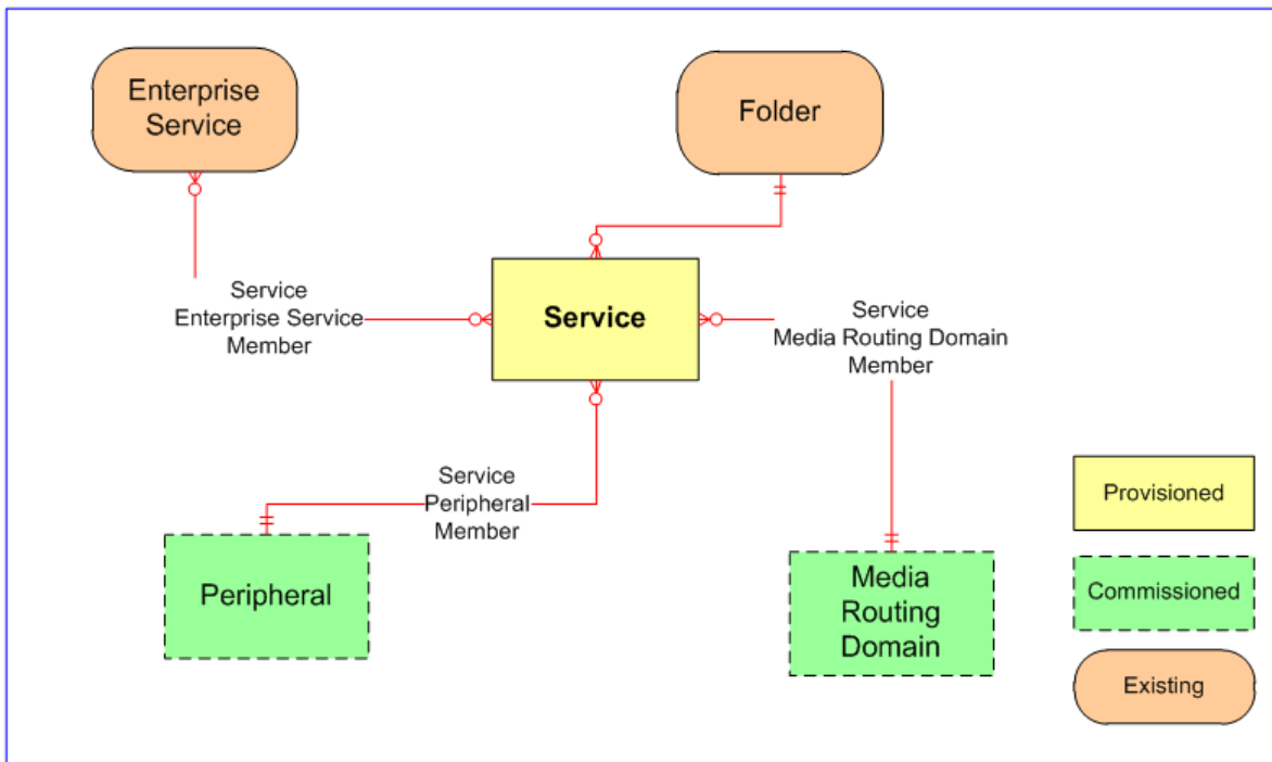
Figure 5.25 Service Relationships
