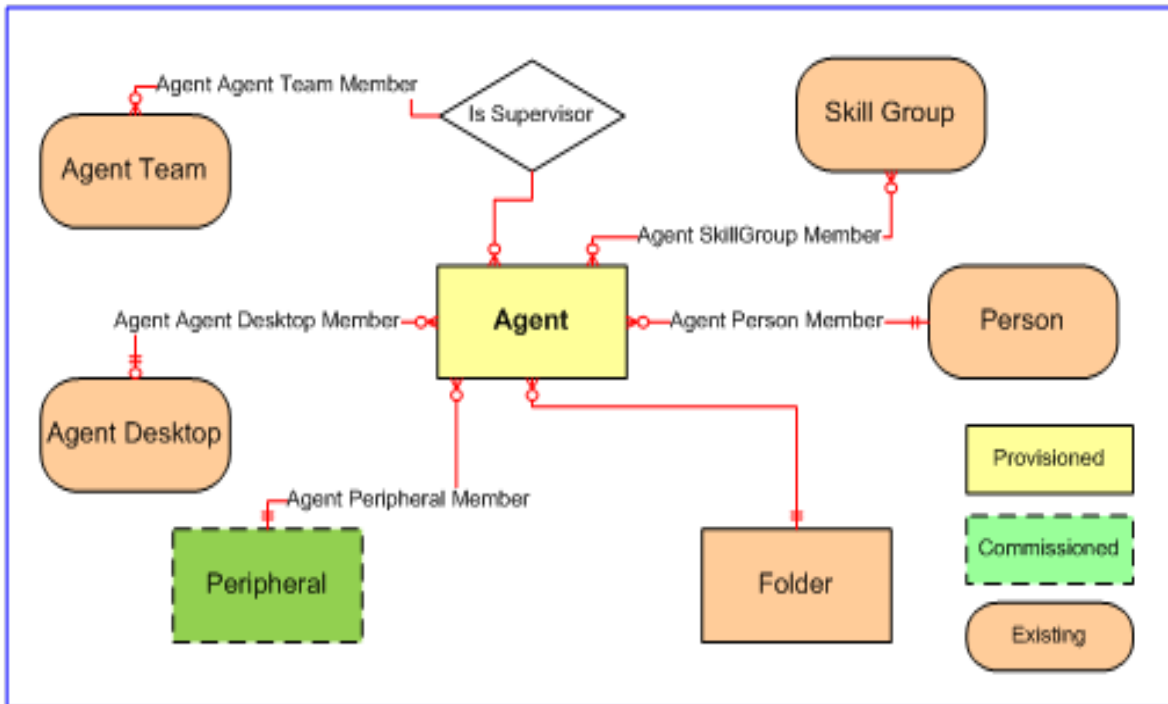
Figure 5.7 Agent Relationships
