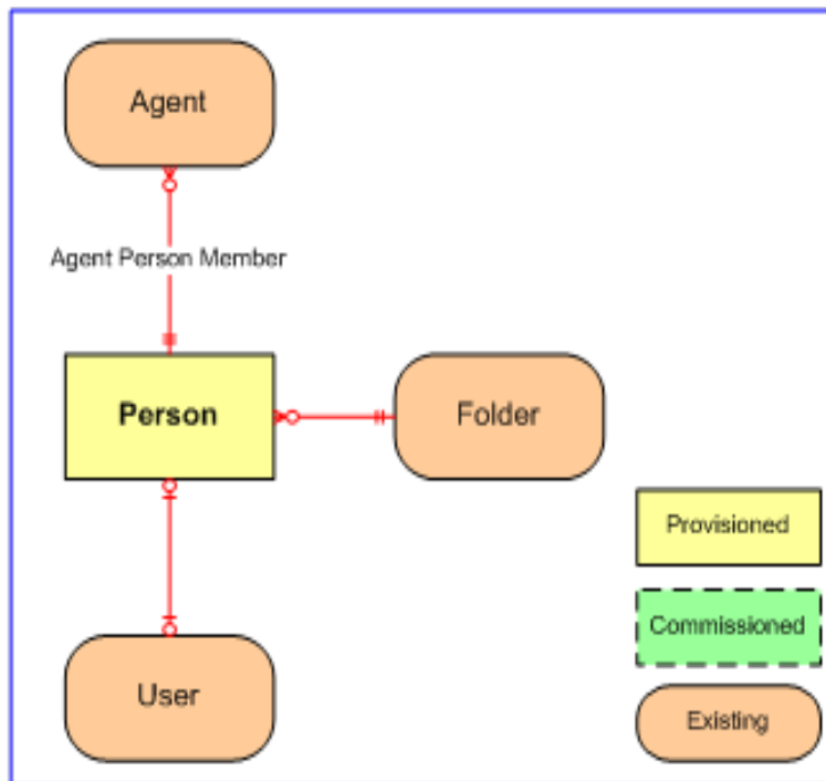
Figure 5.20 Person Relationships
