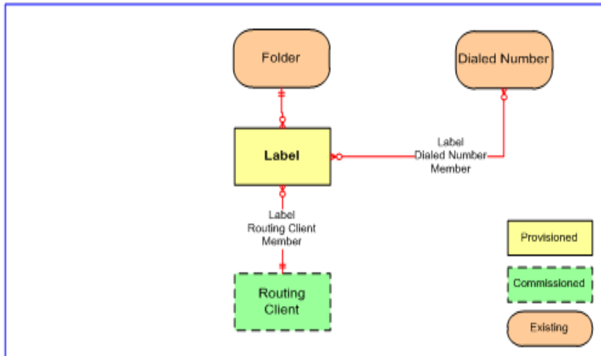
Figure 5.17 Label Relationships
