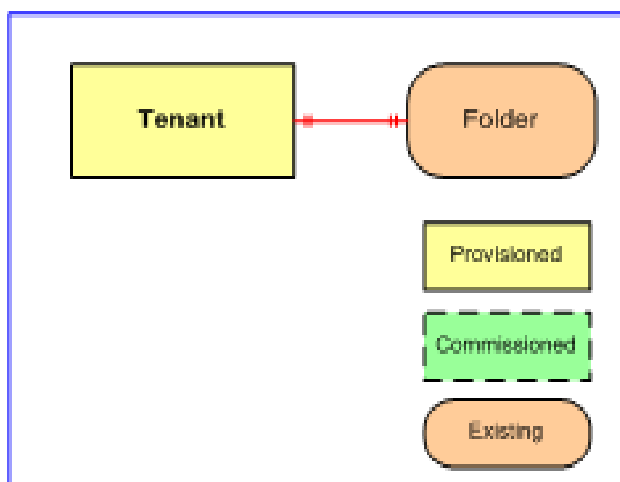
Figure 5.27 Tenant Relationships
