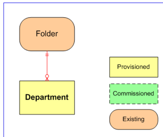
Figure 5.12 Department Relationships
