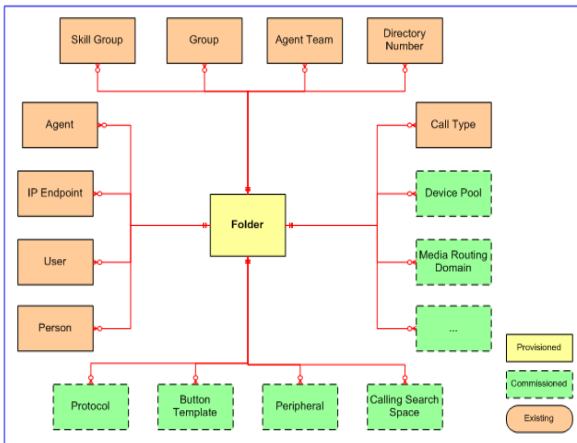
Figure 5.4 Folder Relationships
