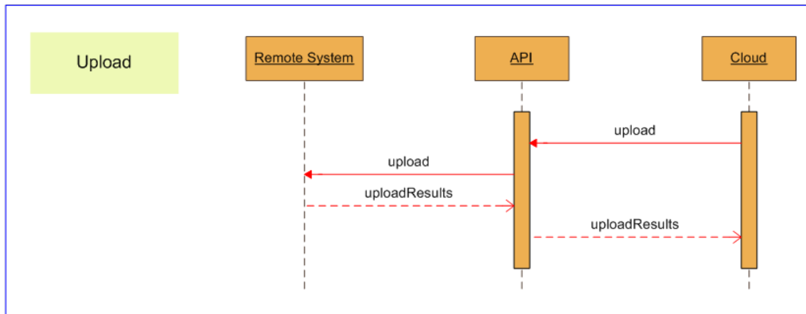
Figure 5.38 Sequence Diagram for Resource Management Upload API
