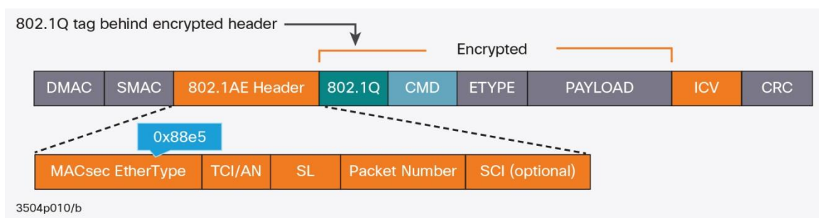
Figure 10. WAN MACsec – 802.1Q Tag Encrypted
