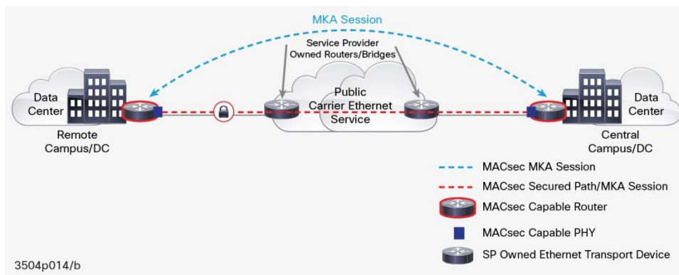
Figure 13. WAN MACsec Site-to-Site Example and Components
