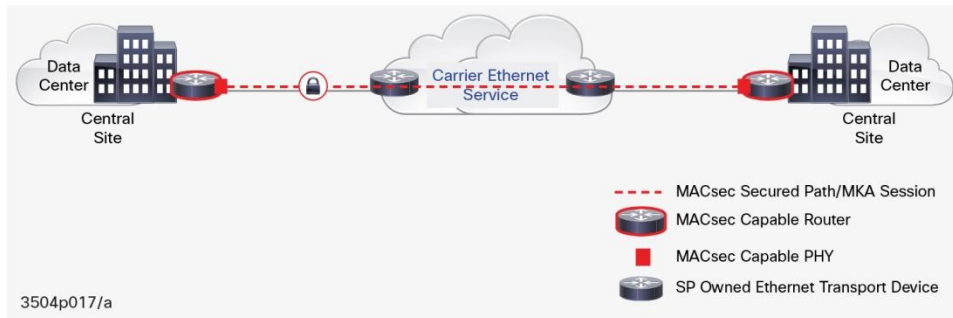
Figure 17. WAN MACsec Point to Point E-LINE Example
