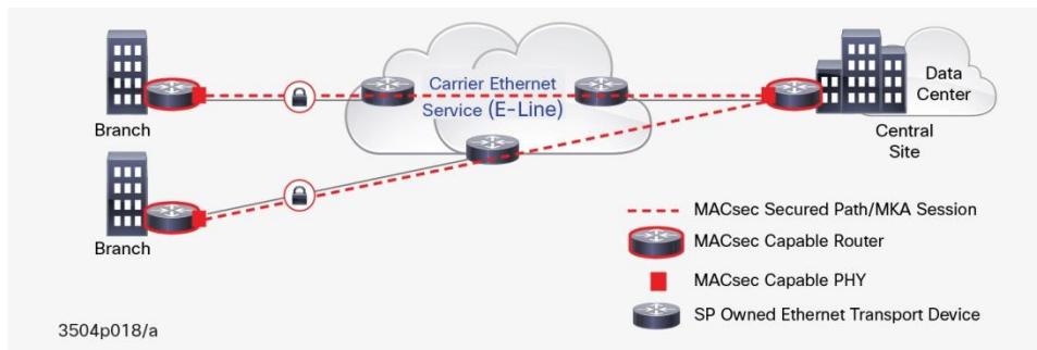
Figure 18. WAN MACsec Point to Multipoint E-LINE Example
