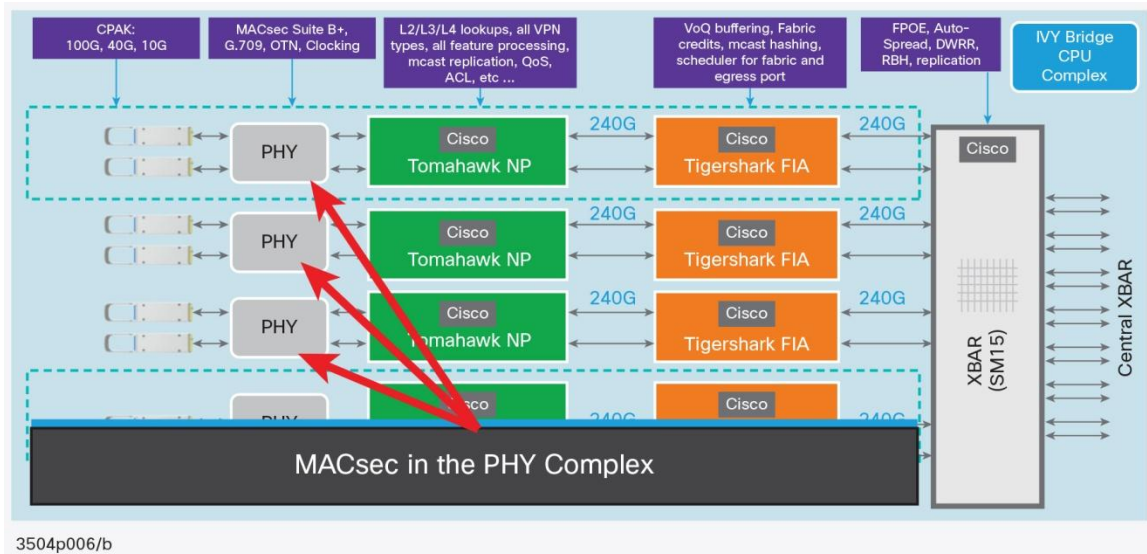
Figure 6. MACsec in the PHY – ASR 9000 “Tomahawk” Line Card Example
