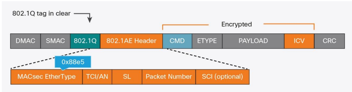
Figure 11. WAN MACsec – 802.1Q Tag in the Clear Example
