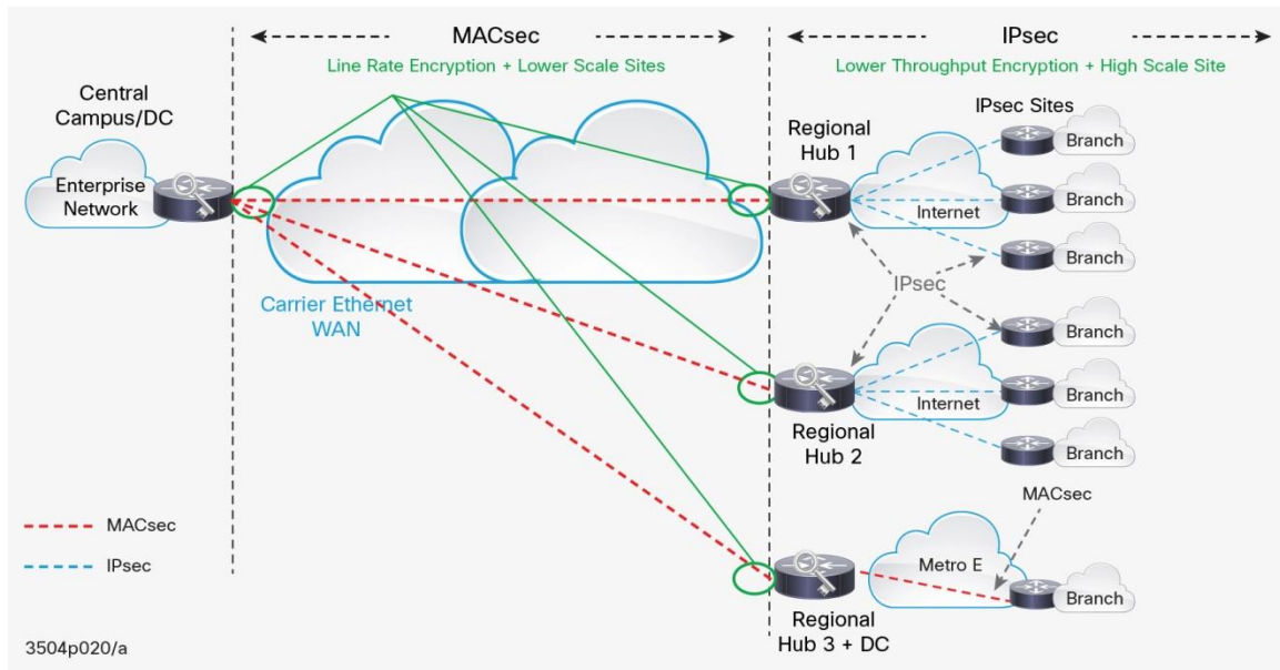
Figure 20. Typical Two-Tier WAN Design
