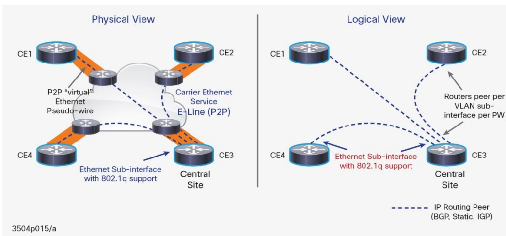
Figure 15. Router Peering Model over MEF E-LINE Service
