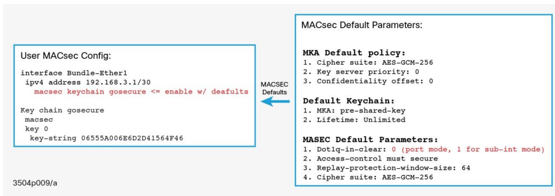
Figure 9. MACsec Policies
