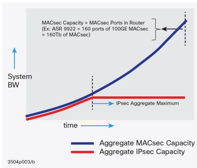
Figure 3. Aggregate MACsec vs. IPsec Encryption System Capacity
