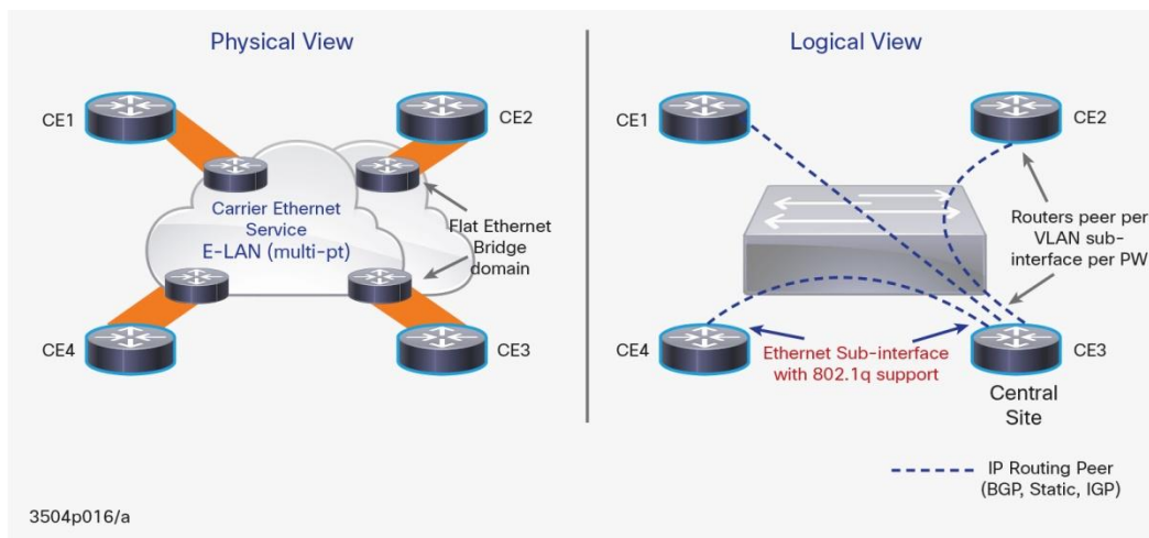
Figure 16. Router Peering Model over MEF E-LAN Service
