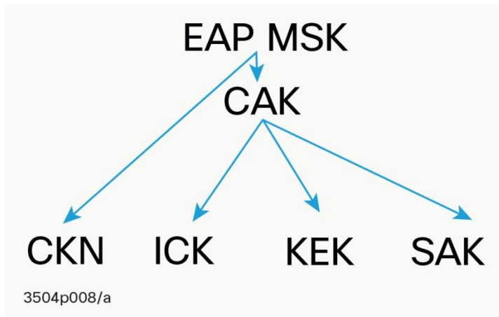
Figure 8. 802.1X/EAP Key Derivation
