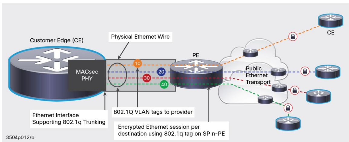
Figure 12. MACsec Tag in the Clear for a Hub/Spoke Design
