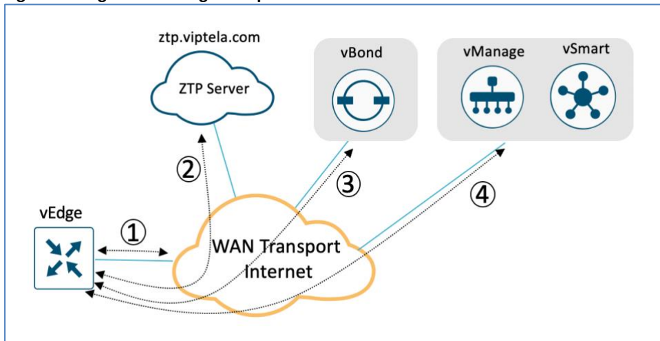
Figure 7 vEdge onboarding – ZTP process
