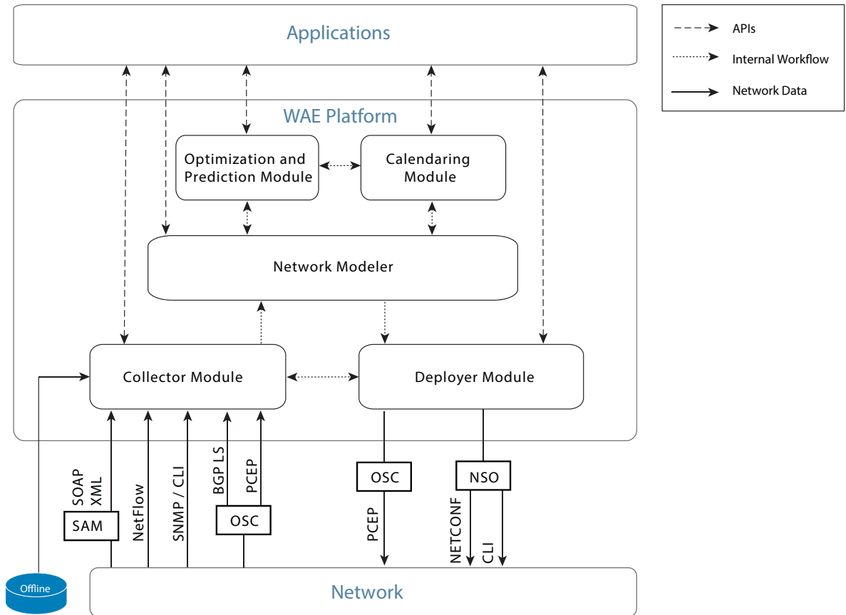
Figure 1-1 WAE Platform Workflow
