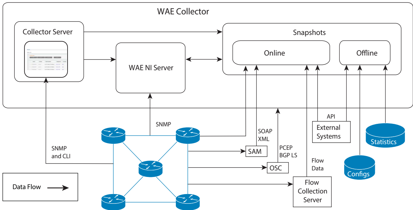
Figure 4-1 WAE Collector Workflow
