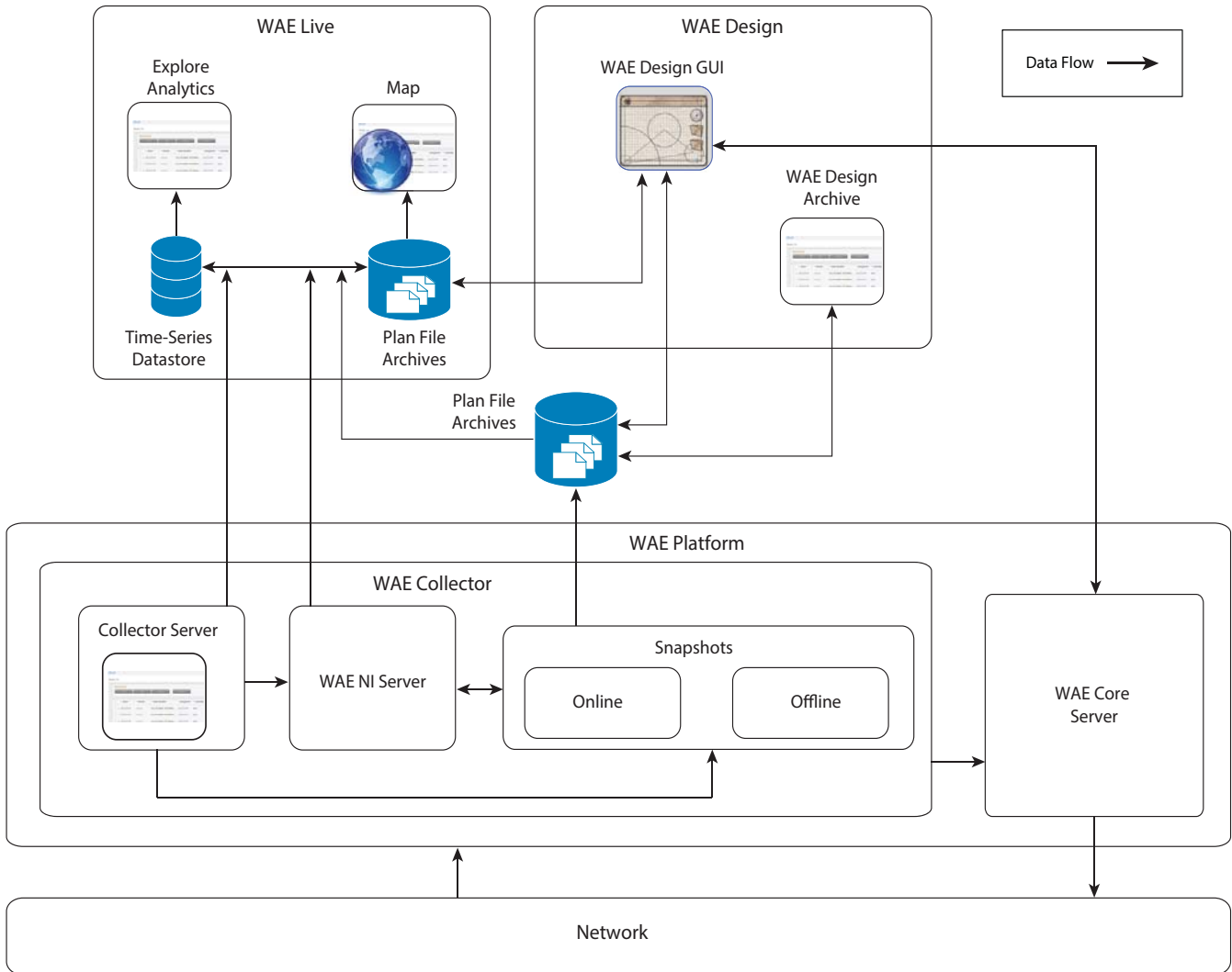
Figure 4-2 Data Flow after Collection
