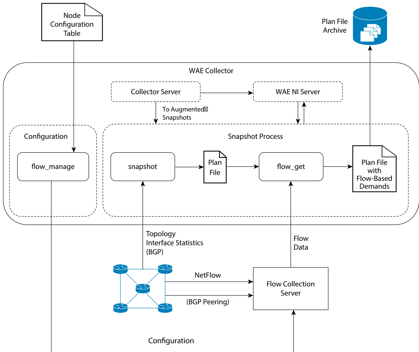
Figure 22-1 Flow Collection Workflow
