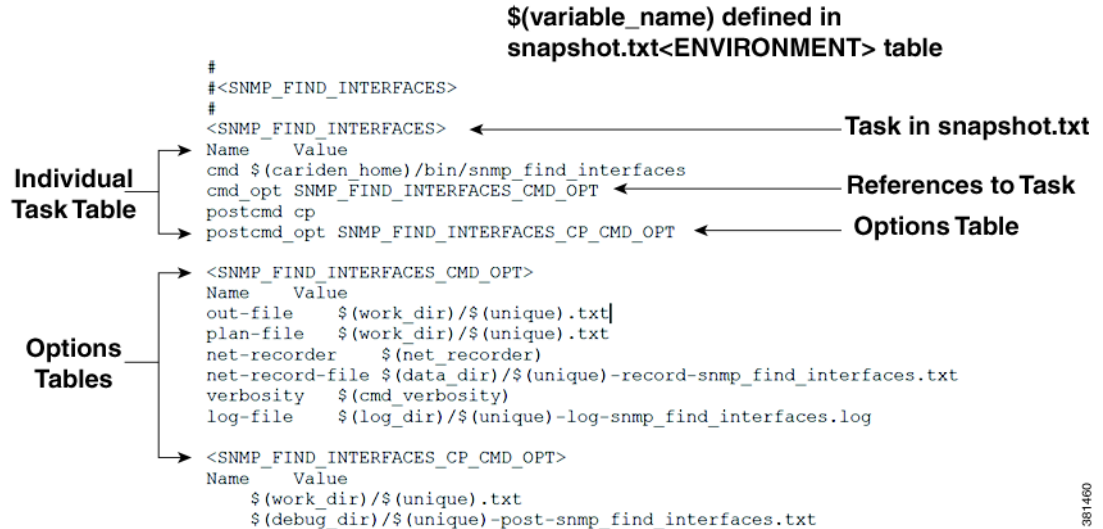
Figure 17-1 Example Task Defined in snapshot.inc
