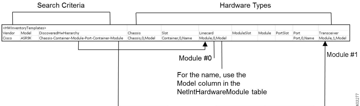
Figure 23-1 Example HWInventoryTemplates Entry
