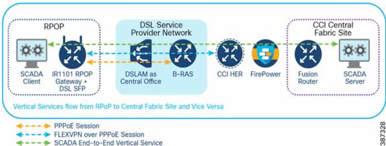
Figure 29 CCI RPoP connectivity to CCI Headend via DSL backhaul
