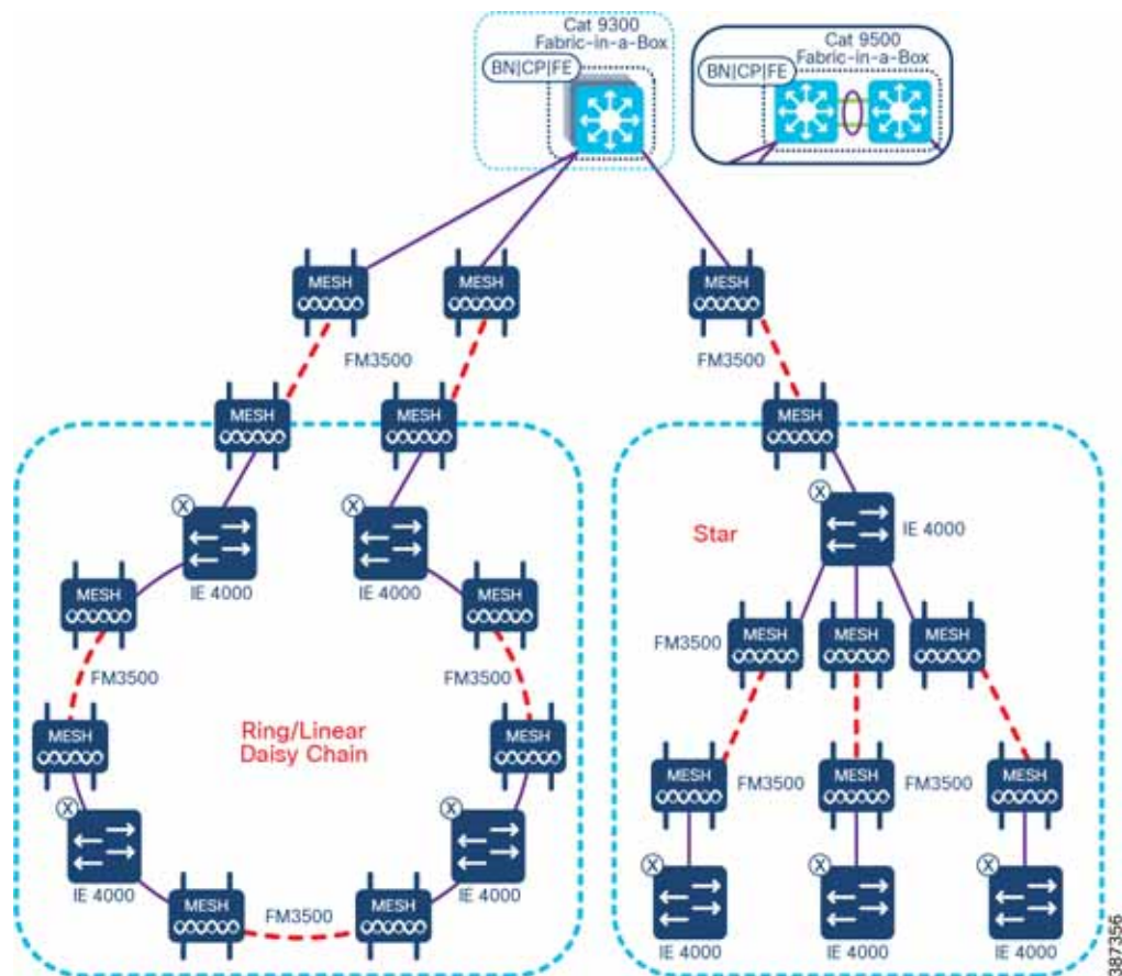
Figure 39 CURWB Access
