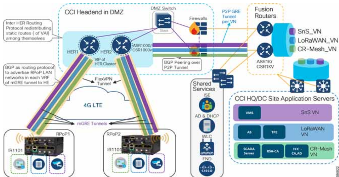
Figure 24 RPoP Gateway with Macro-Segmentation Design
