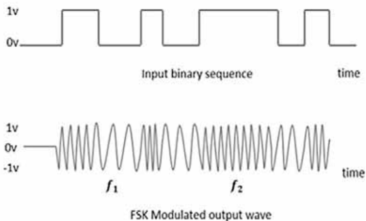
Figure 47 FSK Modulation Wave
