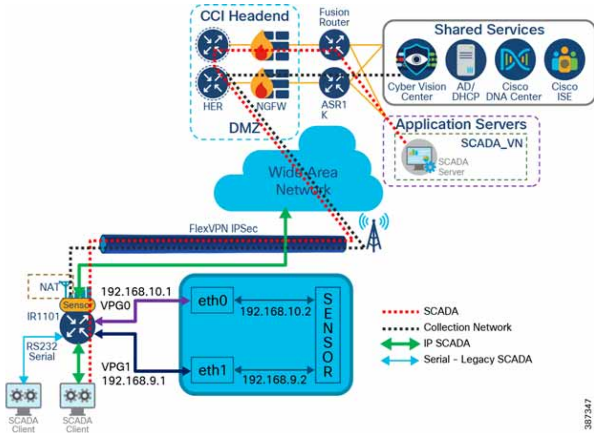
Figure 70 RPoP IR1101 Gateway as Cyber Vision Sensor
