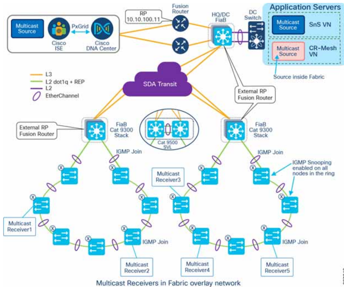
Figure 81 Multicast over SD-Access Transit Network
