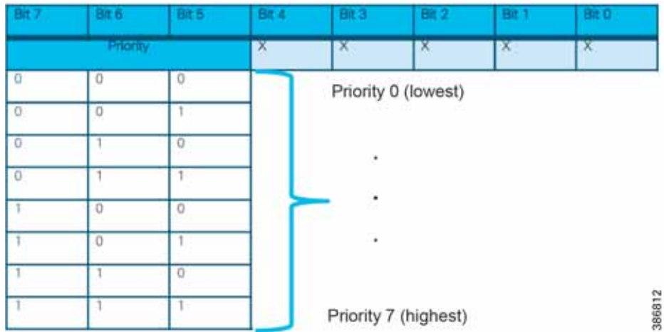
Figure 36 Priority Value in DSCP/TOS Field
