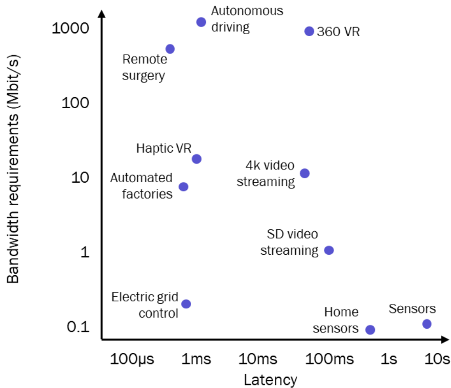
Figure 2: Network latency and bandwidth requirements for a range of use cases
