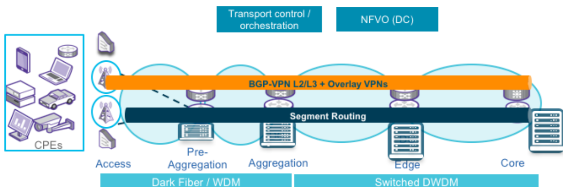
Figure 7: Transport slicing architecture
