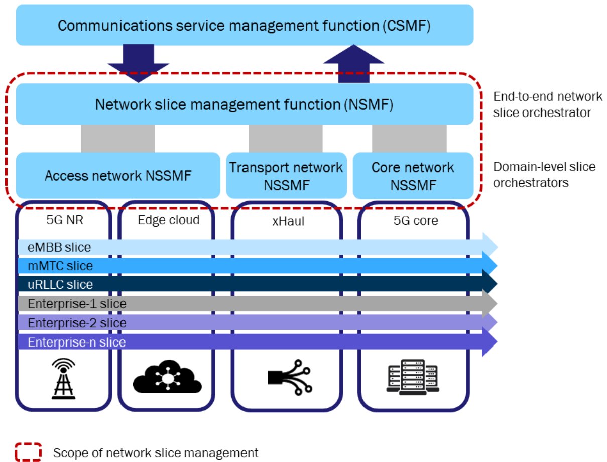
Figure 5: 3GPP reference architecture for network slicing
