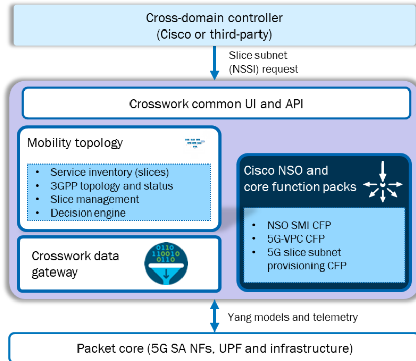
Figure 13: Cisco's Crosswork Core Controller, with associated use cases
