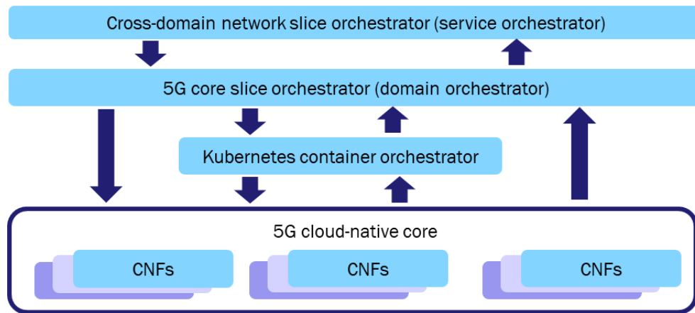
Figure 10: 5G core and slice orchestration
